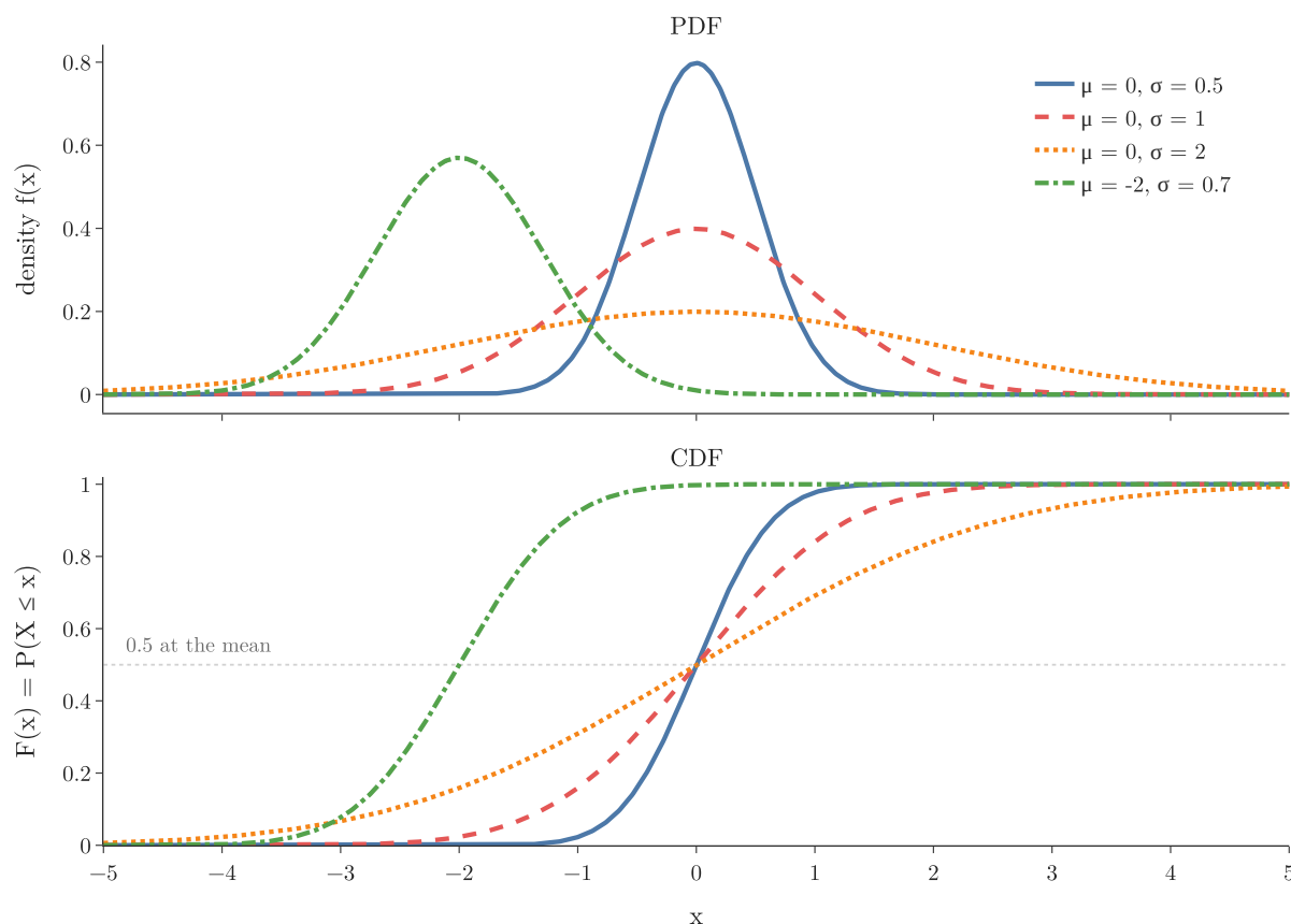
Figure 7: Normal PDFs (top) and their CDFs (bottom)
