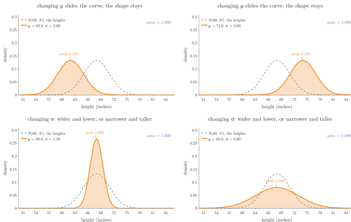
Figure 2: The heights curve N(68, 3^2) with its mean moved from 62 to 74, then its standard deviation changed from 1.5 to 5; the peak height and the area are printed in every frame
