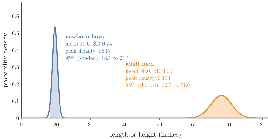
Figure 3: Newborn boys’ length, N(19.6, 0.75^2) , and adult men’s height, N(68, 3^2) : the narrow curve is four times as tall; the shaded parts hold 95% of each group
