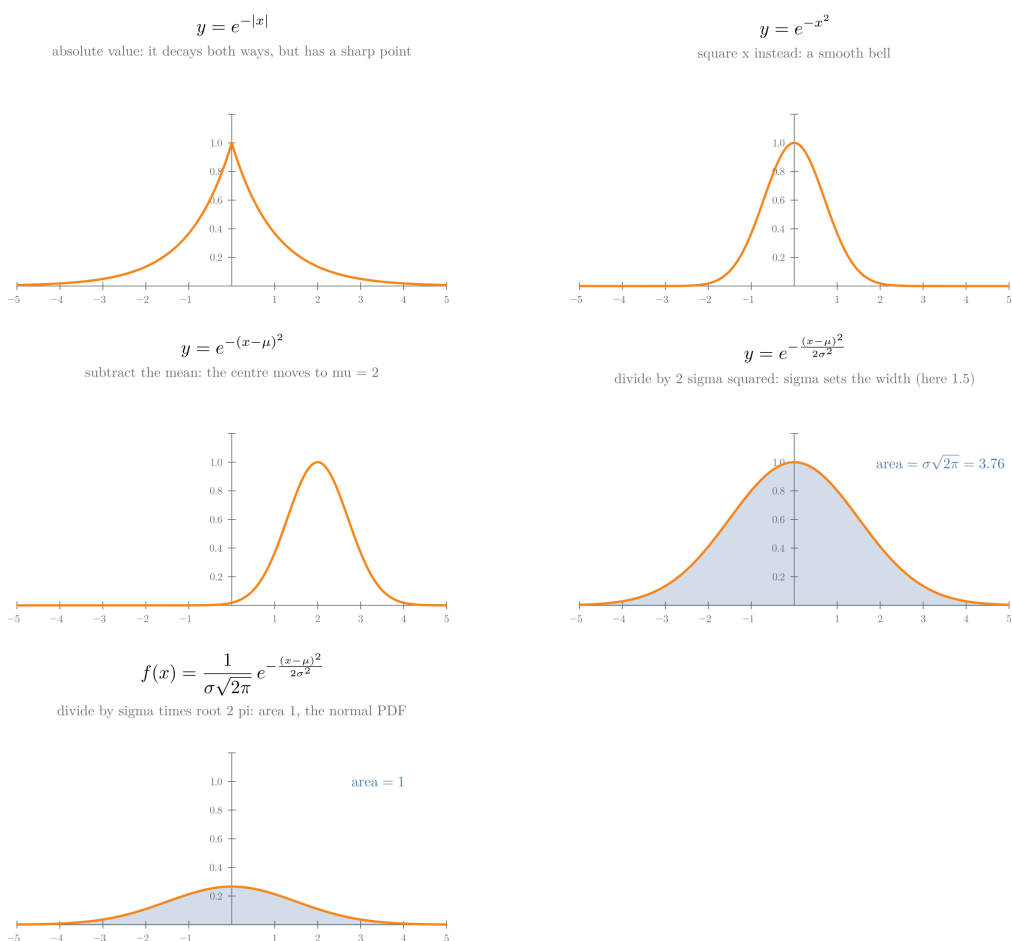
Figure 4: Building the normal PDF term by term: the bell, the shift, the width, the area
