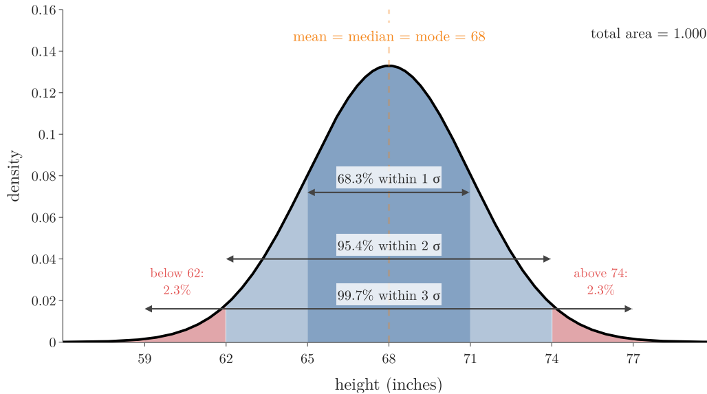
Figure 6: Properties of N(68, 3^2) : one centre for mean, median and mode, 68.3%, 95.4% and 99.7% within 1, 2 and 3 standard deviations, equal tails, total area 1
