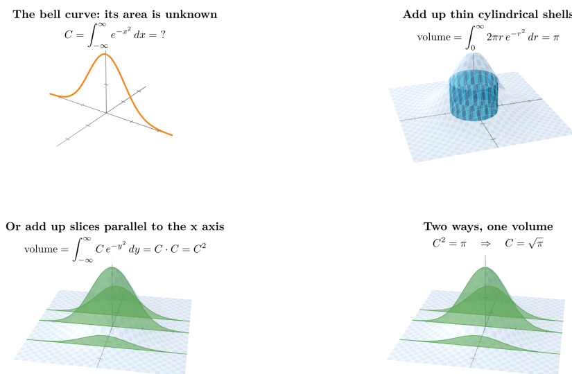
Figure 5: The bell lifted to a round bell-shaped surface: its volume by thin cylindrical shells is pi, by slices it is C^2 , so C = \text{square root of pi} (idea after 3Blue1Brown, “Why \pi is in the normal distribution (beyond integral tricks)”) )
