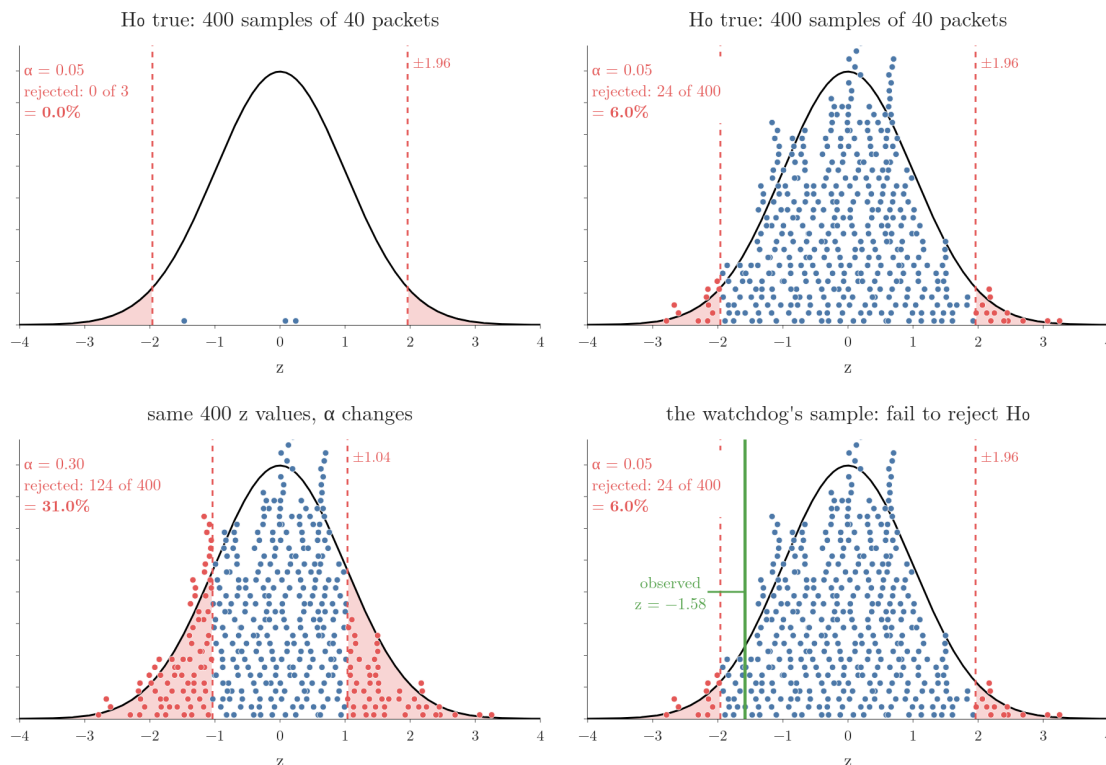
Figure 8: 400 z values from samples where H_0 is true drop onto the standard normal curve; red dots fall in the rejection region, and their share tracks \alpha as \alpha changes
