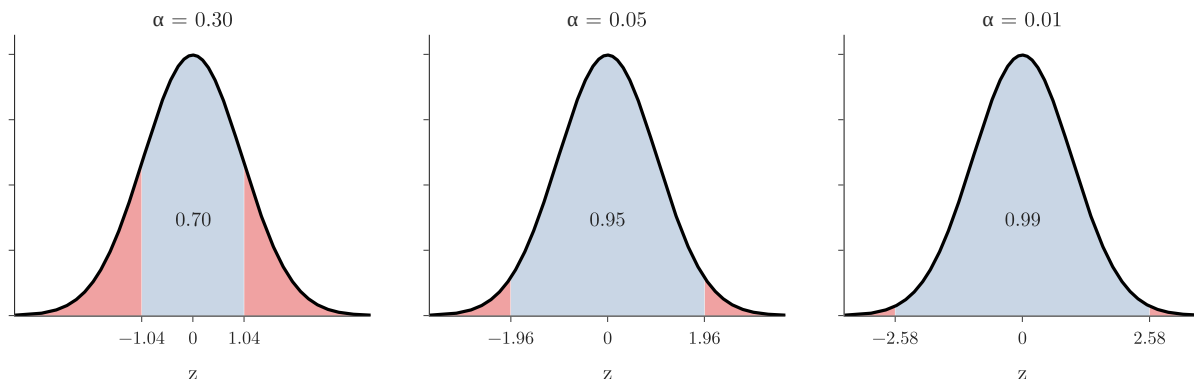
Figure 7: Two-tailed rejection regions (red) for three significance levels; the middle area is 1 - \alpha
