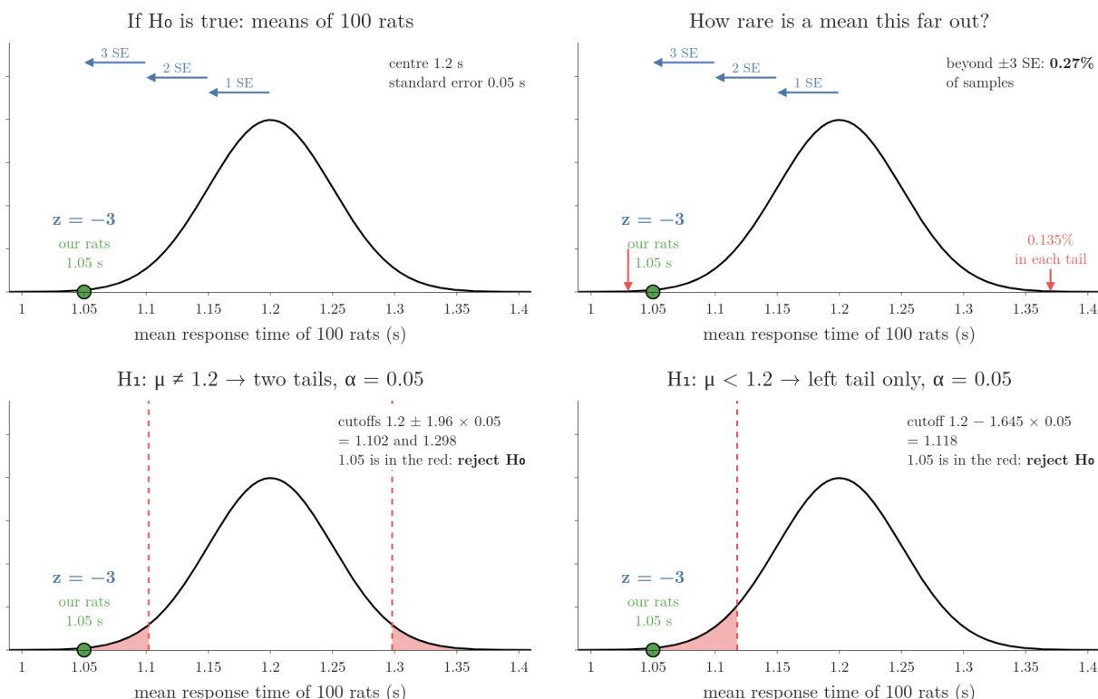
Figure 2: The rat drug test step by step: the sampling distribution of the mean if H_0 is true (centre 1.2 s, standard error 0.05 s); 1.05 s sits 3 standard errors below; only 0.27% of samples land that far out; then the two-tailed and the one-tailed rejection regions at \alpha = 0.05 . Idea after Khan Academy, “Hypothesis testing and p-values”
