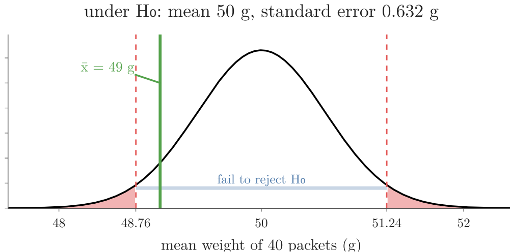
Figure 6: The chips test in grams: sample means between 48.76 g and 51.24 g fail to reject H_0 ; the watchdog's 49 g lies inside
