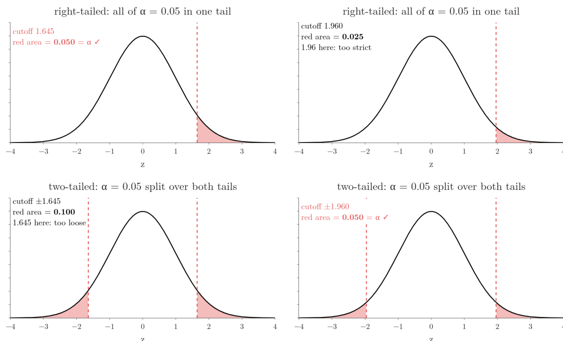
Figure 5: Finding the critical value: a cutoff slides until the red tail area equals \alpha = 0.05 , at 1.645 for one tail and \pm 1.96 for two
