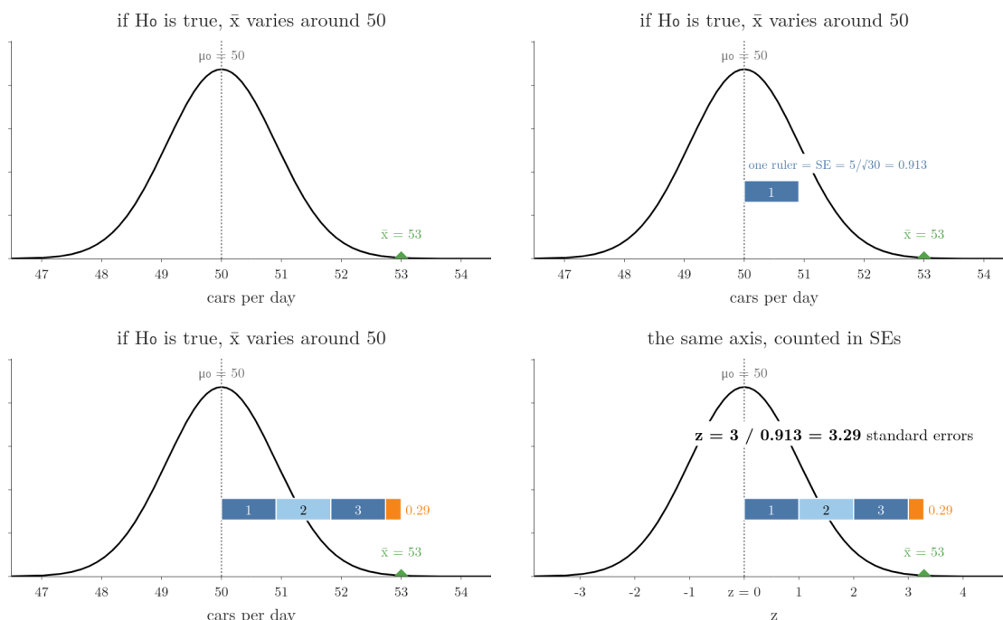
Figure 3: Counting standard errors: rulers of 0.913 laid from 50 towards 53 fit 3.29 times, so z = 3.29
