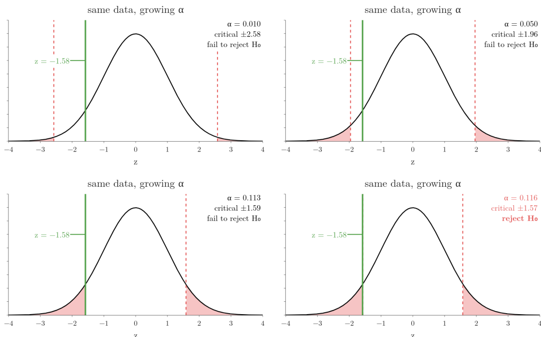
Figure 4: The chips z = -1.58 stays put while \alpha grows; once \alpha passes 0.114 the red tails reach it and the same data “rejects” H_0
