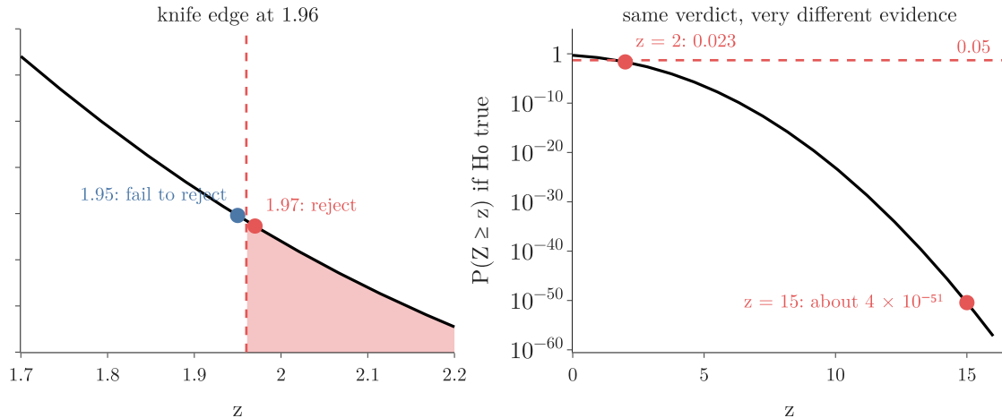
Figure 9: Left: z = 1.95 and 1.97 straddle 1.96 and get opposite verdicts. Right: P(Z \geq z) on a log scale; z = 2 and z = 15 are both below 0.05 , about 49 powers of ten apart
