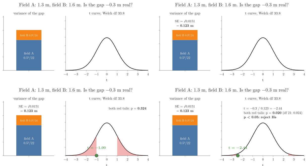
Figure 2: The tomato fields: the gap’s variance is built from one part per field, its square root is the standard error 0.123 m, and t = -0.3/0.123 = -2.44 leaves p = 0.020 in the two red tails. Idea after Khan Academy, “Two-sample t test for difference of means”
