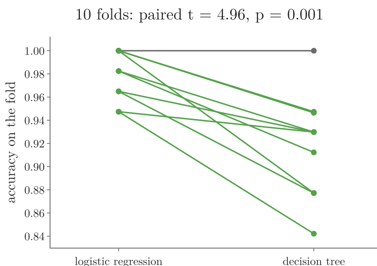
Figure 7: Logistic regression against a decision tree on the same 10 folds of scikit-learn’s breast cancer data: one line per fold, paired t = 4.96, p = 0.001
