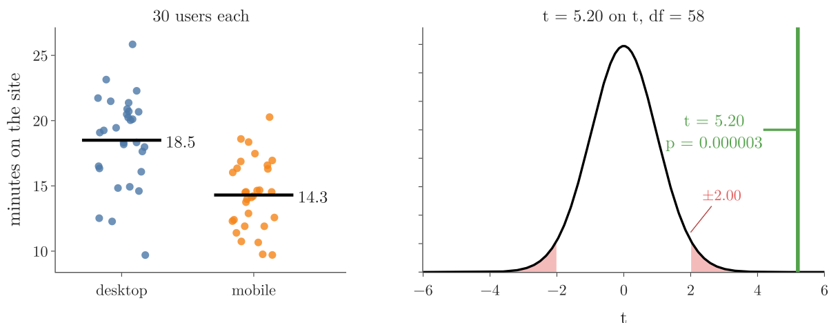
Figure 3: The 60 users (left) and t = 5.20 on the t -distribution with 58 degrees of freedom (right), far past the cutoffs \pm 2.00
