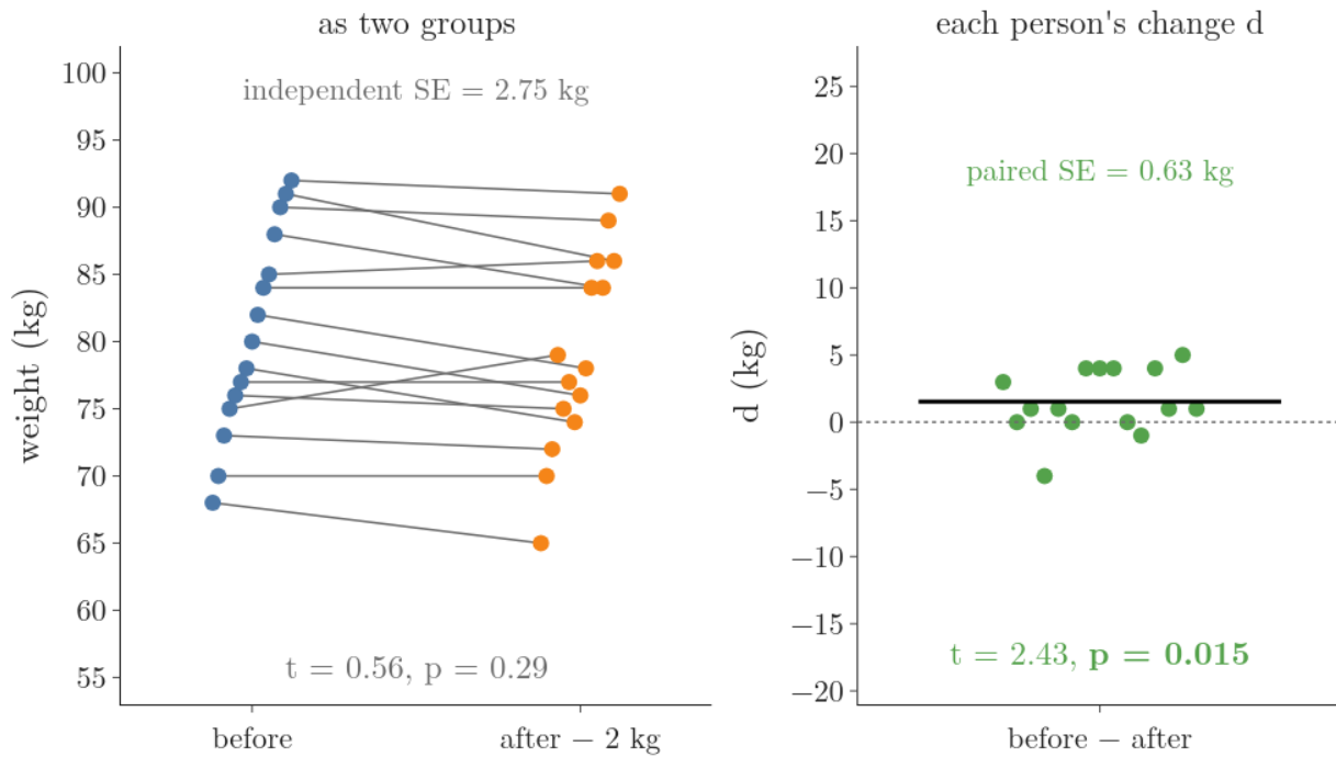
Figure 6: The 2 kg-lower table as two groups (left, independent SE 2.75 kg) and as 15 personal changes d (right, paired SE 0.63 kg), both panels on the same 49 kg scale
