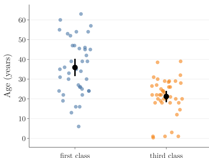
Figure 4: Our samples of 40 first-class and 40 third-class ages, with each sample mean and its 95% confidence interval
