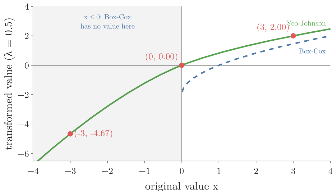
Figure 4: Yeo-Johnson (green) and Box-Cox (blue dashed) with \lambda = 0.5 : only Yeo-Johnson covers zero and negative values
