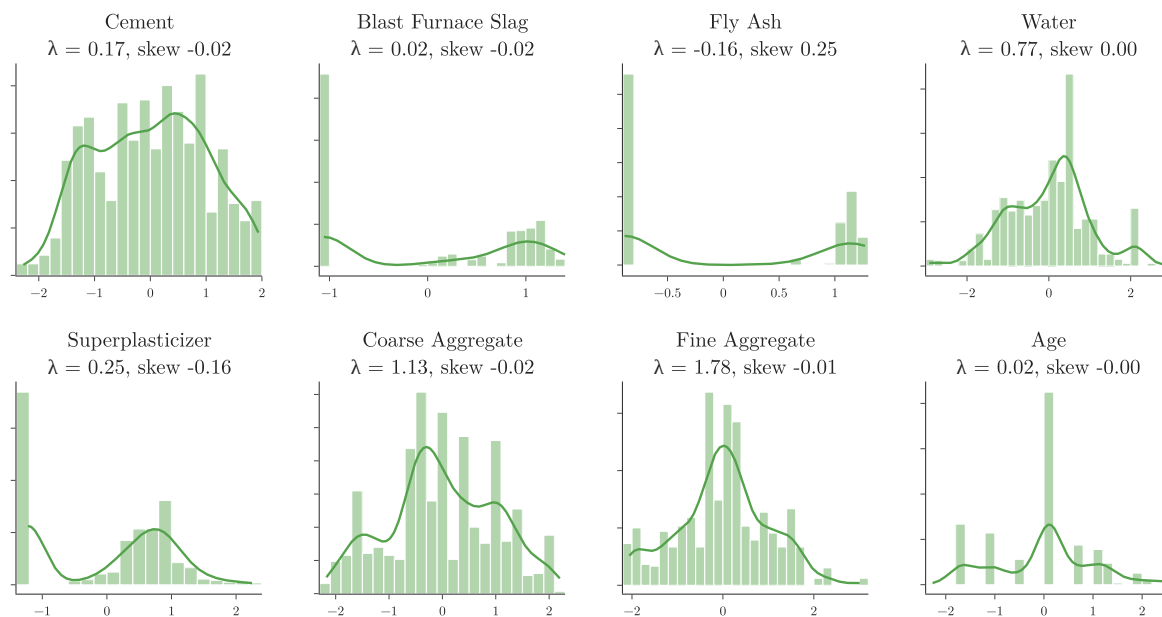
Figure 8: All 8 training columns after Yeo-Johnson, with each learned lambda and skewness
