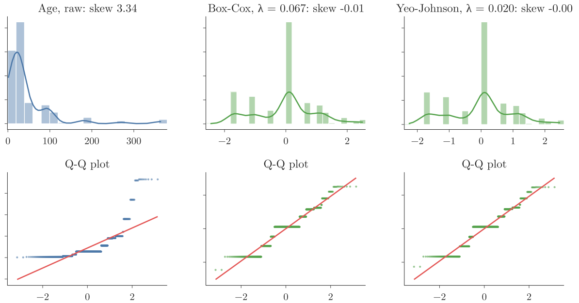
Figure 6: Age before (blue) and after Box-Cox and Yeo-Johnson (green): histogram and Q-Q plot
