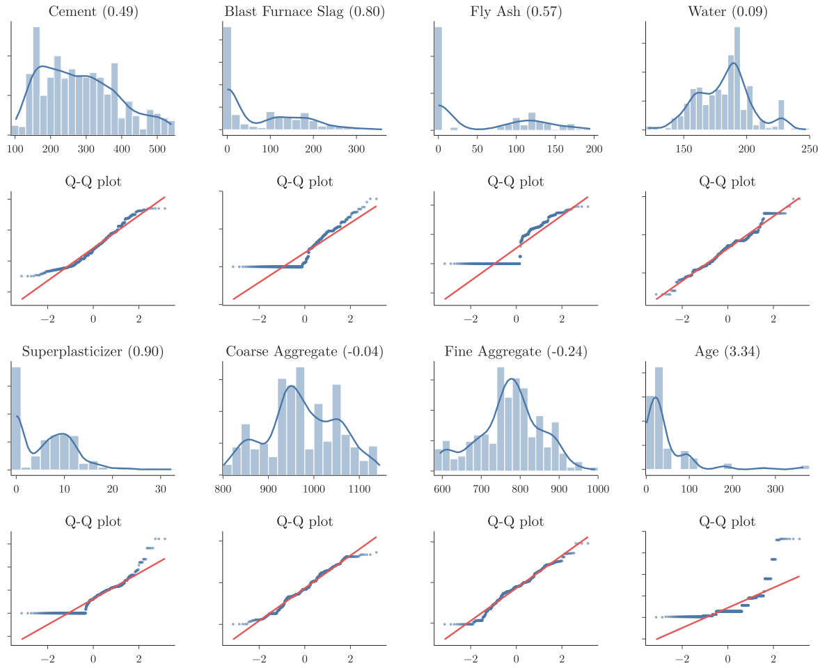
Figure 5: The 8 raw input columns of the training set: histogram (skewness in brackets) and Q-Q plot
