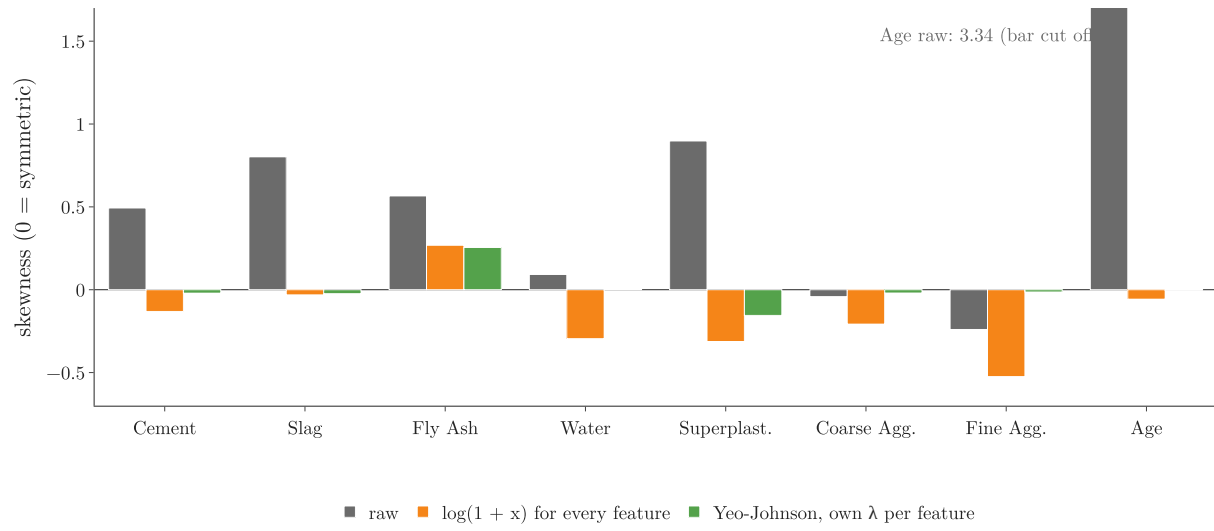
Figure 9: Skewness of each concrete feature: raw, after \log(1 + x) on every feature, and after Yeo-Johnson with its own lambda per feature
