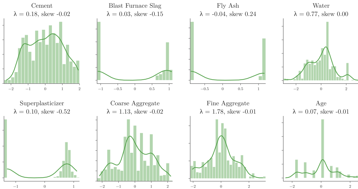
Figure 7: All 8 training columns after Box-Cox, with each learned lambda and skewness
