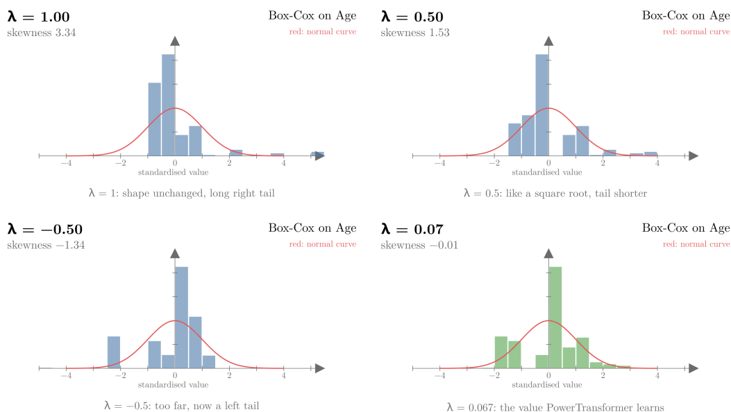
Figure 3: Box-Cox on Age as lambda moves: 1 (unchanged), 0.5, -0.5 (overshoot), and the learned 0.067
