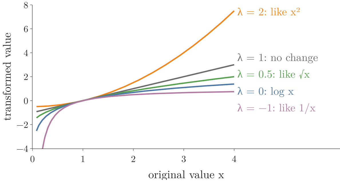
Figure 2: The Box-Cox formula for five values of lambda: each one is a transform from Note 30
