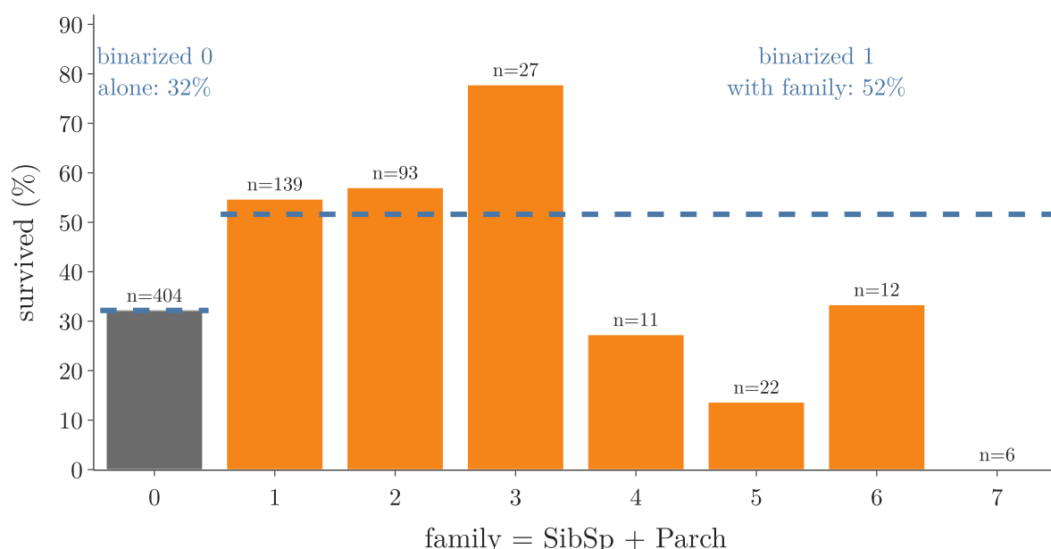
Figure 10: Survival by family size among the 714 passengers with an age; binarizing at 0 keeps the jump from alone (0) to with family (1)
