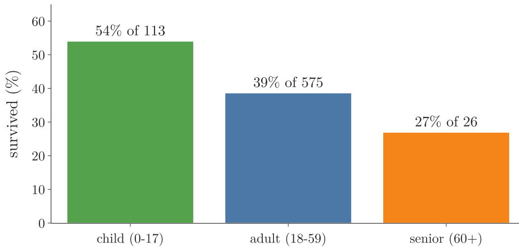
Figure 8: Survival of the three custom age groups among the 714 passengers with a recorded age
