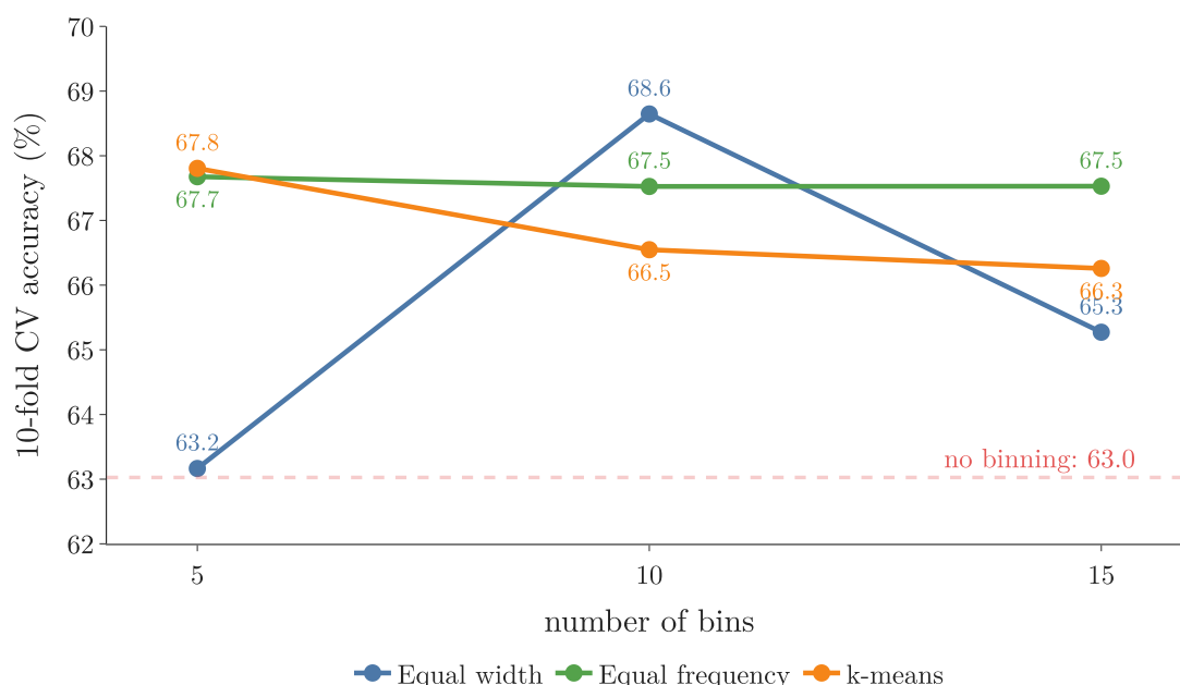
Figure 7: Cross-validated accuracy of the binned decision tree for each strategy and number of bins; the dashed line is the tree without binning
