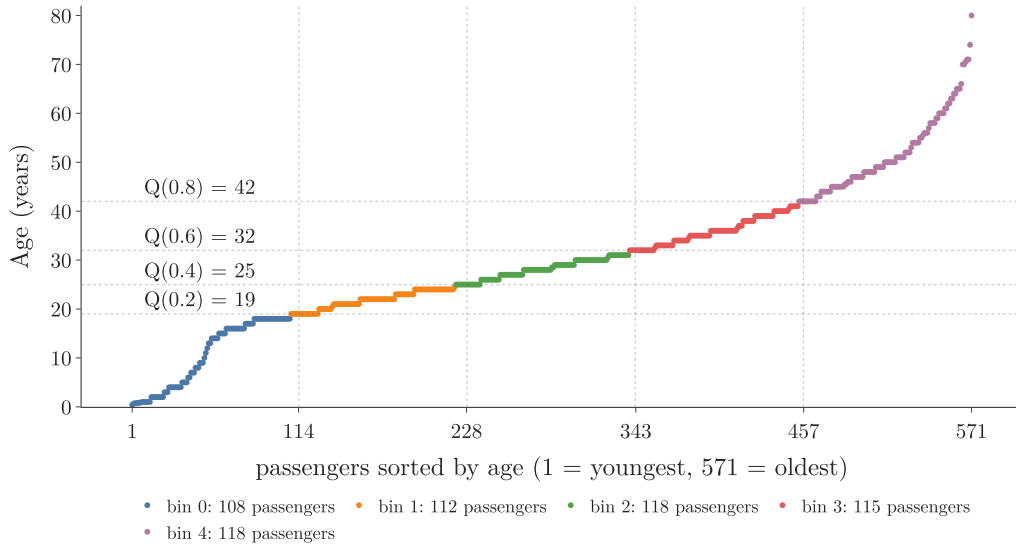
Figure 4: The 571 training ages in sorted order: cutting the list into five equal piles (vertical lines) gives the quantile edges 19, 25, 32 and 42 (horizontal lines)
