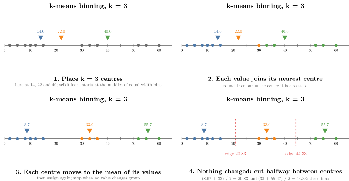
Figure 5: k-means binning on 12 values with k = 3 : place centres, assign, move, repeat, then cut halfway between centres
