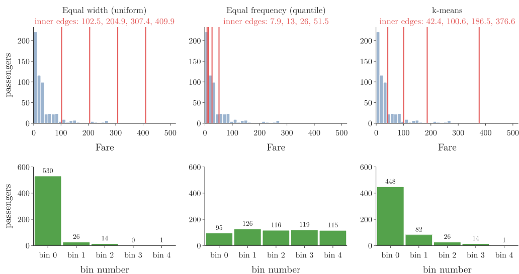
Figure 6: The three binning strategies on Fare (571 training passengers, 5 bins): bin edges (top) and passengers per bin (bottom)
