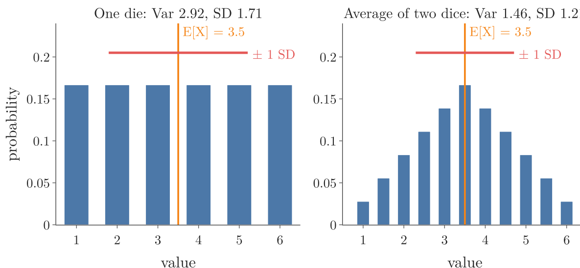
Figure 7: One die and the average of two dice: same expected value, different variance
