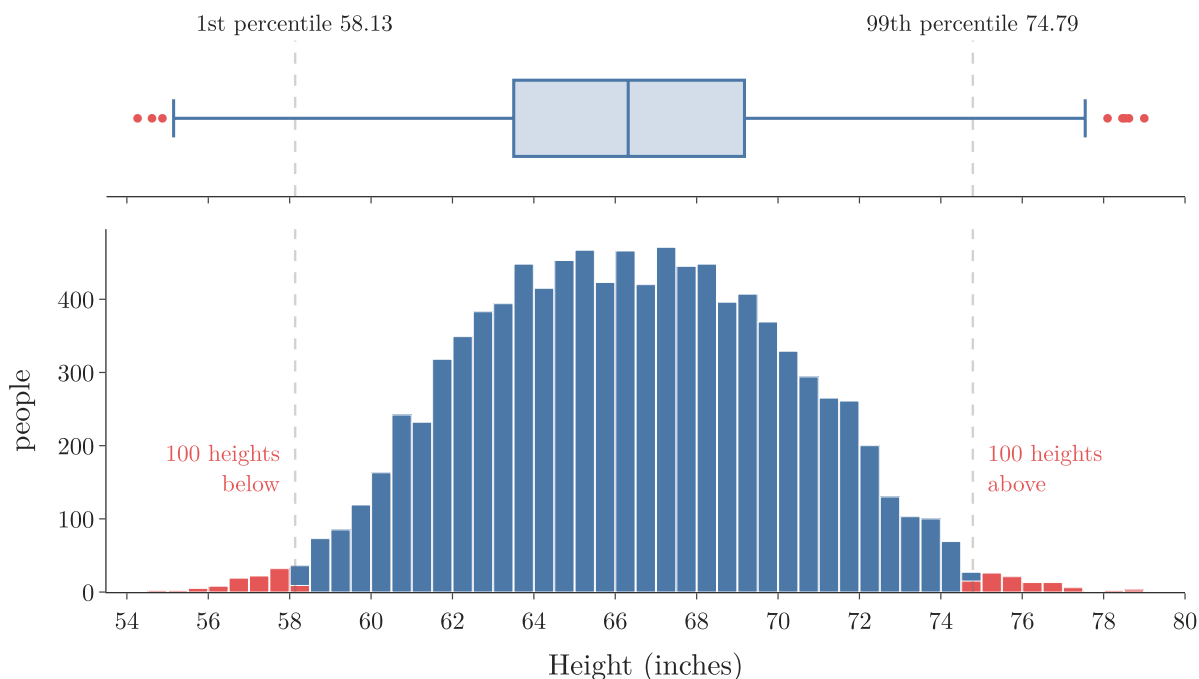
Figure 3: Height of 10,000 people: box plot above, histogram below, with the 1st and 99th percentiles dashed and the 200 values outside them in red
