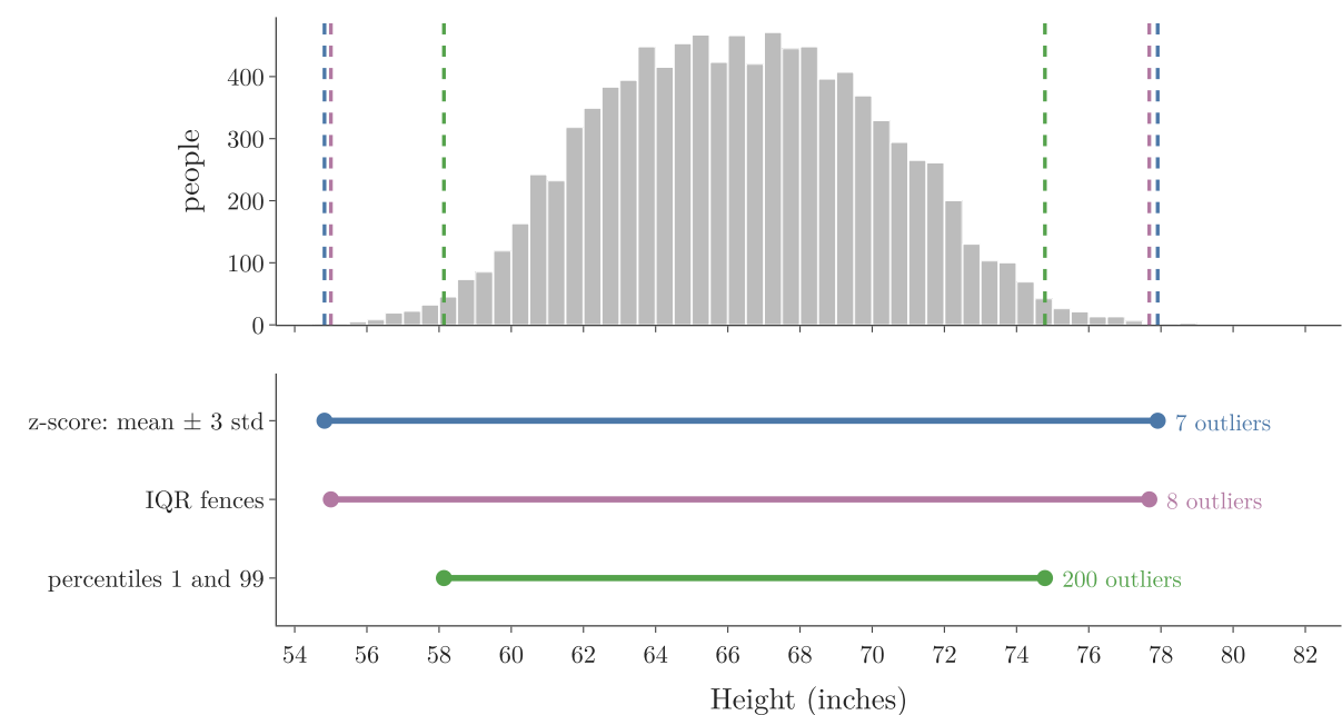
Figure 7: The three detection rules on Height: the z-score and IQR limits lie close to the ends and flag 7 and 8 values; the 1st and 99th percentiles lie further in and flag 200
