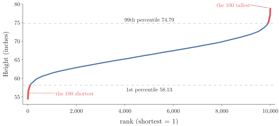
Figure 2: The 10,000 heights sorted by rank; the 1st and 99th percentiles are the heights at ranks 100 and 9,900, and the 100 shortest and 100 tallest lie beyond them
