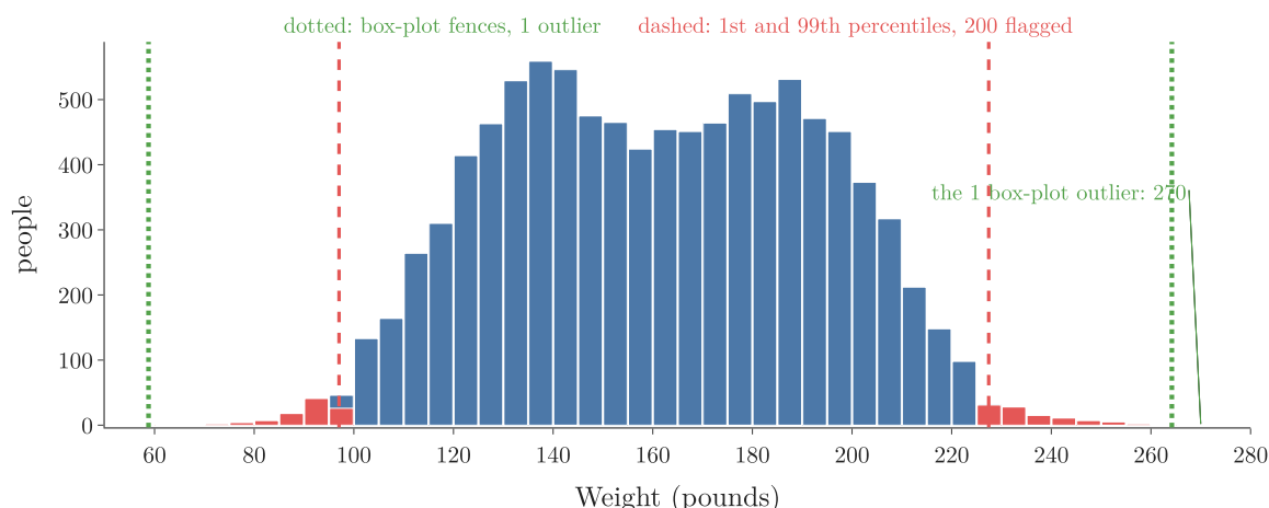
Figure 6: Weight: the box-plot fences (green, dotted) flag 1 value, at 270 pounds; the 1st and 99th percentiles (red, dashed) flag 200
