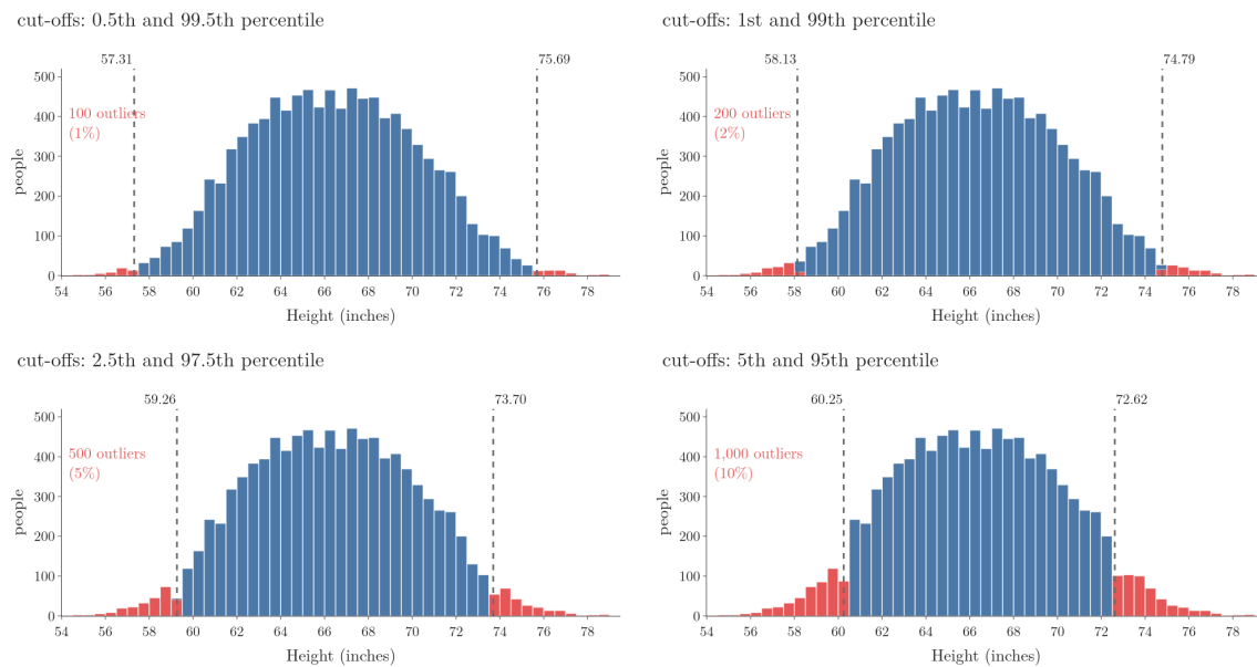
Figure 5: Sliding the cut-offs inwards on Height: the limits move in and the share flagged grows from 100 (1%) to 1,000 (10%)
