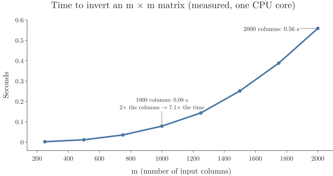
Figure 5: Time to invert a matrix as its size grows
