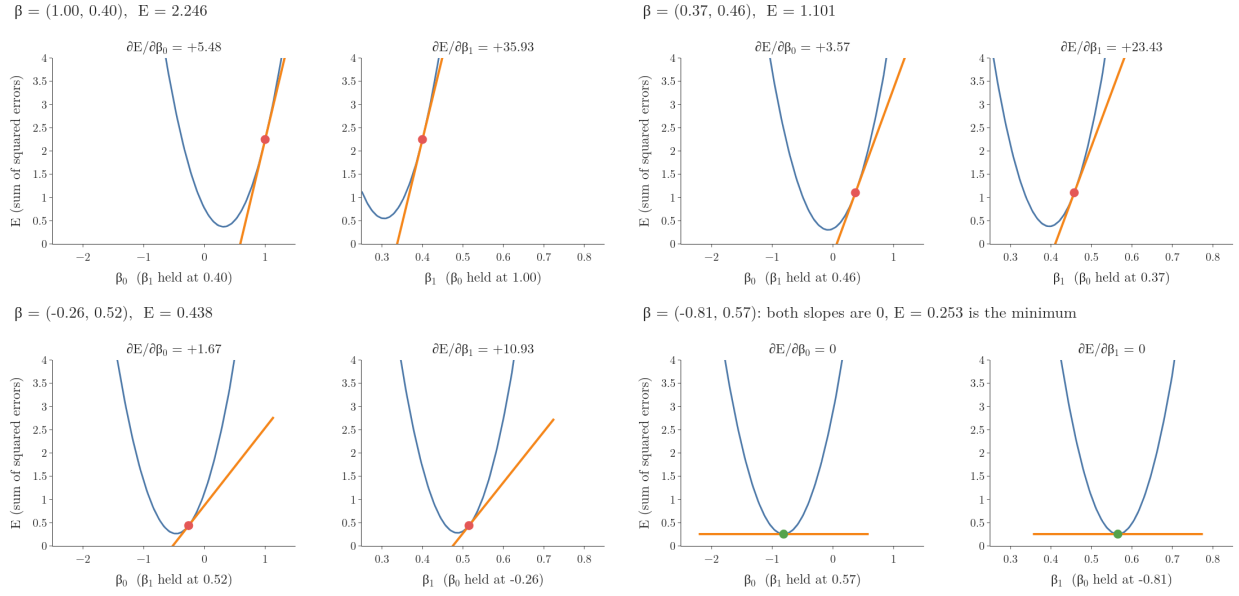
Figure 3: The gradient -2X^T y + 2X^T X \beta on the four students: each panel is the error E along one coefficient, the orange tangent's slope is one entry of the gradient, and both reach 0 together at \beta = (-0.81, 0.57)
