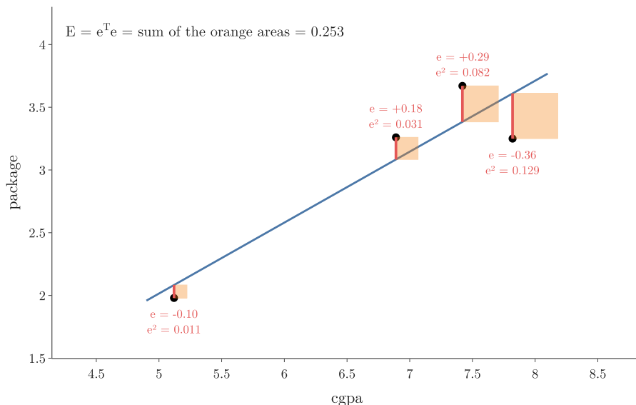
Figure 2: The four students of Section 6.1 and their best line: the residuals e (red) and their squares (orange); E = e^T e = 0.253 is the total orange area
