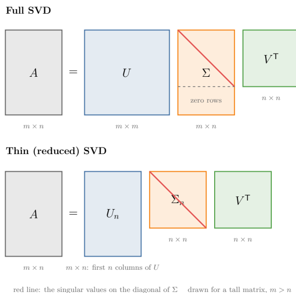
Figure 9: Shapes of the factors in the full and in the thin SVD of a tall matrix
