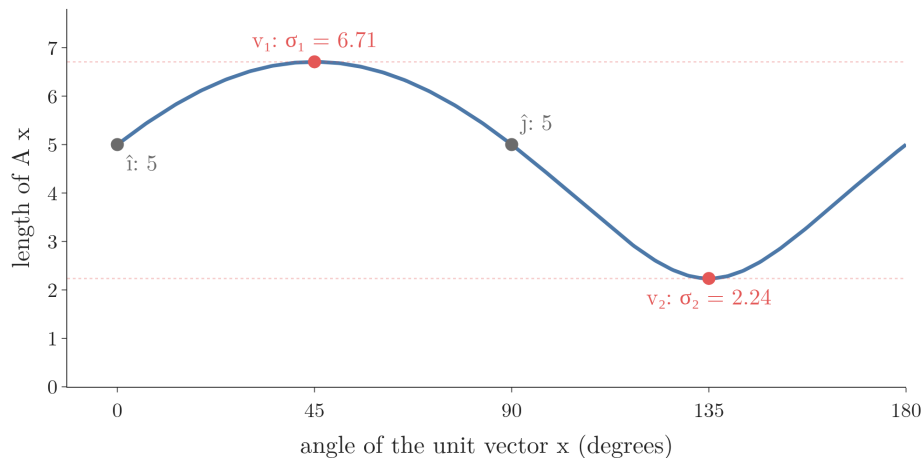
Figure 7: The length of A\mathbf{x} for every unit vector \mathbf{x} , by its angle: the curve never leaves the band between \sigma_2 and \sigma_1
