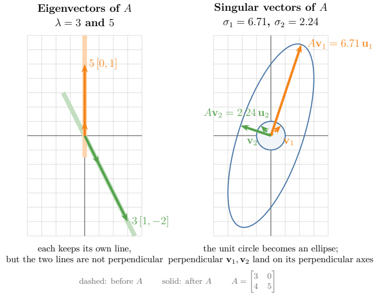
Figure 5: Eigenvectors keep their line; singular vectors are the perpendicular pair that stays perpendicular
