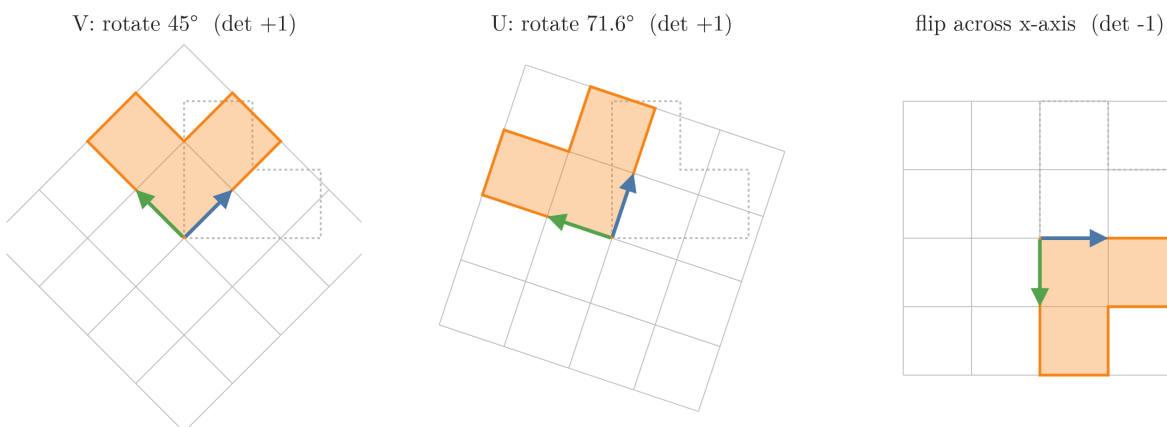
Figure 3: The three orthogonal matrices of this Note acting on a grid and an L-shaped tile (dotted: before; orange: after). Arrows: where \hat{i} (blue) and \hat{j} (green) land
