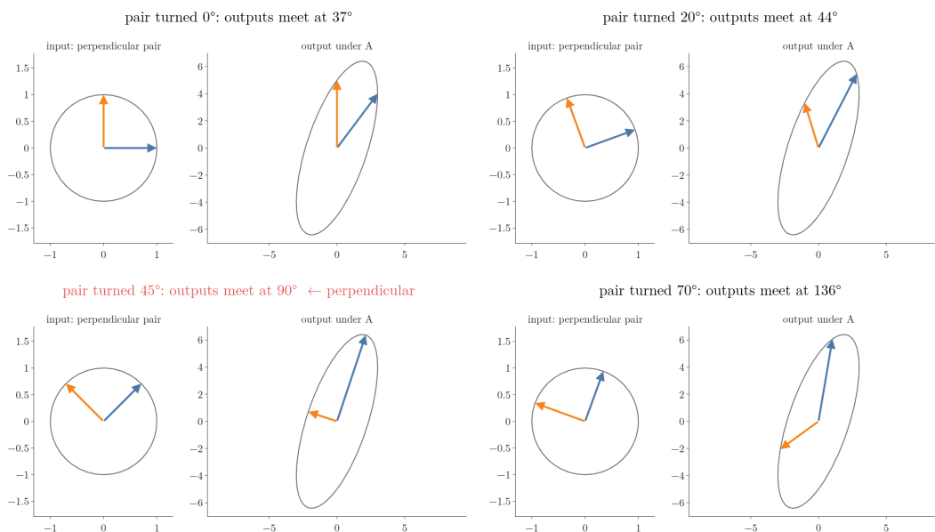
Figure 4: A perpendicular pair of unit vectors (left) turns in 5^\circ steps; A sends it to the pair on the right. The title gives the angle between the two outputs
