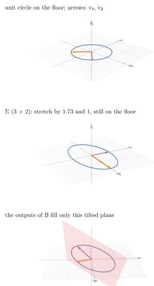
Figure 8: The SVD of the 3 \times 2 matrix B in 3D. The unit circle lies on the floor (third coordinate 0) with \mathbf{v}_1 (orange) and \mathbf{v}_2 (purple). V^T turns it on the floor, \Sigma stretches it into an ellipse of axes 1.73 and 1, still on the floor, and U tilts it up onto the plane of B 's outputs (red). The dashed curve is B applied in one step. 2D-to-3D picture after 3Blue1Brown, “Nonsquare matrices as transformations between dimensions”
