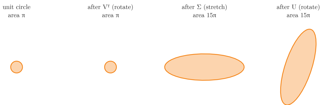
Figure 6: Area of the unit circle after each factor: the two rotations keep it at \pi , the stretch \Sigma multiplies it by \sigma_1\sigma_2 = 15
