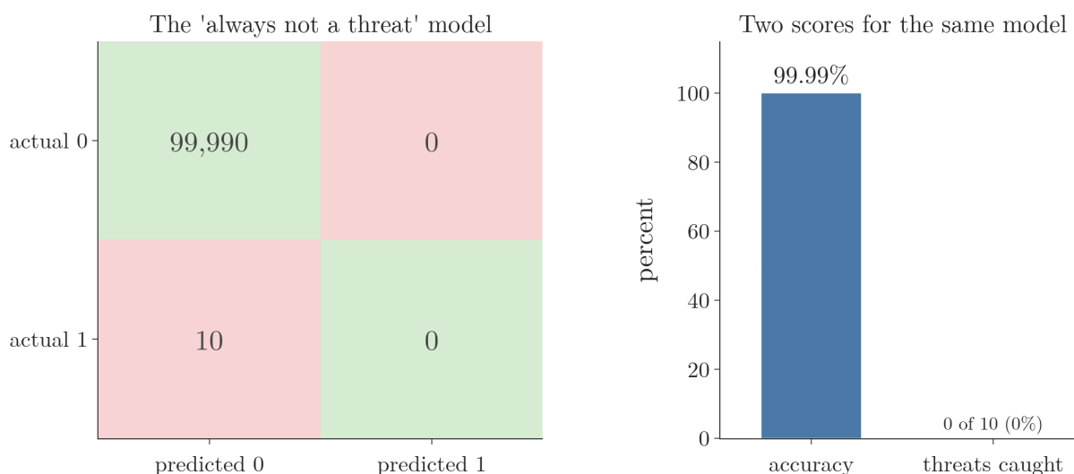
Figure 5: The “always not a threat” model on 100,000 passengers. Left: its confusion matrix. Right: its accuracy against the share of threats it catches.
