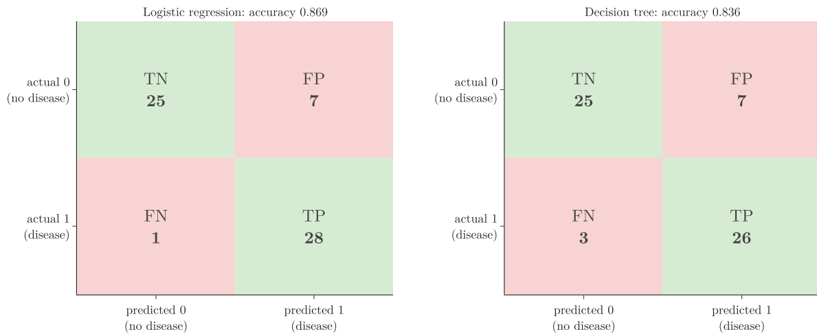
Figure 2: Confusion matrices for logistic regression and the decision tree
