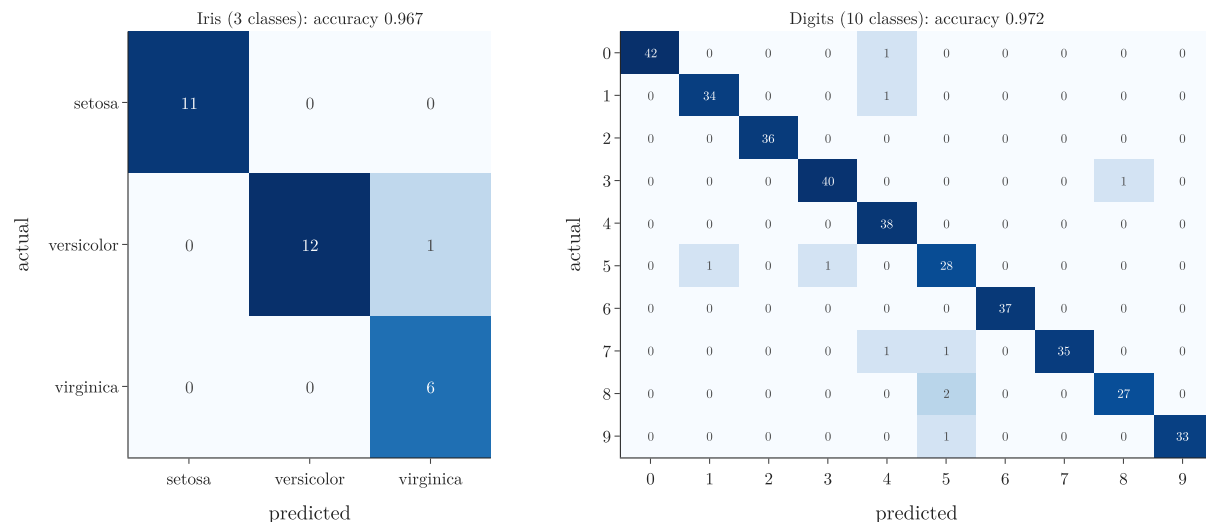
Figure 4: Confusion matrices for iris (3 classes) and digits (10 classes)
