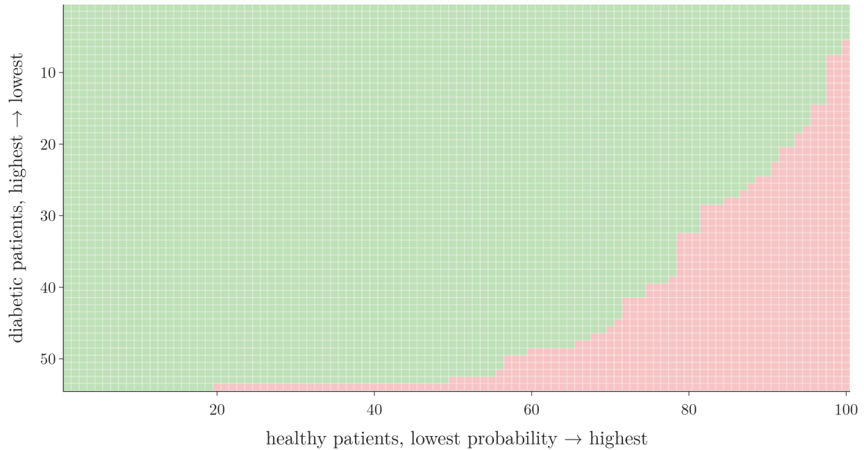
Figure 5: All 5,400 pairs of one diabetic and one healthy test patient. A cell is green when the diabetic patient gets the higher predicted probability, pink when the healthy one does.
