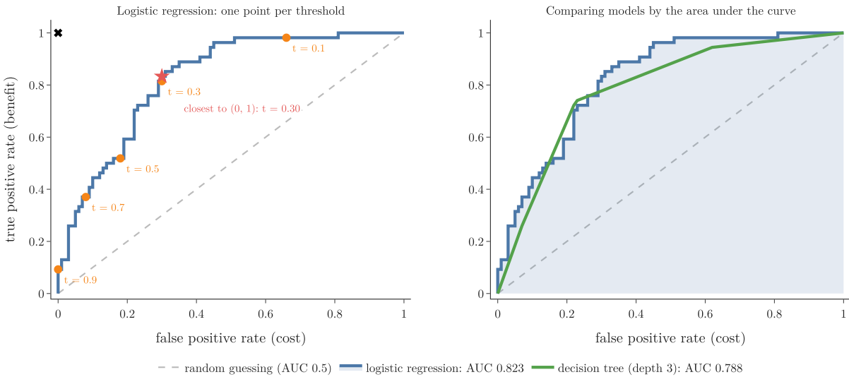
Figure 4: The ROC curve with five thresholds marked, and two models compared
