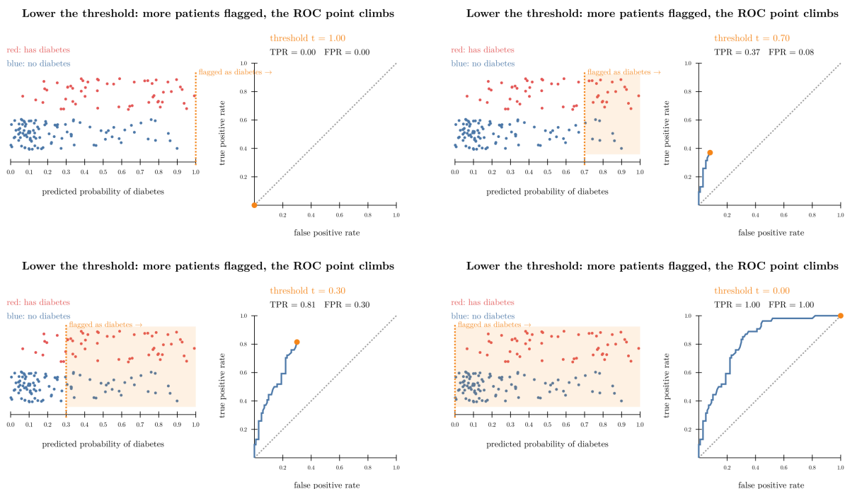
Figure 3: Lowering the threshold traces out the ROC curve
