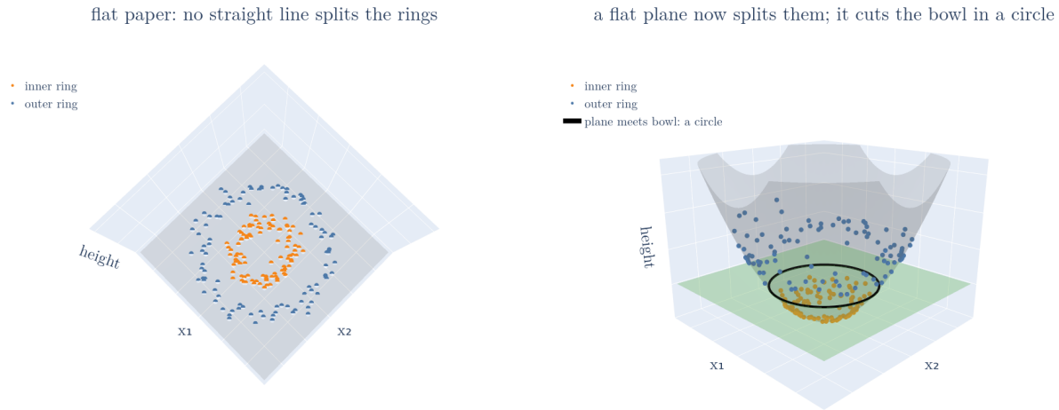
Figure 1: Two rings of points. Flat: no straight line separates them. Lifted to height x_1^2 + x_2^2 (the squared features), a flat plane separates them, and the plane meets the bowl in a circle
