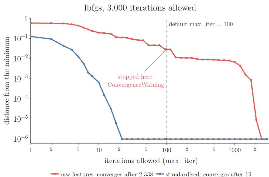
Figure 4: lbfgs on raw (red) and standardised (blue) breast-cancer features: distance from the minimum against iterations allowed. Points at the bottom are within one millionth of the minimum. The dashed line is the default max_iter = 100
