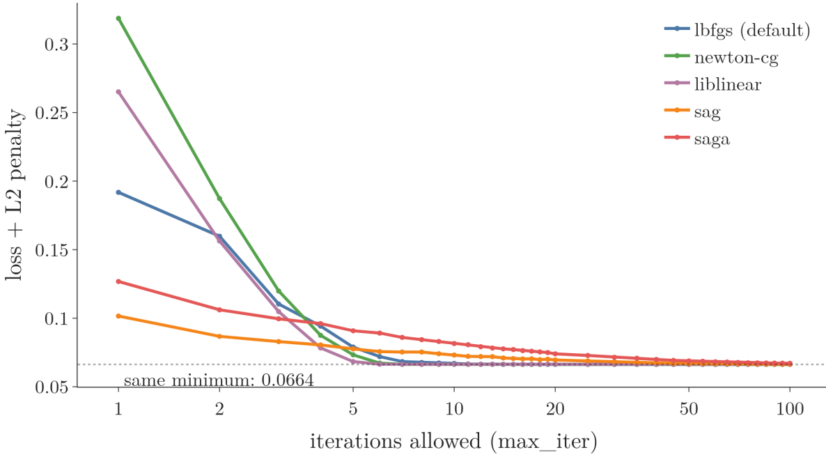
Figure 3: Five solvers on the standardised breast-cancer data (L2, C = 1 ): log loss plus penalty after k iterations. All reach the same minimum, 0.0664
