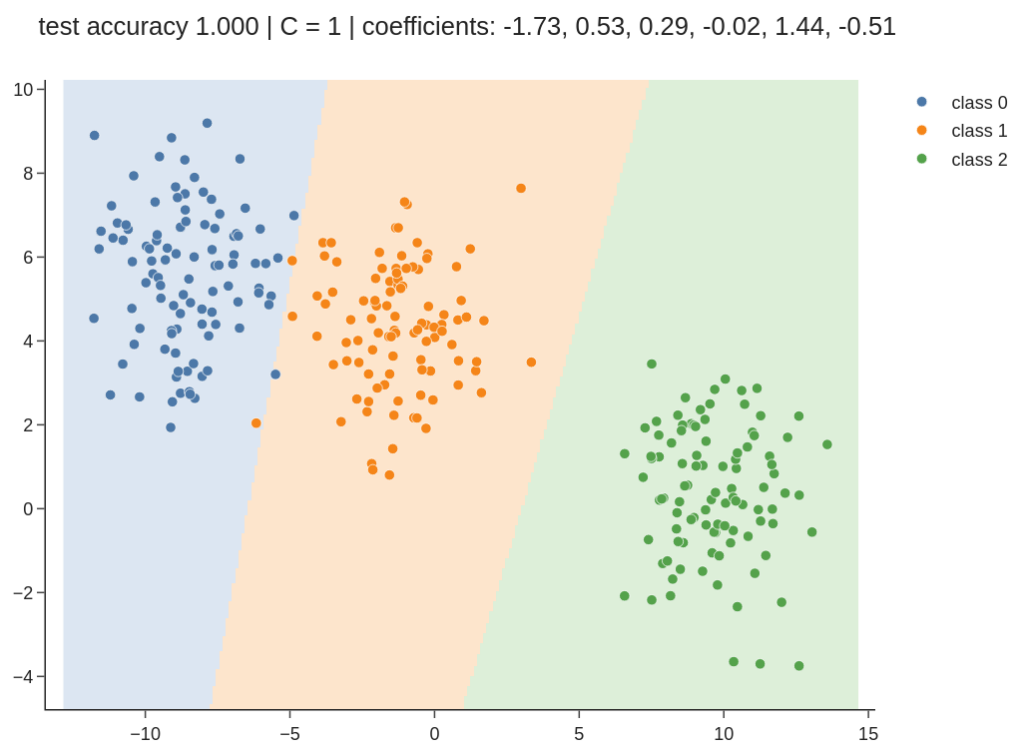
Figure 6: The playground on the three-class dataset with the default settings
