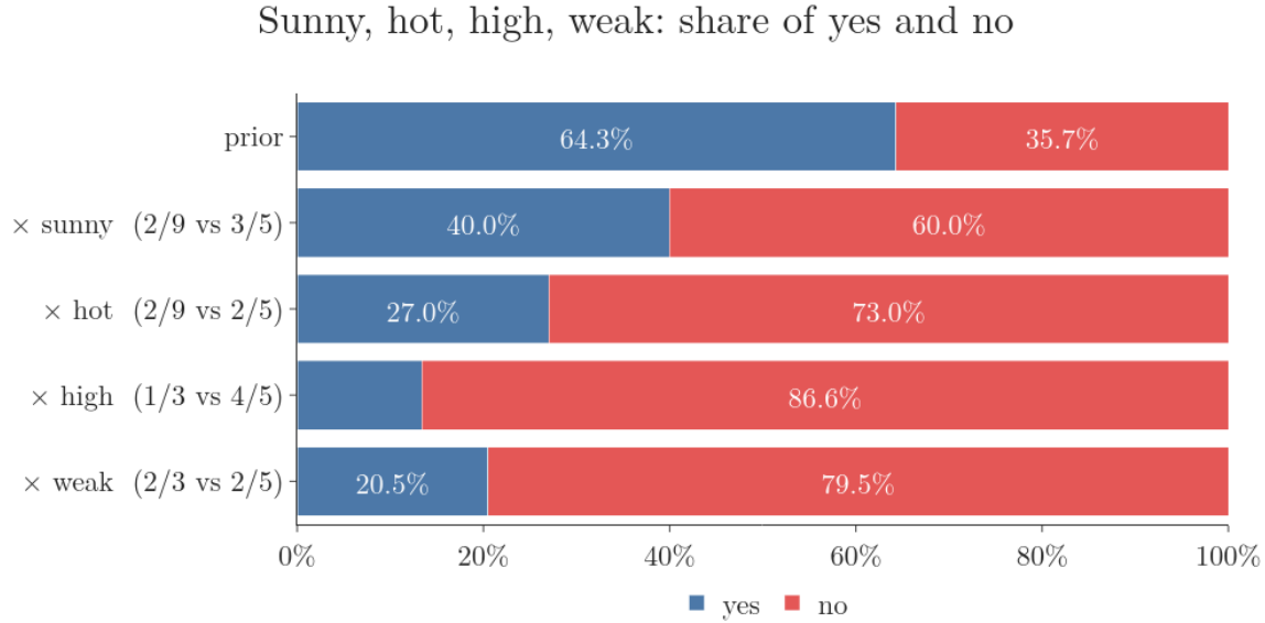
Figure 3: The sunny, hot, high, weak day, one factor at a time. Each bar is the yes/no share of the running product; brackets give P(\text{value} \mid \text{yes}) vs P(\text{value} \mid \text{no})
