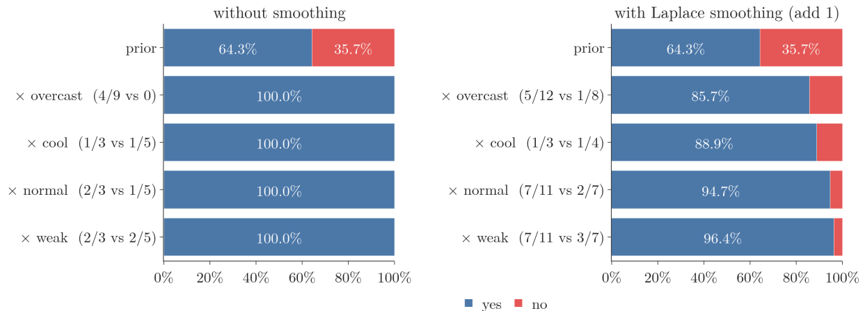
Figure 5: The overcast day without (left) and with (right) Laplace smoothing. Smoothed factors such as 1/8 for P(\text{overcast} \mid \text{no}) keep every class alive: 96.4% yes instead of 100%
