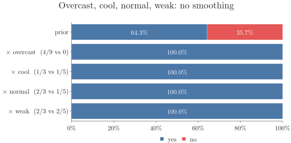
Figure 4: The overcast, cool, normal, weak day without smoothing. The factor P(\text{overcast} \mid \text{no}) = 0 sets the no share to 0 for good
