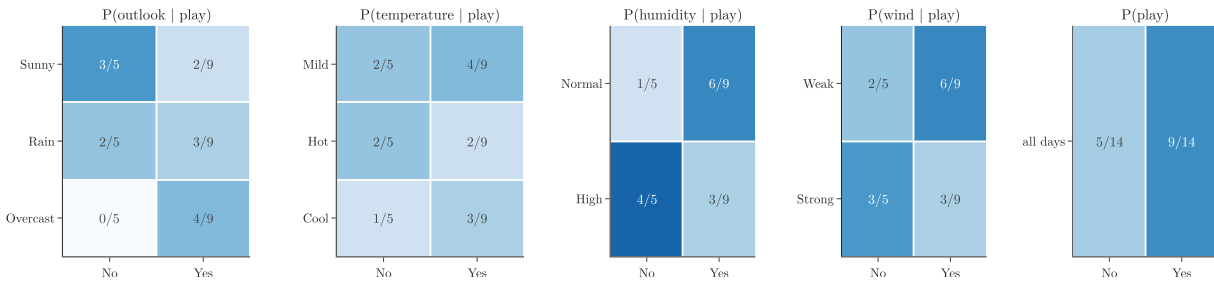
Figure 2: The full lookup table: P(\text{value} \mid \text{play}) for every feature, and P(\text{play})
