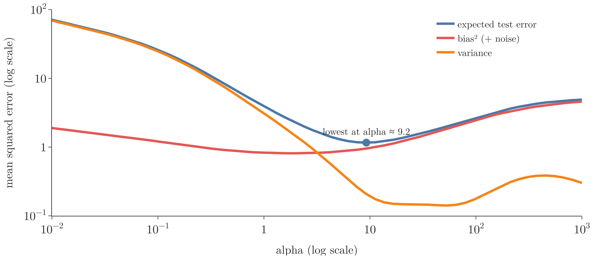
Degree-15 polynomial with Ridge: more alpha, less variance, more bias
