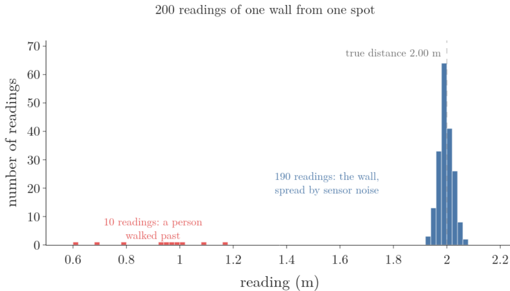
Figure 4: A histogram of 200 readings of one wall from one spot: 190 cluster around 2.00 m between 1.92 and 2.07 m, and 10 readings taken while a person walked past lie between 0.6 and 1.2 m
