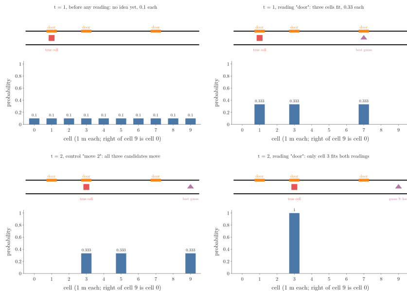
Figure 6: Animation: after the reading “door” the distribution keeps cells 1, 3 and 7 while a best guess picks cell 7; after “move 2” the candidates become cells 3, 5 and 9; after a second “door” only cell 3 fits, while the best guess at cell 9 expected a wall and is lost
