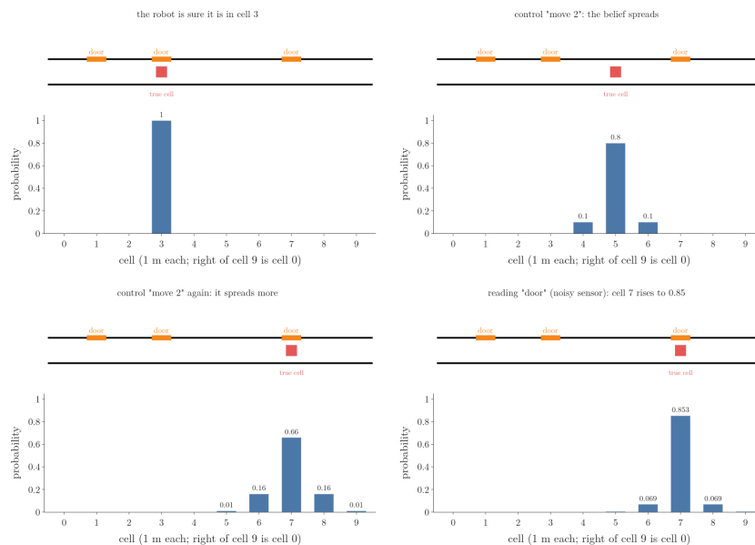
Figure 10: Animation: the robot is sure it is in cell 3; after one noisy move the probabilities are 0.1, 0.8, 0.1 at cells 4, 5, 6; after a second move 0.01, 0.16, 0.66, 0.16, 0.01 at cells 5 to 9; the noisy reading “door” lifts the door cell 7 to 0.853 and lowers cells 6 and 8 to 0.069
