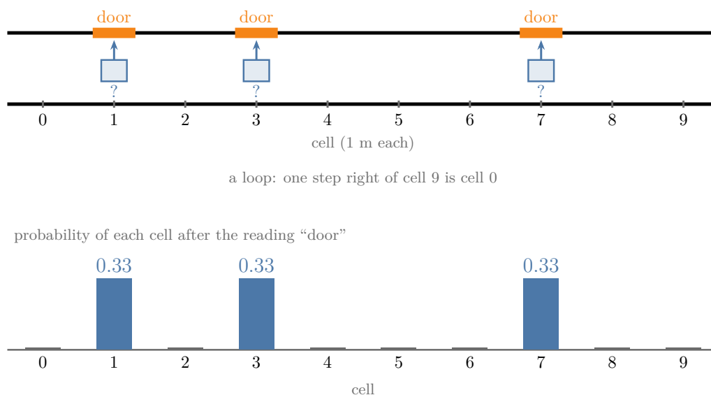
Figure 1: A hallway of 10 cells of 1 m, numbered 0 to 9 and joined into a loop, with doors at cells 1, 3 and 7. The robot's sensor says "door". The robot could be at any of the three doors, so each of those cells gets probability 0.33
