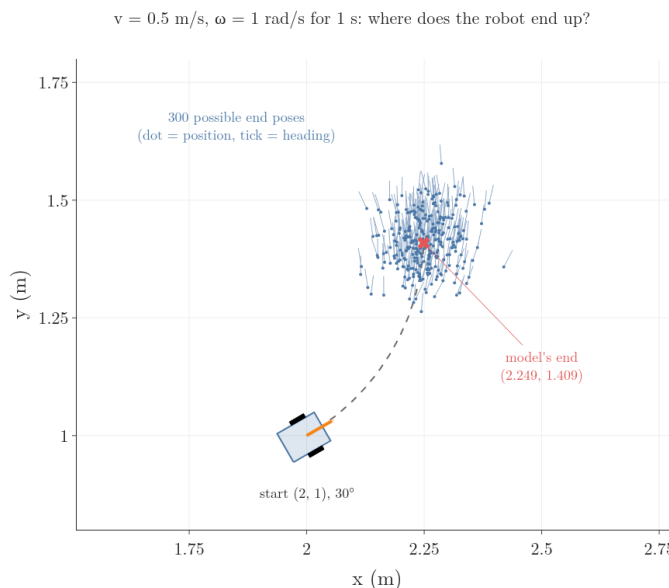
Figure 1: The robot at (2, 1) facing 30 degrees drives 0.5 m/s while turning 1 rad/s for 1 s. The kinematic model predicts one end pose, (2.249, 1.409); 300 sampled end poses form a cloud around it, each with a slightly different heading
