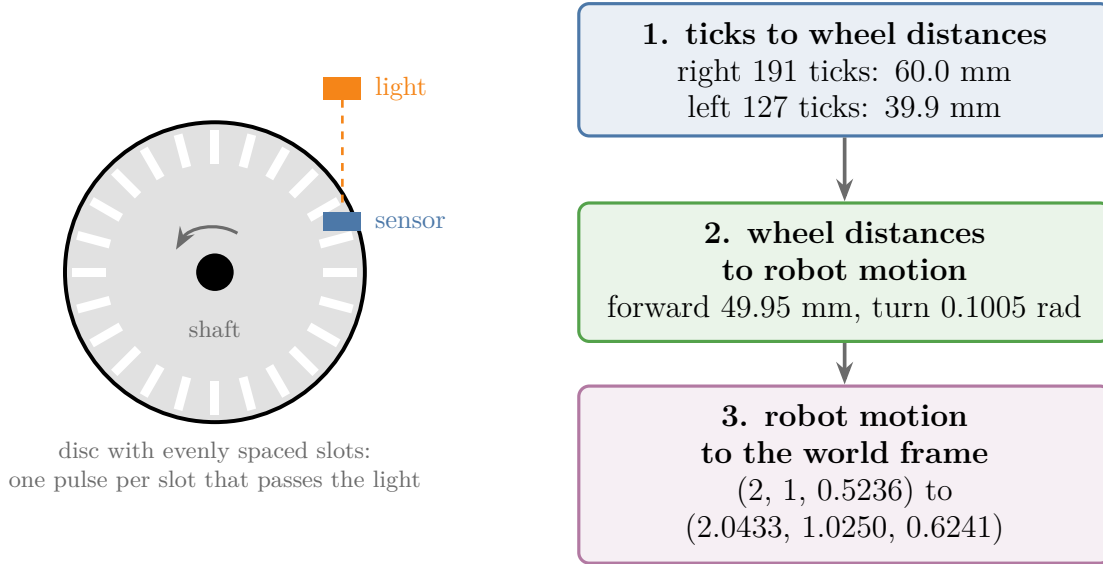
Figure 3: Left: an optical encoder, a slotted disc on the wheel shaft between a light and a sensor; each passing slot gives one tick. Right: the three steps of wheel odometry with the Note’s numbers: 191 and 127 ticks give wheel distances 60.0 mm and 39.9 mm, which give a forward move of 49.95 mm and a turn of 0.1005 rad, which move the pose from (2, 1, 0.5236) to (2.0433, 1.0250, 0.6241)
