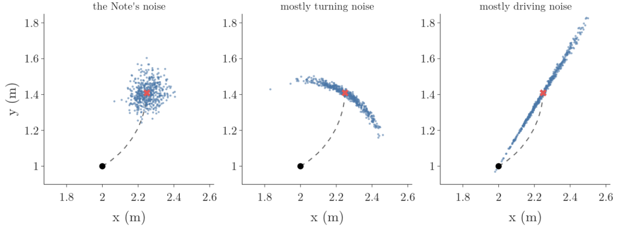
Figure 7: 500 sampled end positions for the same odometry reading under three noise settings: the Note's noise gives a round cloud around (2.249, 1.409); mostly turning noise bends it into a banana around the start; mostly driving noise stretches it along the line from the start
