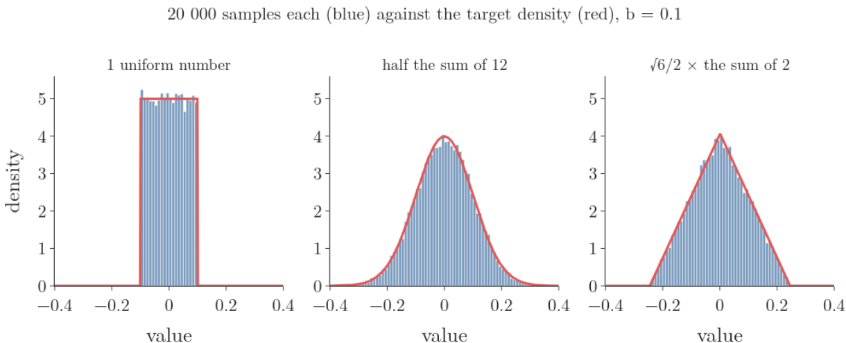
Figure 6: Left: 20 000 uniform numbers between -0.1 and 0.1 form a flat block. Middle: half the sum of 12 of them forms a bell that matches the normal density with standard deviation 0.1. Right: the square root of 6 over 2 times the sum of 2 of them forms a triangle that matches the triangular density with standard deviation 0.1
