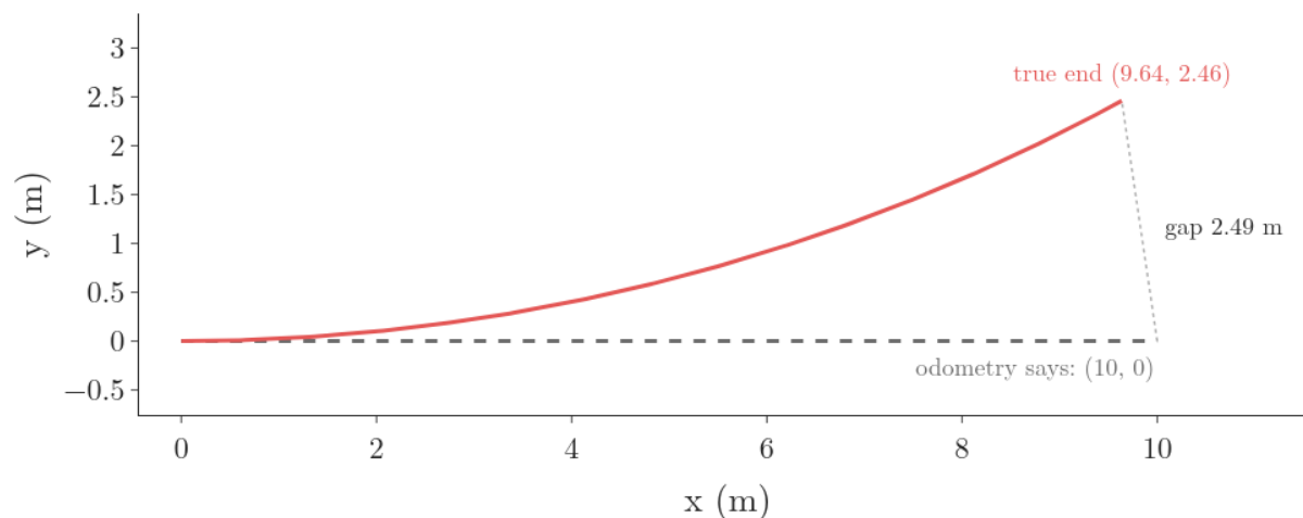
Figure 4: A robot whose right wheel is 1 percent larger than the model thinks: odometry says it drove straight to (10, 0); really it curved left to (9.64, 2.46), 2.49 m away
