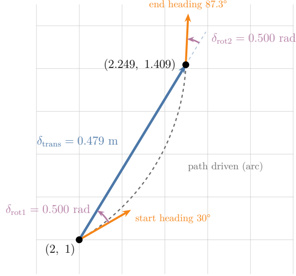
Figure 5: Odometry from (2, 1) facing 30 degrees to (2.249, 1.409) facing 87.3 degrees, as turn, drive, turn: first turn 0.500 rad to face the end point, drive 0.479 m along the straight line, second turn 0.500 rad to the end heading. The robot really drove the dashed arc
