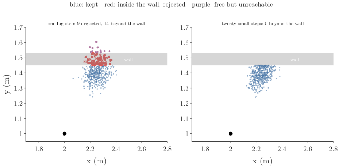
Figure 11: Left: one big step of 0.48 m; of 500 samples, 95 land inside a wall and are rejected, but 14 land beyond the wall in free space and are kept, though the robot could not have driven through the wall. Right: the same motion in twenty small steps, rejecting and redrawing at each step: no sample gets beyond the wall
