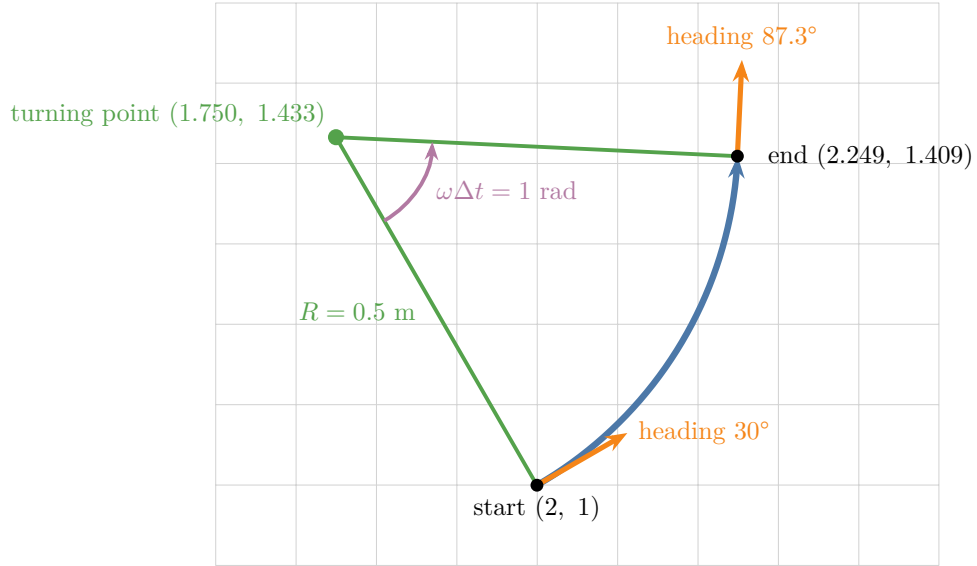
Figure 9: The velocity model without noise: v = 0.5 m/s and \omega = 1 rad/s give a turning radius of 0.5 m; the turning point (1.750, 1.433) lies 0.5 m to the robot's left; in 1 s the robot turns 1 rad about it and ends at (2.249, 1.409) facing 87.3 degrees
