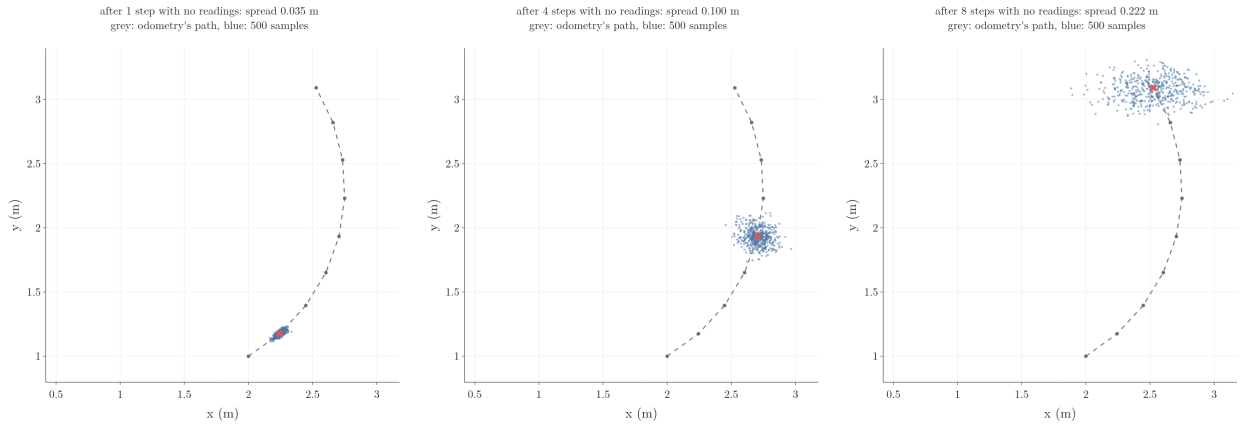
Figure 8: Animation: 500 samples follow odometry steps of turn 0.1 rad, drive 0.3 m, turn 0.1 rad from (2, 1); the cloud grows from 0.035 m after one step to 0.100 m after four and 0.222 m after eight, and bends along the curved path
