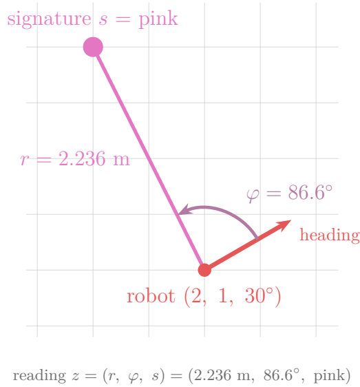
Figure 9: A landmark reading: from the robot at (2, 1) facing 30 degrees, the pink pole at (1, 3) is at range r = 2.236 \text{ m} and bearing \varphi = 86.6 degrees from the heading; its signature is pink
