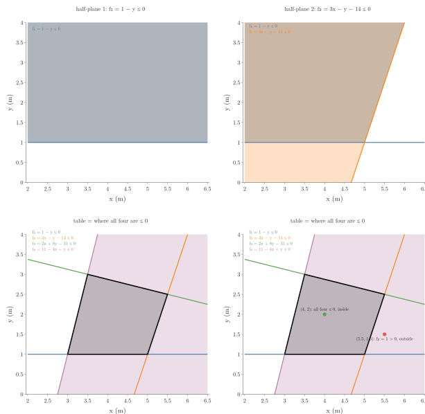
Figure 4: Animation: the half-planes f_1 = 1 - y \leq 0 , f_2 = 3x - y - 14 \leq 0 , f_3 = 2x + 8y - 31 \leq 0 and f_4 = 11 - 4x + y \leq 0 are shaded one at a time; the region inside all four is the table. The point (4, 2) gives all four values at most 0 and is inside; the point (5.5, 1.5) gives f_2 = 1 and is outside
