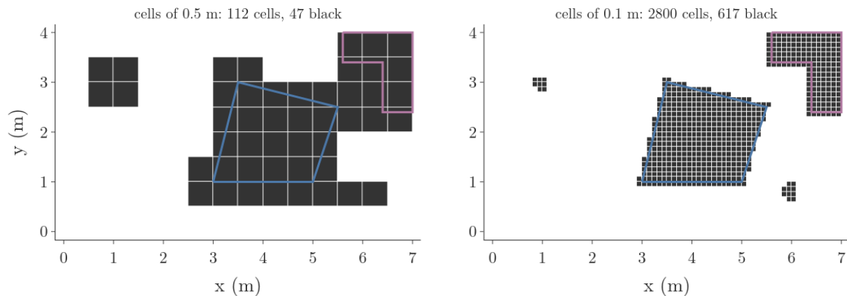
Figure 7: Bitmaps of the room’s furniture: with 0.5 m cells, 112 cells of which 47 are black, a coarse blocky outline; with 0.1 m cells, 2800 cells of which 617 are black, close to the true table, cabinet and poles drawn as outlines
