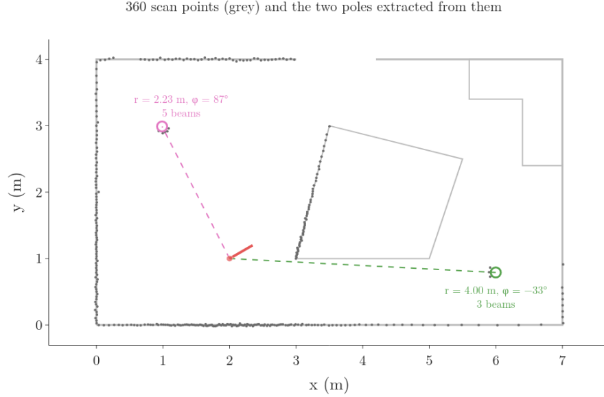
Figure 8: 360 scan points from the robot at (2, 1) facing 30 degrees: grey dots along the walls and the table’s near side; two small clusters are extracted as poles, the pink one at range 2.23 m and bearing 87 degrees from 5 beams, the green one at range 4.00 m and bearing -33 degrees from 3 beams
