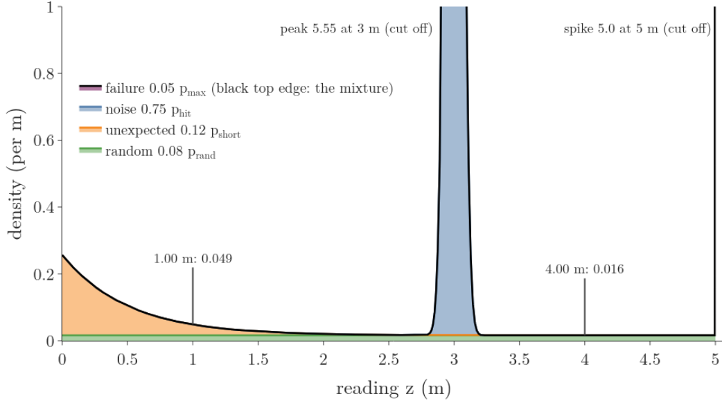
Figure 7: The beam model for an expected range of 3 m, built by stacking the weighted parts: a green floor (random), an orange falling curve up to 3 m (unexpected objects), the blue bell at 3 m (measurement noise, cut off at the top) and the purple spike at 5 m (failure). The black top edge is the mixture; it is 0.049 at 1.00 m and 0.016 at 4.00 m
