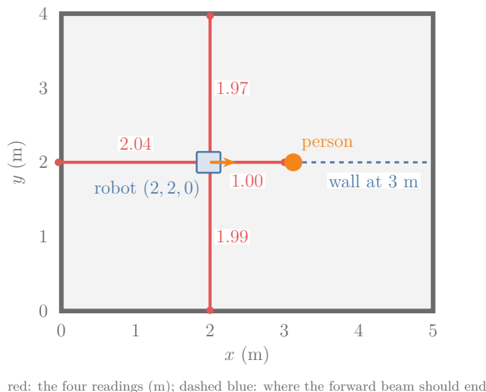
Figure 1: A 5 m by 4 m room seen from above. The robot at (2, 2), facing along x, sends four laser beams. The forward beam should reach the wall 3 m away but stops at a person 1 m ahead; the other three read 1.97, 2.04 and 1.99 m
