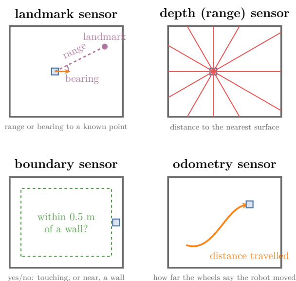
Figure 10: Four kinds of sensors in the 5 m by 4 m room: a landmark sensor measures range or bearing to a known point; a depth sensor measures distances to the nearest surface along many beams; a boundary sensor says whether the robot touches or is near a wall; an odometry sensor reports how far the wheels say the robot moved
