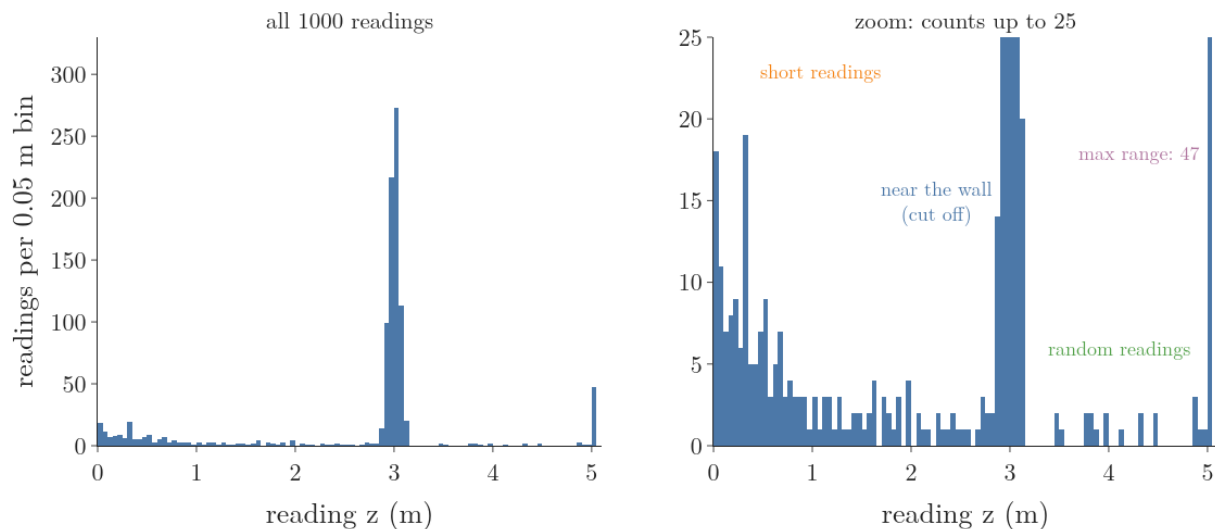
Figure 8: 1000 readings of a wall 3 m away as counts per 0.05 m bin. Left: a tall peak at 3 m. Right, zoomed to counts up to 25: a falling pile of short readings near 0, a thin floor of random readings, and a bar of 47 readings at the maximum range of 5 m
