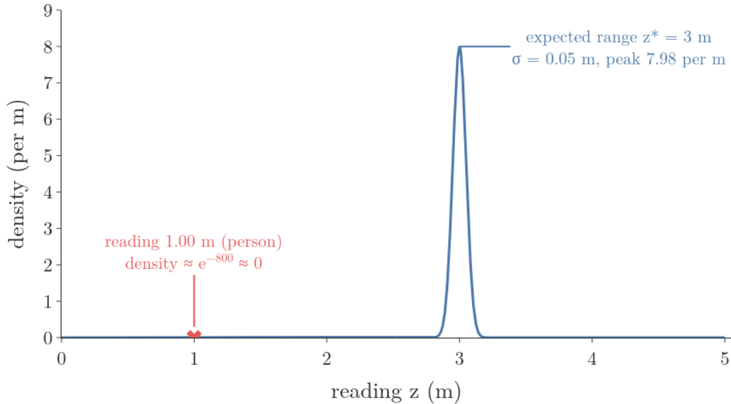
Figure 3: A Gaussian of spread 0.05 m around the expected range 3 m. The reading 1.00 m, caused by a person, sits far out in the tail, where the density is about e to the minus 800, effectively 0
