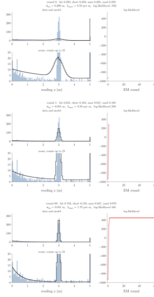
Figure 9: Animation of EM fitting the beam model. Each frame is one round: blue bars are the 1000 readings, the black line is how many readings the current model expects per bin, the right panel is the log-likelihood. Round 0 is a flat, wide guess with log-likelihood -932 ; by round 60 the weights are hit 0.733, short 0.150, max 0.047, rand 0.070, sigma 0.051 m, lambda 1.75 per m, log-likelihood 448
