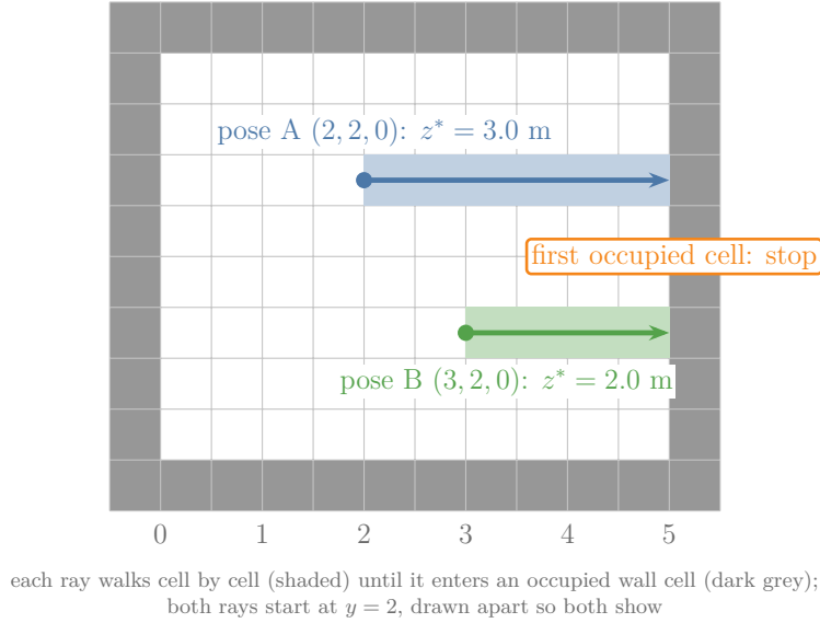
Figure 2: Ray casting in a grid map: from pose A at (2, 2) the forward ray walks cell by cell and enters the wall cells after 3.0 m; from pose B at (3, 2) it does so after 2.0 m
