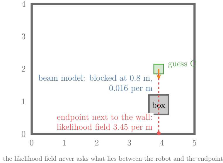
Figure 8: A guessed pose C above the box, facing down. A reading of 1.98 m would end next to the bottom wall, which the likelihood field scores 3.45 per m; the beam model knows the box blocks the beam after 0.8 m and gives 0.016 per m
