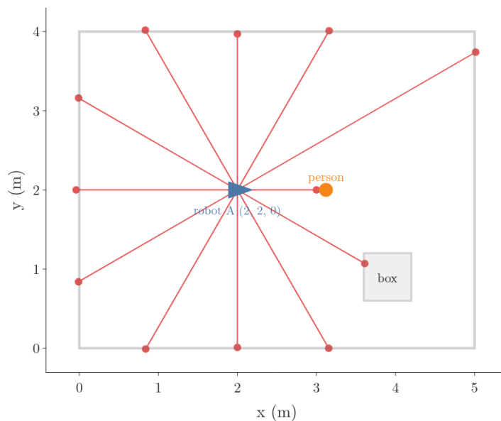
Figure 1: The 5 m by 4 m room with a box in the lower right. The robot at pose A (2, 2, 0) sends 12 laser beams, one every 30 degrees; each beam ends at a red dot on a wall or on the box, except the forward one, which stops at a person 1 m ahead
