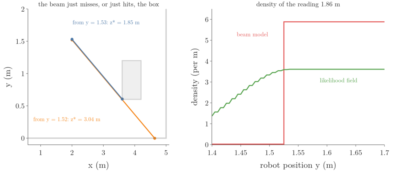
Figure 2: Left: one beam at 330 degrees from the robot at y = 1.53 m hits the box after 1.85 m; from y = 1.52 m it passes under the box and hits the bottom wall after 3.04 m. Right: as the robot position y changes, the beam model’s density of the reading 1.86 m jumps from 0.022 to 5.88 at y = 1.525 , while the likelihood field rises smoothly
