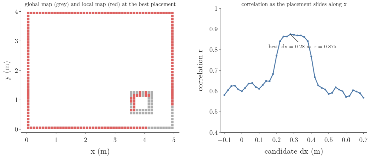
Figure 10: Left: the global map (grey cells along the walls and around the box) with the local map of scan 2 (red cells) placed at the best candidate; the red cells cover the walls and the two box faces the robot can see. Right: the correlation as the candidate dx slides from -0.1 to 0.7 m, about 0.6 at the ends with a flat top near 0.87 between 0.24 and 0.36 m, best at 0.28 m
