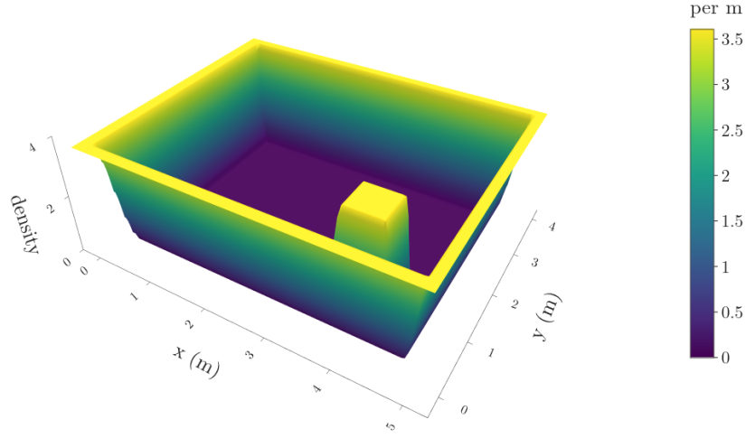
Figure 6: The likelihood field of the room drawn as a 3D surface, seen from above at a slant: high yellow ridges along the four walls and around the box, a flat dark floor elsewhere; colour and height both show the density
