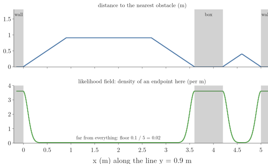
Figure 5: Along the line y = 0.9 m across the room. Top: the distance to the nearest obstacle, zero at the left wall, the box and the right wall, rising linearly away from each and levelling off at 0.9 m, the distance to the bottom wall. Bottom: the likelihood field, a plateau of 3.61 on each obstacle that drops to the floor of 0.02 within about 0.3 m
