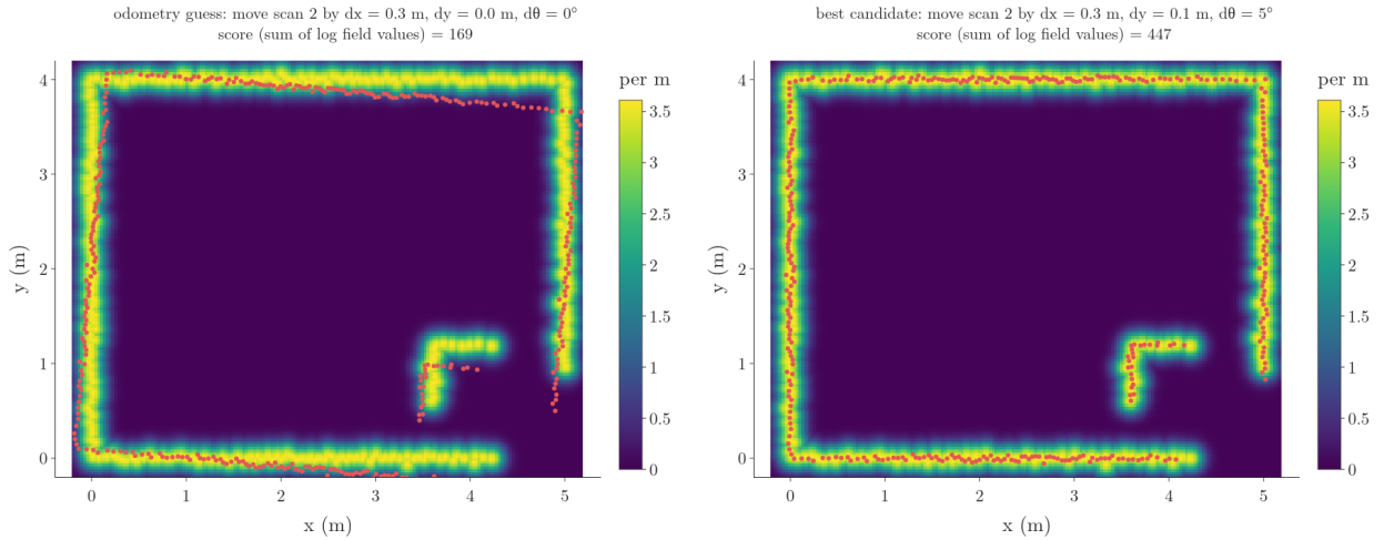
Figure 9: Animation over the likelihood field built from scan 1 (bright = near a scan-1 end point). Red dots are scan 2’s end points placed by a candidate motion. At the odometry guess (0.3, 0, 0) they sit beside the bright ridges, score 169; at the best candidate (0.3, 0.1, 5^\circ) they lie on the ridges, score 447
