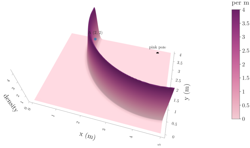
Figure 4: The density of the pink pole’s range reading over every robot position in the room, drawn as a surface: a curved ridge of radius 3.10 m around the pink pole, about 0.2 m wide, with the true position A on its crest
