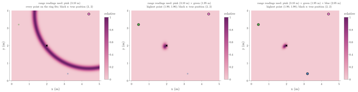
Figure 5: Animation over the room: first the density of the pink range reading, a ring around the pink pole; then pink times green, which leaves one bright spot near (1.9, 2.0); then pink times green times blue, one sharp spot at (1.90, 1.98) next to the true position (2, 2), marked by a black cross
