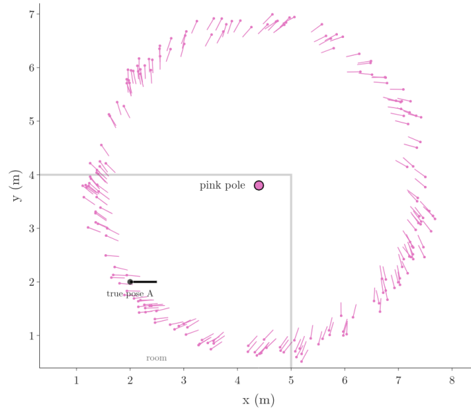
Figure 7: 200 poses drawn from the pink pole’s reading (3.10 m, 40 degrees): dots on a ring of radius about 3.1 m around the pole, each with a short arrow for its heading, turned so the pole appears 40 degrees to its left. The true pose A is on the ring; most of the ring lies outside the room
