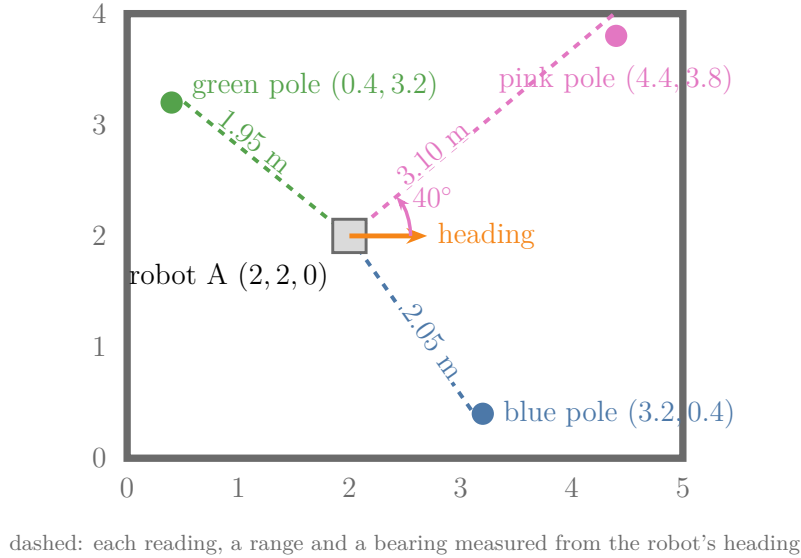
Figure 1: The 5 m by 4 m room with three coloured poles: pink at (4.4, 3.8), green at (0.4, 3.2), blue at (3.2, 0.4). The robot at A = (2, 2, 0) reads each one as a range and a bearing: pink 3.10 m at 40 degrees, green 1.95 m at 141 degrees, blue 2.05 m at -55 degrees
