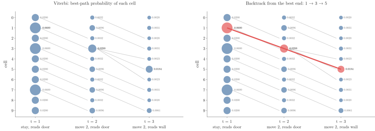
Figure 12: A trellis: time t = 1, 2, 3 across, cells 0 to 9 down. Each node shows the probability of the best path ending there and a grey line to its best predecessor. The largest value at t = 3 is 0.0184 at cell 5; following the back-pointers gives the red path 1, 3, 5
