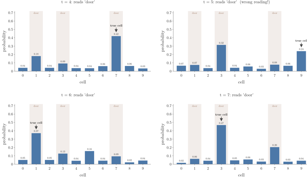
Figure 6: Seven steps of the histogram filter: orange frames show the predicted belief after each move, blue frames the belief after each reading; the tallest bar follows the true cell except at t = 5 , after the wrong reading, when it jumps to cell 3; at t = 6 and t = 7 it is back on the true cell
