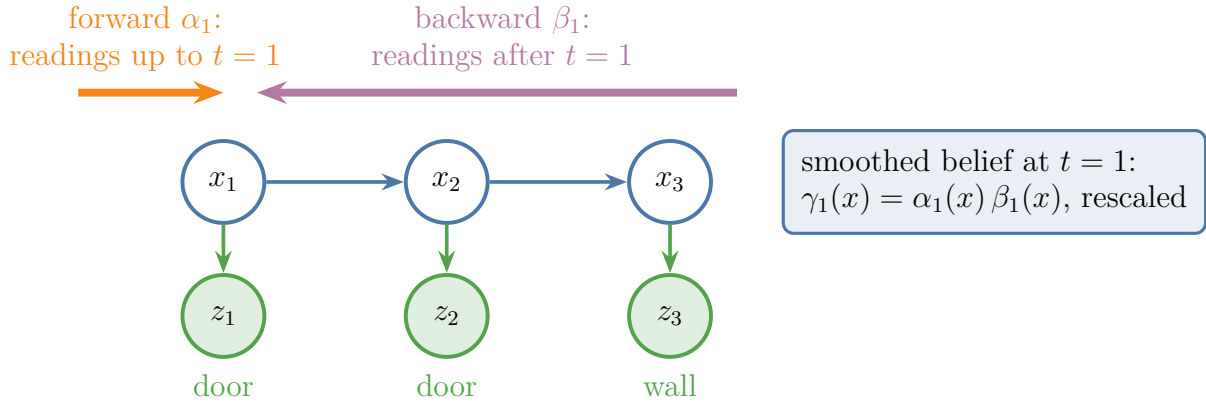
Figure 10: The chain x_1, x_2, x_3 with readings door, door, wall. A forward arrow \alpha_1 brings the evidence of readings up to t = 1 ; a backward arrow \beta_1 brings the evidence of readings after t = 1 ; their product, rescaled, is the smoothed belief
