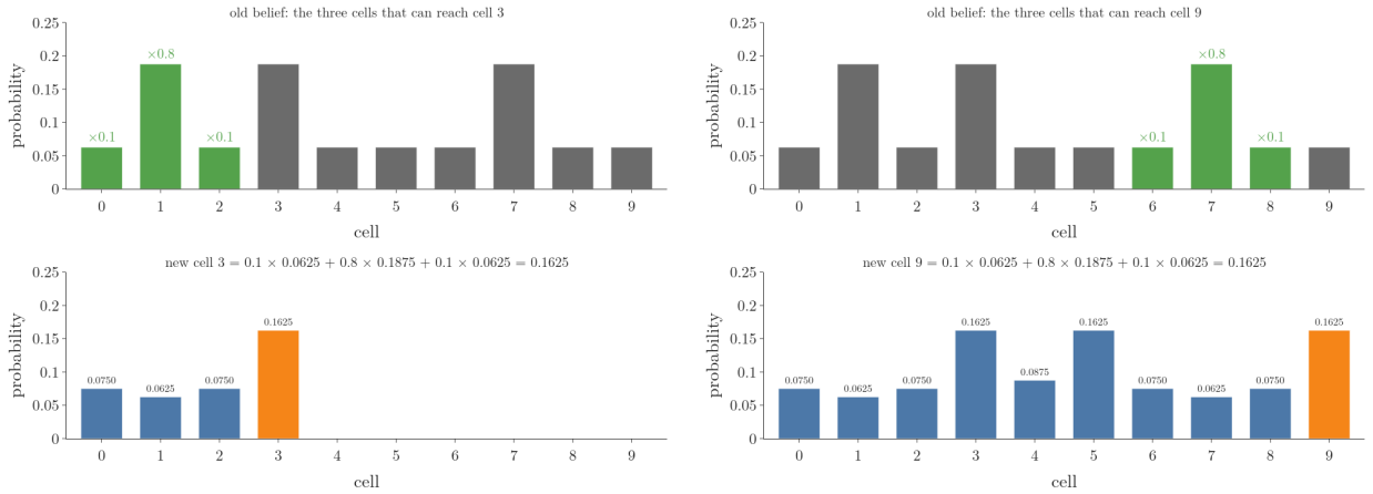
Figure 4: Top: the old belief with the three cells that can reach the new cell highlighted and weighted 0.1, 0.8 and 0.1. Bottom: the new belief filled in cell by cell; new cell 3 = 0.1 \times 0.0625 + 0.8 \times 0.1875 + 0.1 \times 0.0625 = 0.1625
