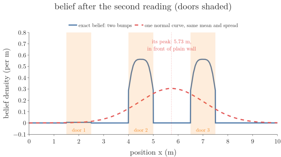
Figure 2: The exact belief after the second reading has two bumps, at door 2 and door 3; the single normal curve with the same mean and spread peaks at 5.73 m, in front of plain wall
