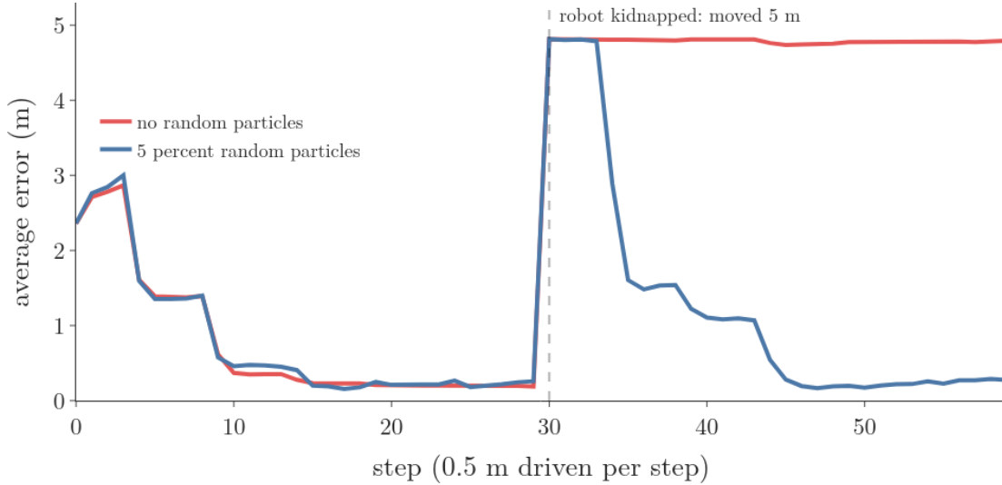
Figure 9: Average error over 200 runs. Both versions localize within about 15 steps. After the kidnap at step 30, the filter without random particles stays about 5 m off; with 5 percent random particles the error falls back below 0.3 m by step 45
