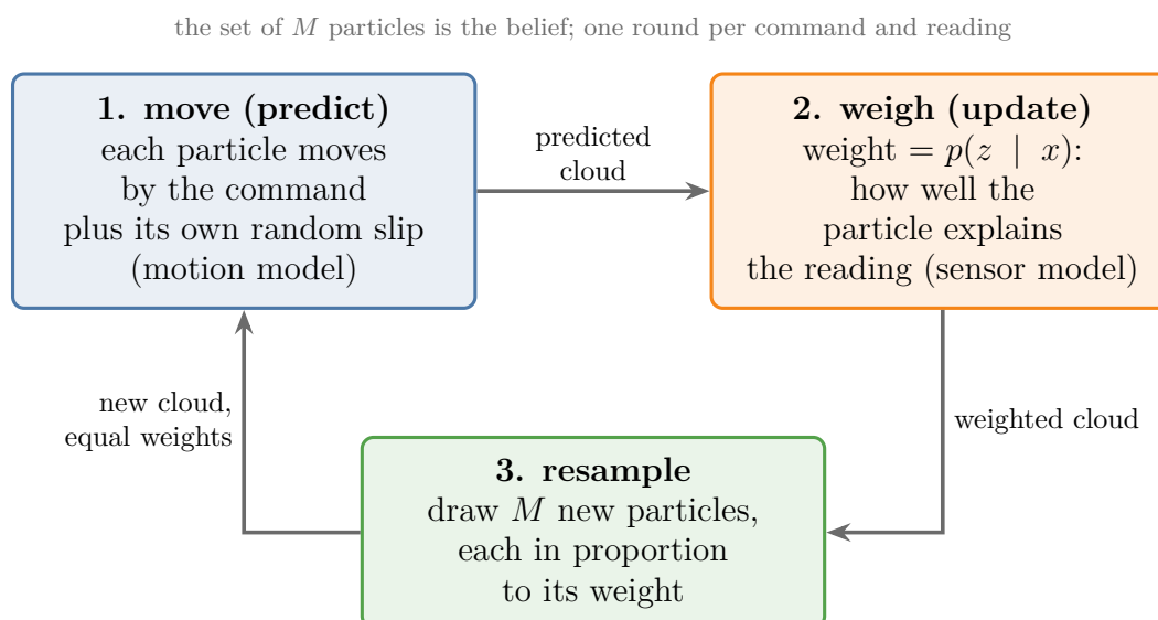
Figure 4: One round of the particle filter: move every particle by the command plus its own random slip; weigh each by p(z | x) ; resample M new particles in proportion to the weights
