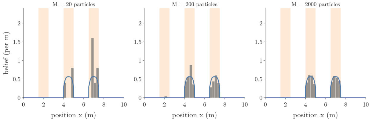
Figure 3: The particle histogram after the second reading against the exact belief: with 20 particles the bars are ragged, with 200 closer, with 2000 they follow the two bumps
