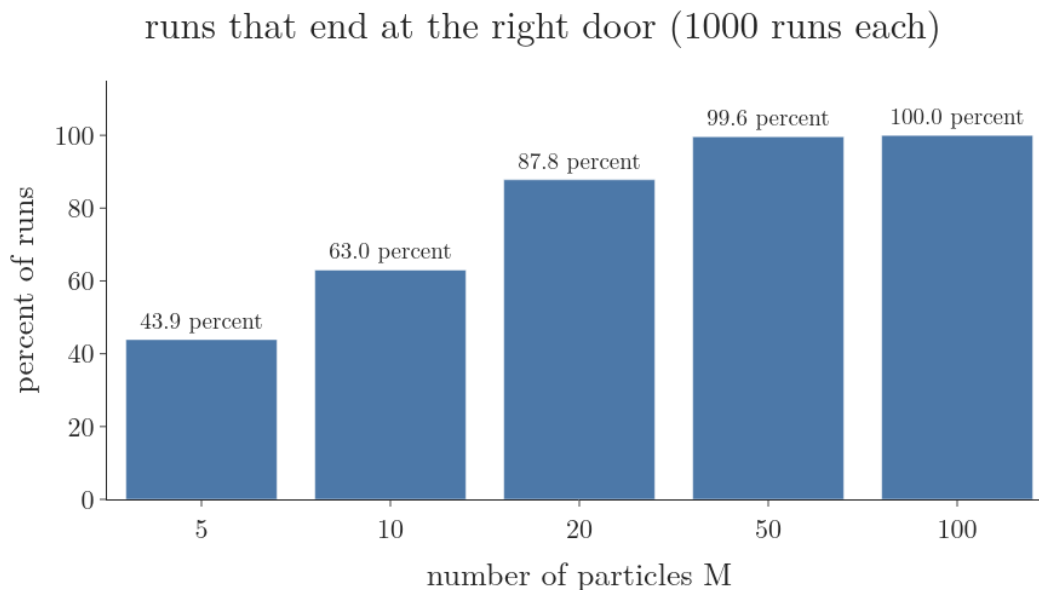
Figure 8: Share of 1000 runs that end at the right door: 43.9 percent with 5 particles, 63.0 with 10, 87.8 with 20, 99.6 with 50, 100 with 100
