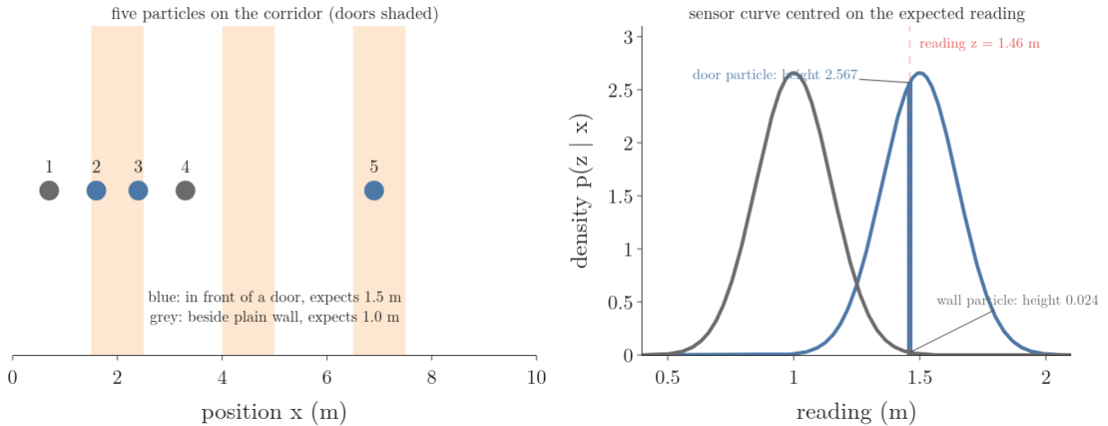
Figure 5: Left: five particles on the corridor, three at doors (blue) and two beside wall (grey). Right: the sensor's bell curve centred on 1.5 m for a door particle and on 1.0 m for a wall particle; at the reading 1.46 m the heights are 2.567 and 0.024
