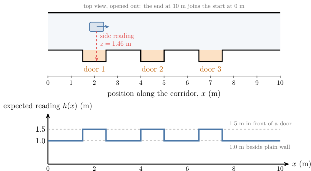
Figure 1: A corridor that loops round a block, opened out from 0 to 10 m, with three doors set back into the right-hand wall; the robot at 2.1 m reads 1.46 m to the side. Below: the map, the reading expected at each position
