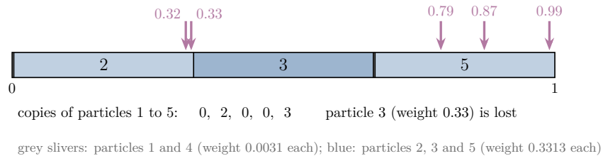
Figure 6: The five weights laid end to end from 0 to 1. Top: low-variance sampler with start 0.12 and pointers every 0.2 gives copies 0, 2, 1, 0, 2. Bottom: five independent random numbers give copies 0, 2, 0, 0, 3, and particle 3 is lost
