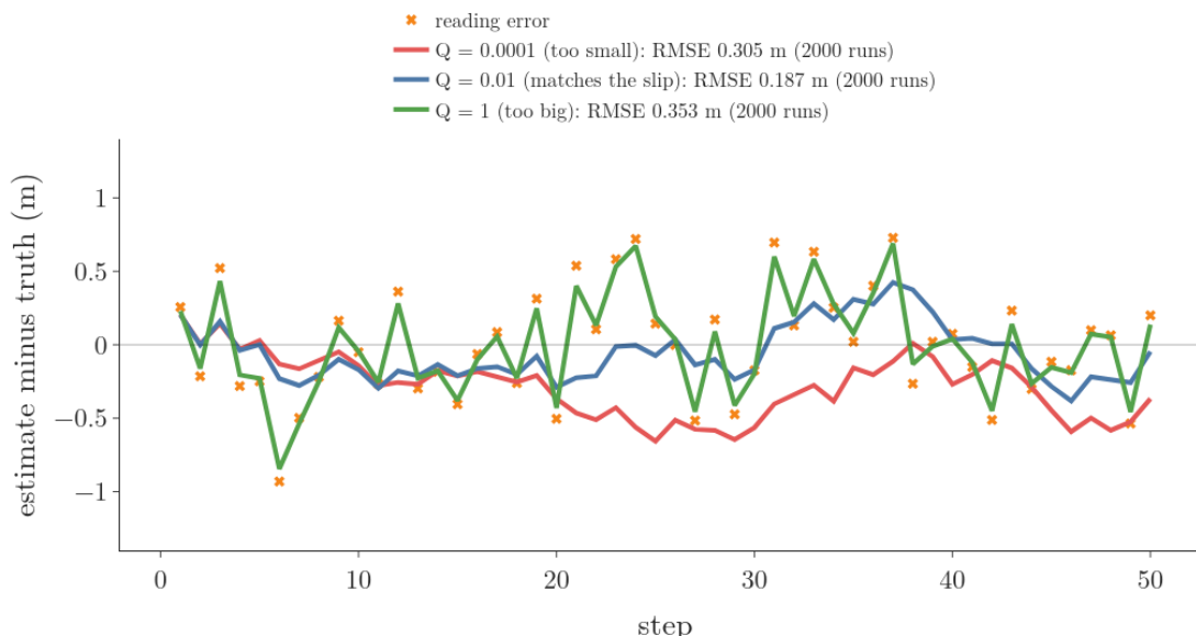
Figure 10: Error of three filters on one 50-step run; the legend gives each filter’s RMSE over all 2000 runs. Q = 0.0001 lags below the truth for long stretches; Q = 1 jumps with every reading; Q = 0.01 stays closest to zero
