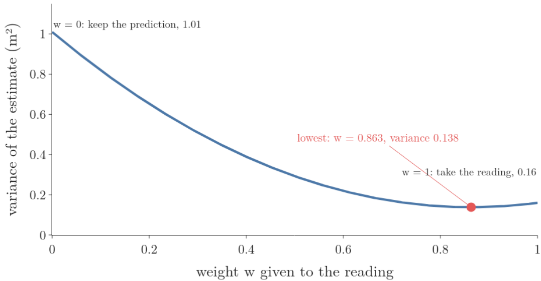
Figure 3: The variance of the blended estimate against the weight on the reading, for the first step: 1.01 at w = 0 , 0.16 at w = 1 , lowest at w = 0.863 with variance 0.138
