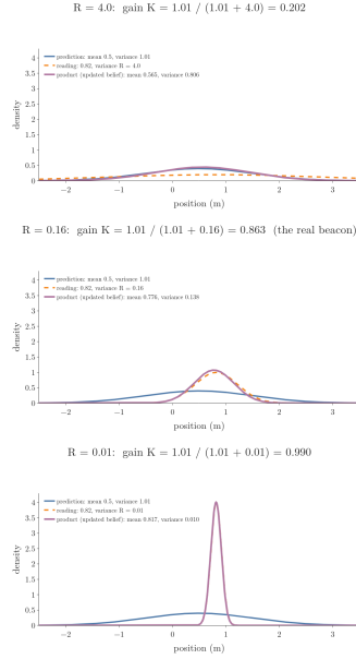
Figure 4: The step-1 prediction (mean 0.5, variance 1.01) multiplied by a reading at 0.82 whose variance R falls from 4 to 0.01: the product moves from the prediction to the reading and narrows; at R = 0.16 the product has mean 0.776 and variance 0.138
