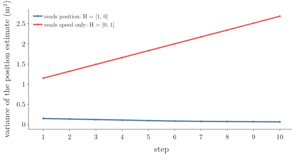
Figure 9: Variance of the position estimate over ten steps: with a position sensor it stays small and ends at 0.066; with only a speed sensor it grows steadily to 2.68
