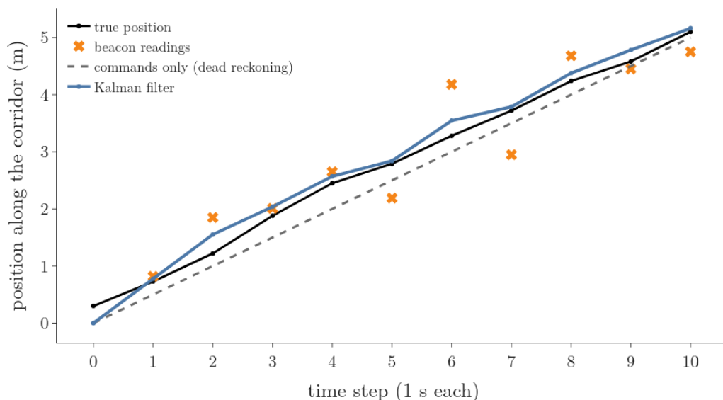
Figure 1: Ten steps of a robot in a corridor: the true position, the jumpy beacon readings, the drifting estimate from the commands alone, and the Kalman filter estimate that follows the truth
