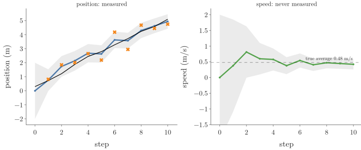
Figure 8: The two-variable filter fed only position readings. Left: position estimate, readings and truth with a band of two standard deviations. Right: the speed estimate, never measured, settles near the true average of 0.48 m/s while its band narrows
