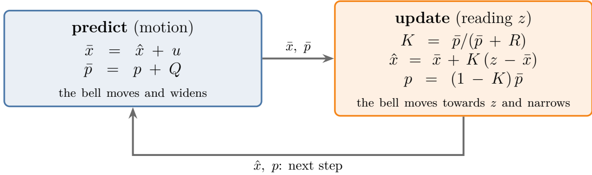
Figure 5: The one-dimensional Kalman filter as a loop: predict moves the mean by u and adds Q to the variance; update computes K , moves the mean a fraction K towards the reading and multiplies the variance by 1 - K
