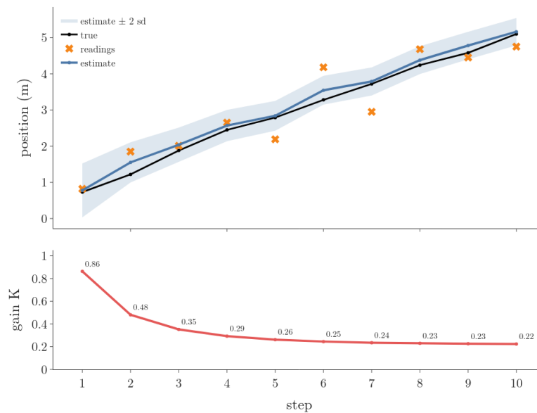
Figure 7: Top: true position, readings and the estimate with a band of two standard deviations. Bottom: the gain falls from 0.86 at step 1 to 0.22 at step 10
