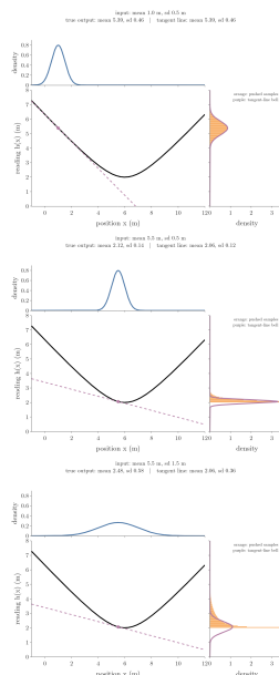
Figure 2: A bell of positions (top) pushed through the beacon curve (middle, black) gives the orange histogram of readings (right); the purple bell is what the tangent line at the mean predicts. Far from the beacon (mean 1 m) the two agree; near it (mean 5.5 m) the true readings are lopsided against 2 m, and with a wide input (sd 1.5 m) the tangent bell is far too narrow
