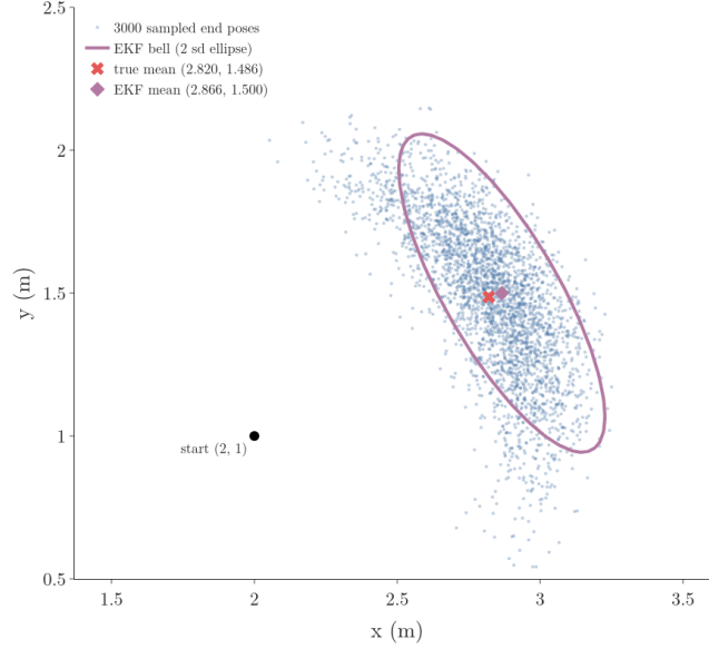
Figure 3: 3000 sampled end poses after driving 1 m from (2, 1, 30 degrees) with a heading spread of 0.3 rad form a curved banana; the EKF's ellipse of two standard deviations from G P G-transpose covers it roughly, with its mean 0.04 m ahead
