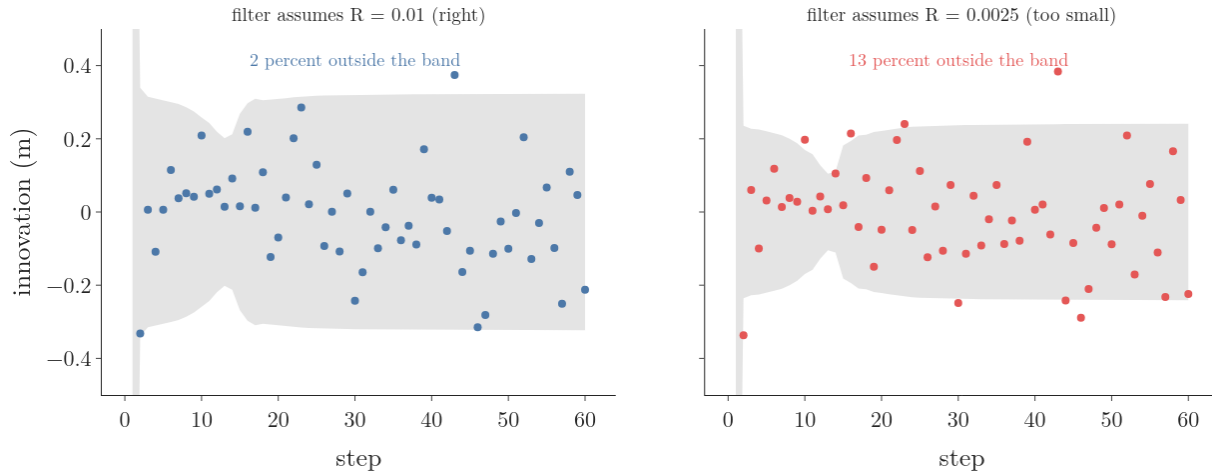
Figure 6: Innovations of one 60-step run with the band of two predicted standard deviations: with R = 0.01 2 percent fall outside; with R = 0.0025 the band is half as wide and 13 percent fall outside
