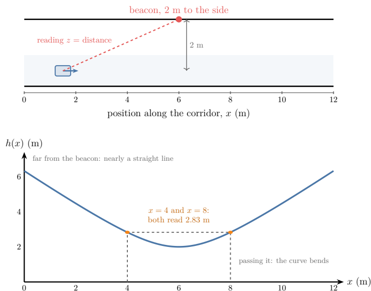
Figure 1: Top: a radio beacon on the corridor wall at 6 m, 2 m to the side; the robot reads its straight-line distance to it. Bottom: that distance as a function of position, a curve with its lowest point at 2 m under the beacon; positions 4 m and 8 m both read 2.83 m
