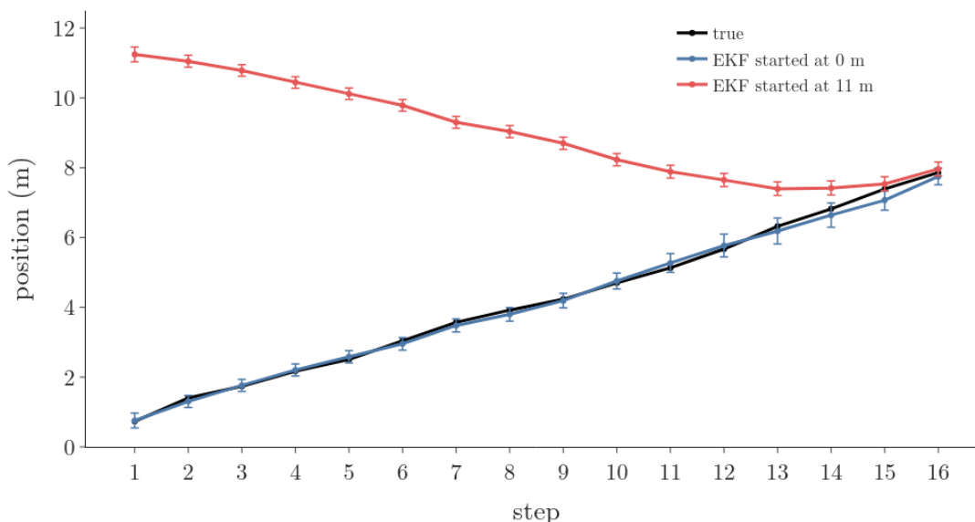
Figure 5: The same 16 readings fed to an EKF started at 0 m (follows the truth) and one started at 11 m (follows the mirror path, wrong by up to 10.5 m with narrow error bars, until the robot passes the beacon at 6 m)
