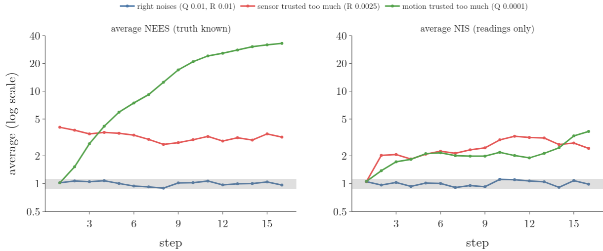
Figure 7: Average NEES (left) and NIS (right) over 500 runs, per step, log scale. The filter with the right noises stays in the grey band around 1; trusting the sensor too much sits near 3; trusting the motion too much makes NEES climb past 30
