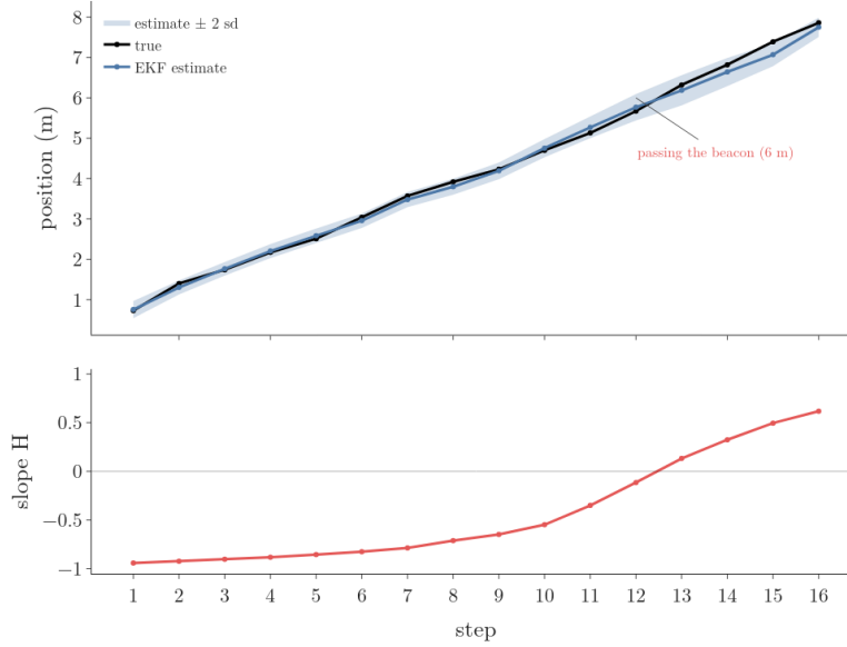
Figure 4: Top: the EKF estimate follows the truth for 16 steps, with a band of two standard deviations that widens as the robot passes the beacon. Bottom: the slope H of the distance rises from -0.94 through 0 at the beacon to +0.62
