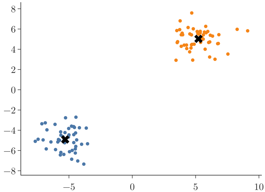
2 blobs, k = 2
