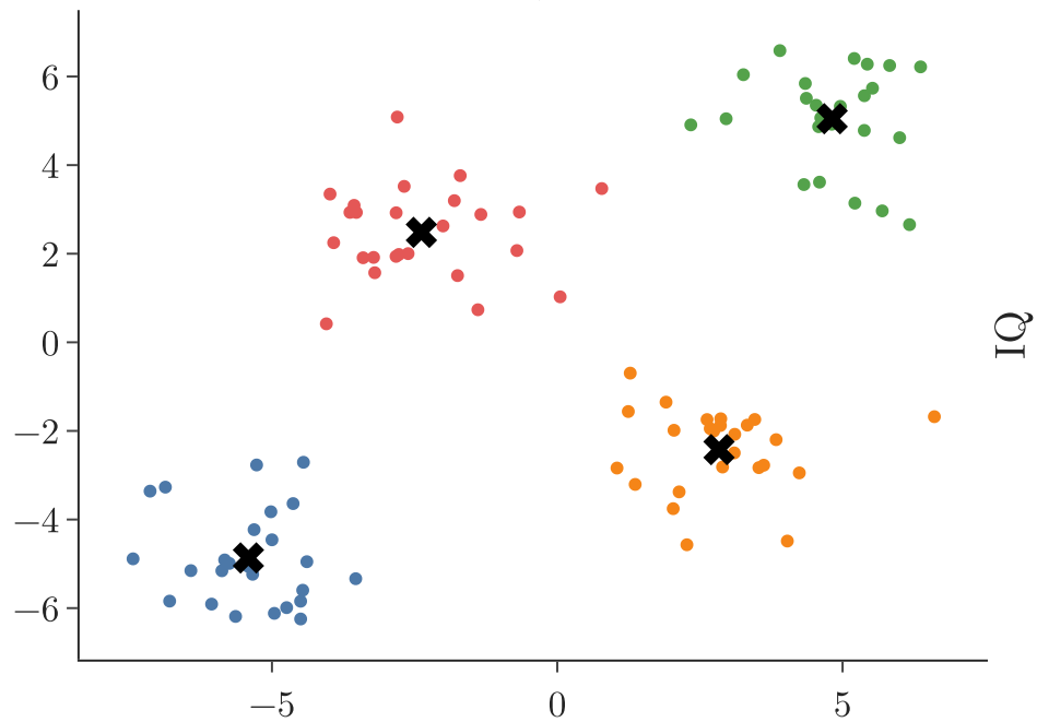
4 blobs, k = 4
