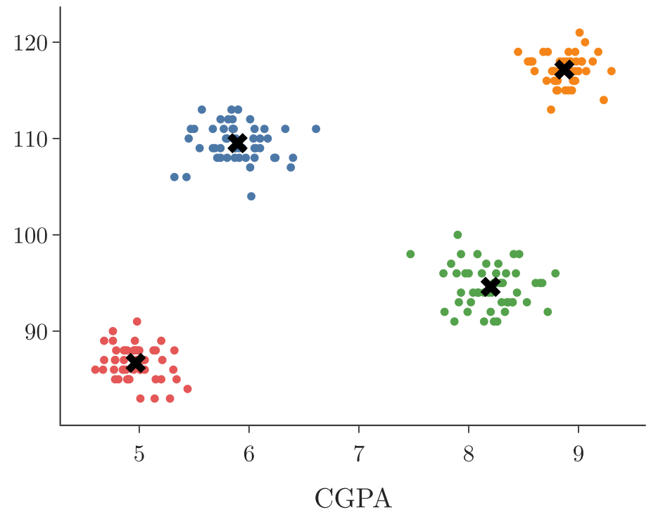
students, k = 4
