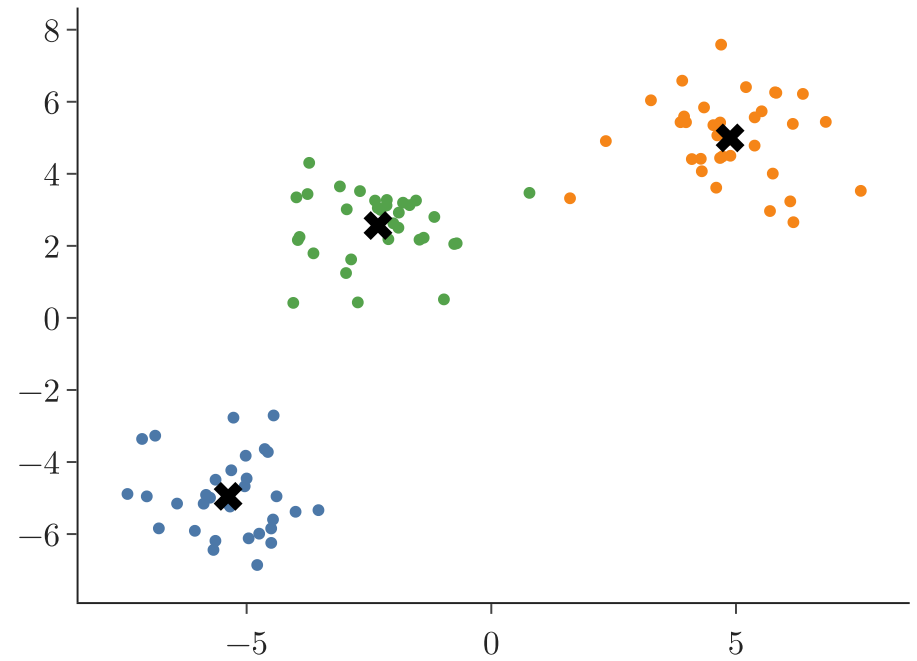
3 blobs, k = 3
