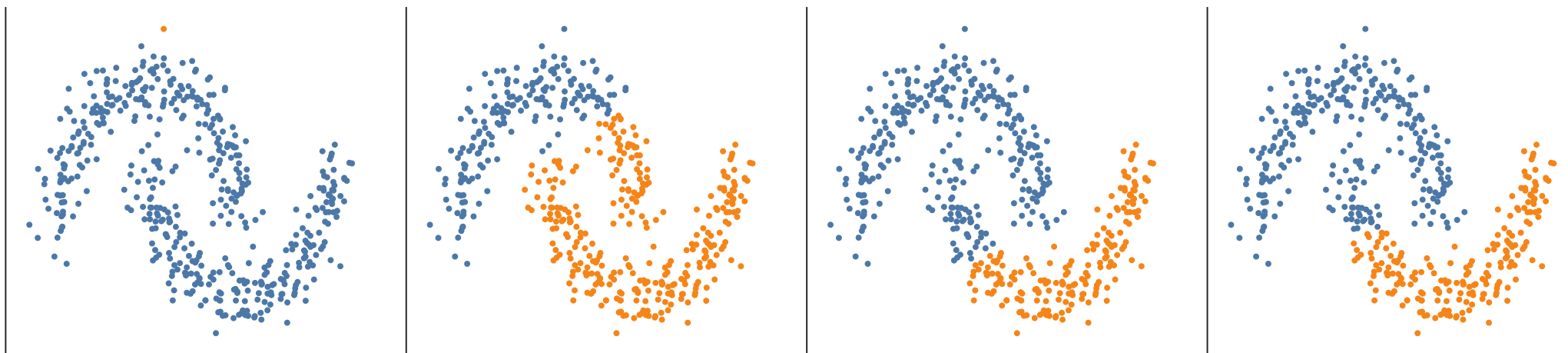
moons, noisy
