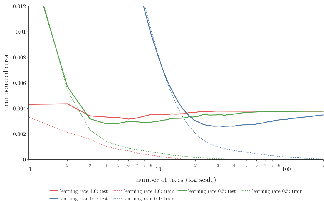
Figure 5: Training error (dotted) and test error (solid) after each tree, for learning rates 1, 0.5 and 0.1
