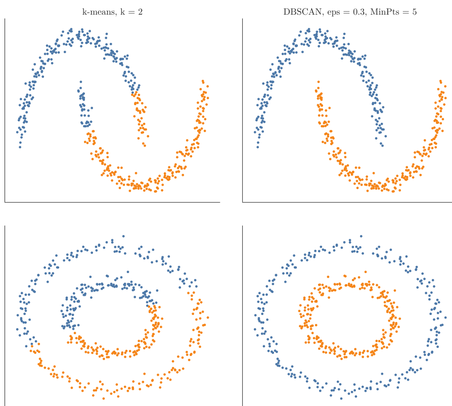
Figure 1: k-means (left) and DBSCAN (right) on two moons and two circles
