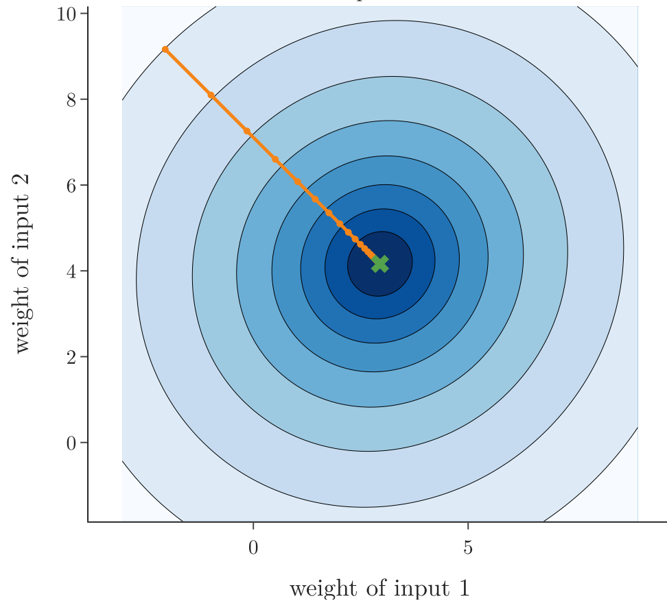
Standardised inputs: round contours
