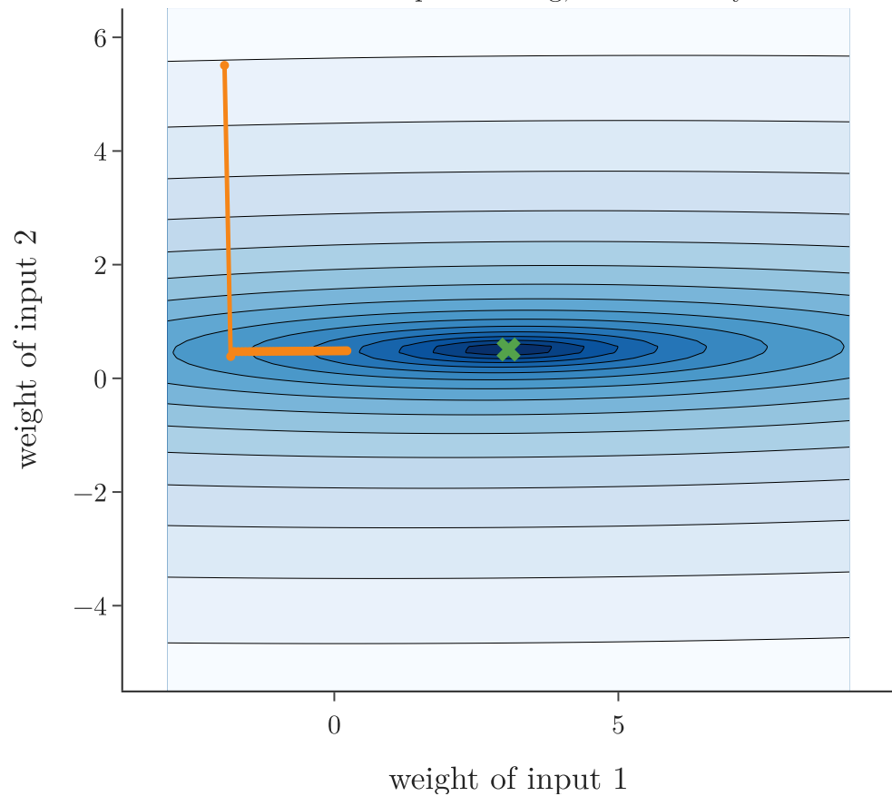
Unscaled inputs: a long, narrow valley
