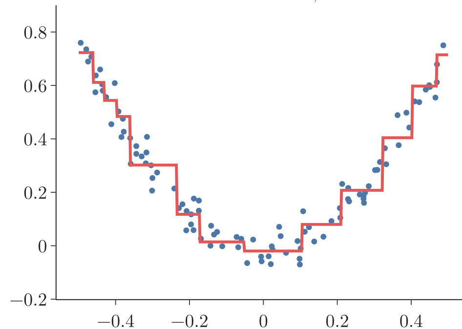
2 trees: train MSE 0.0021, test 0.0044
