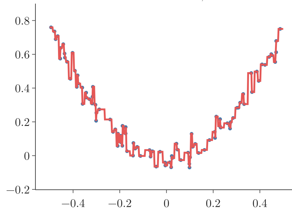
50 trees: train MSE 0.0000, test 0.0038
