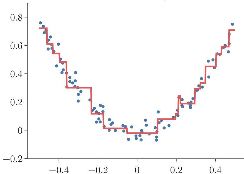
3 trees: train MSE 0.0016, test 0.0034
