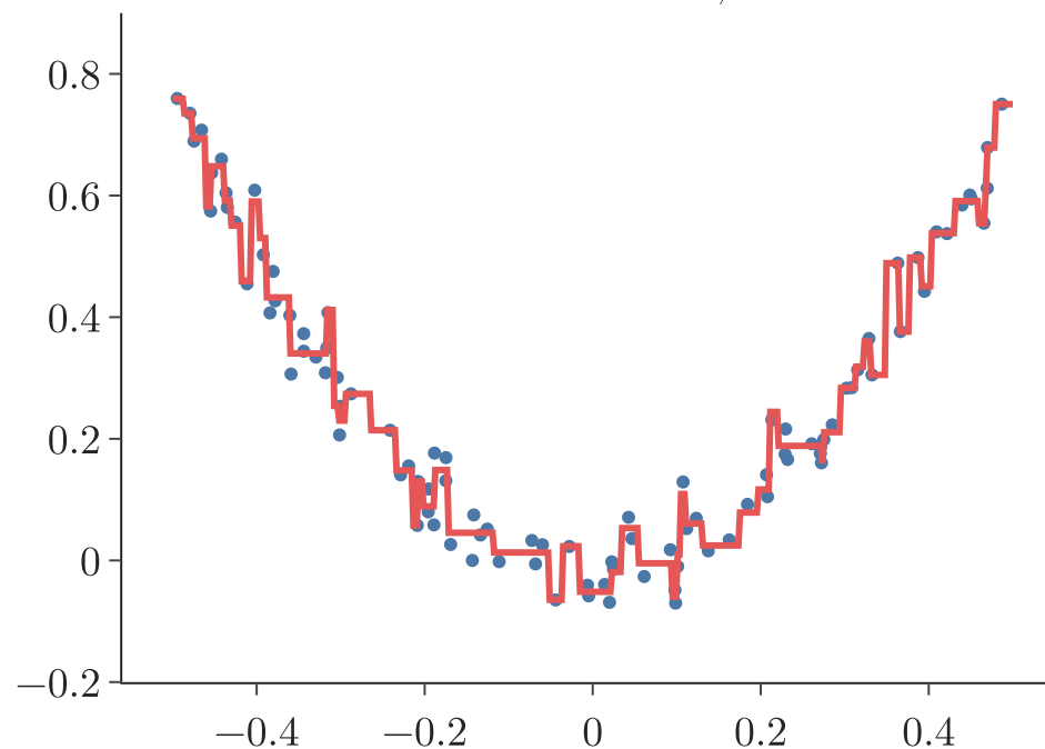
10 trees: train MSE 0.0003, test 0.0035
