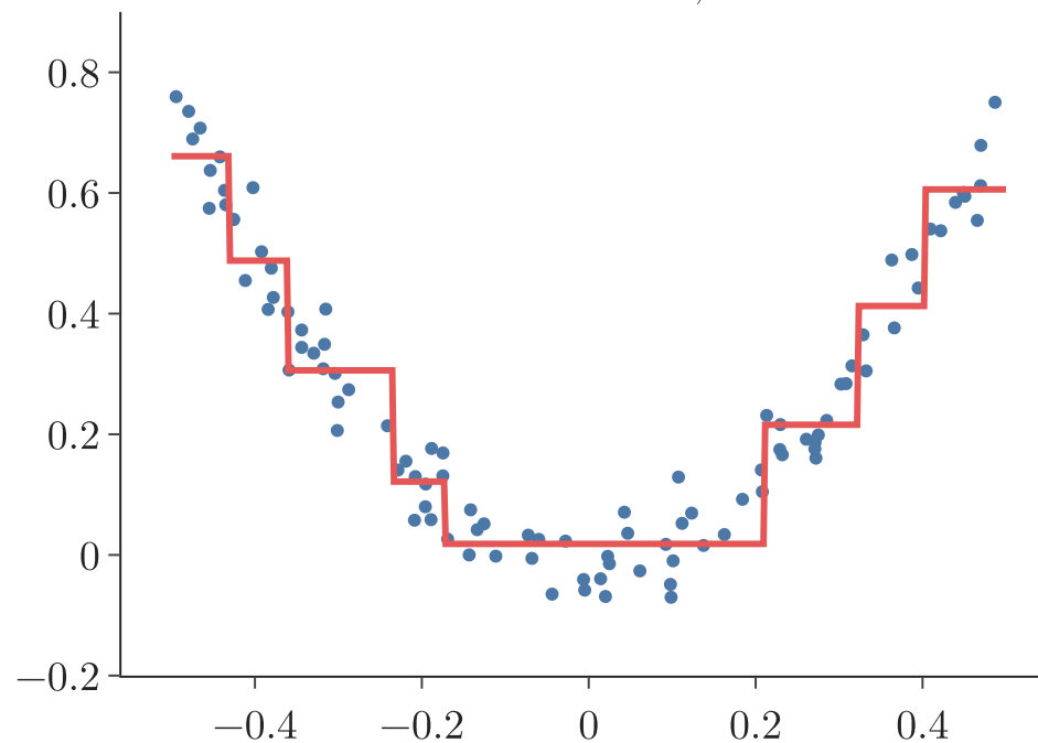
1 tree: train MSE 0.0033, test 0.0043
