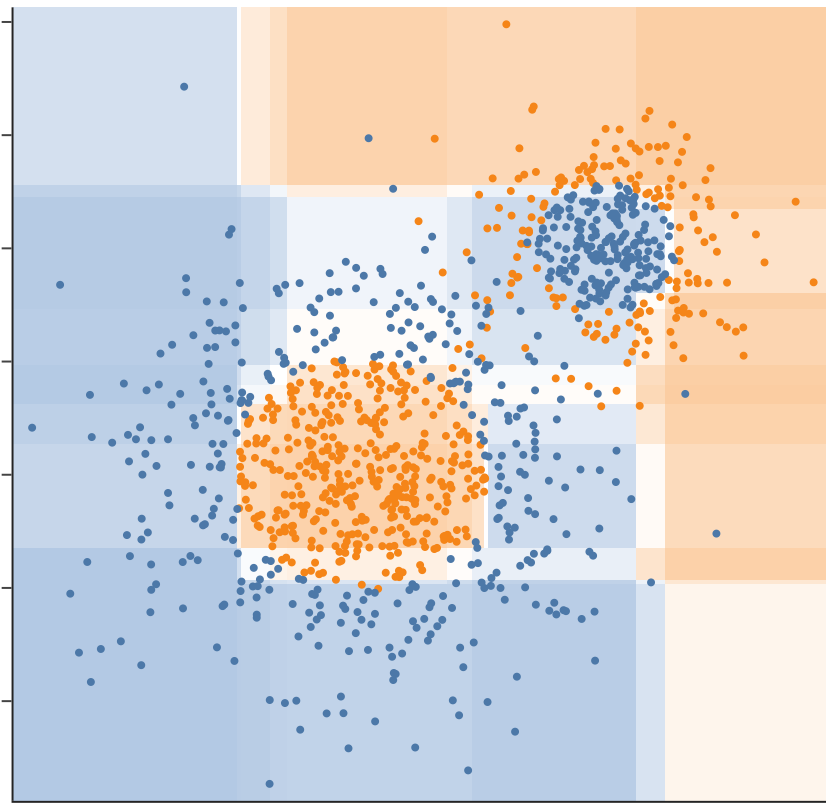
10 trees: train 0.89, test 0.84
