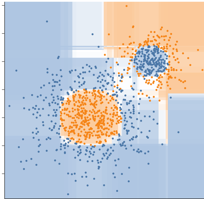
30 trees: train 0.95, test 0.90
