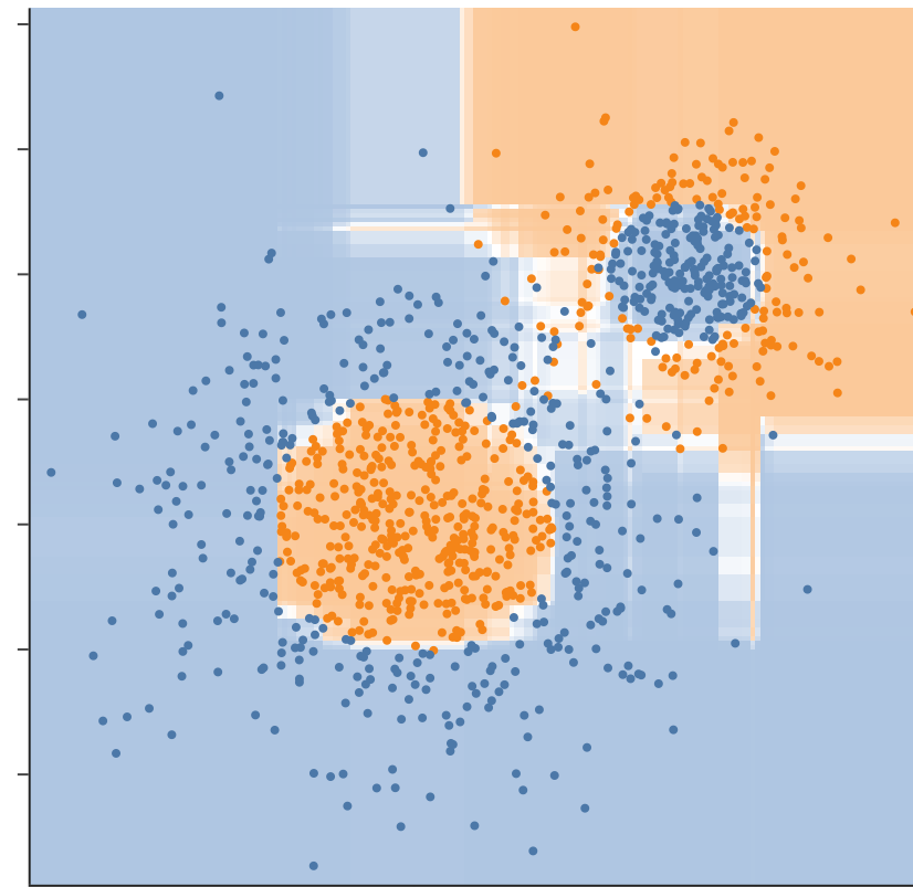
100 trees: train 0.99, test 0.93
