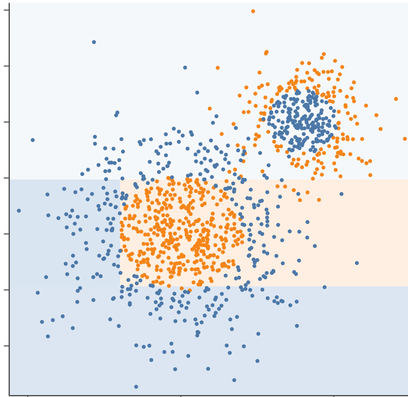
1 tree: train 0.76, test 0.69
