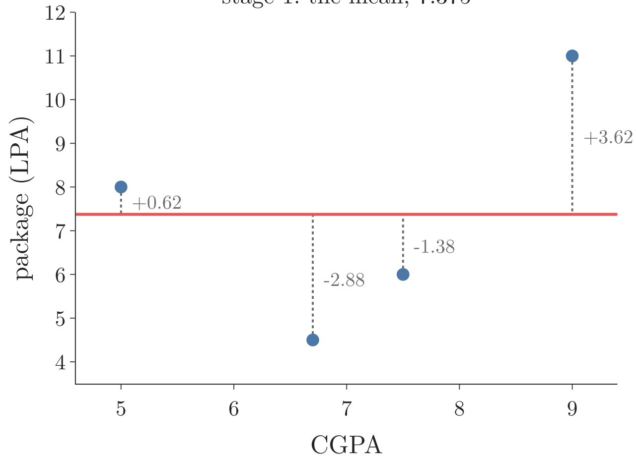
stage 1: the mean, 7.375
