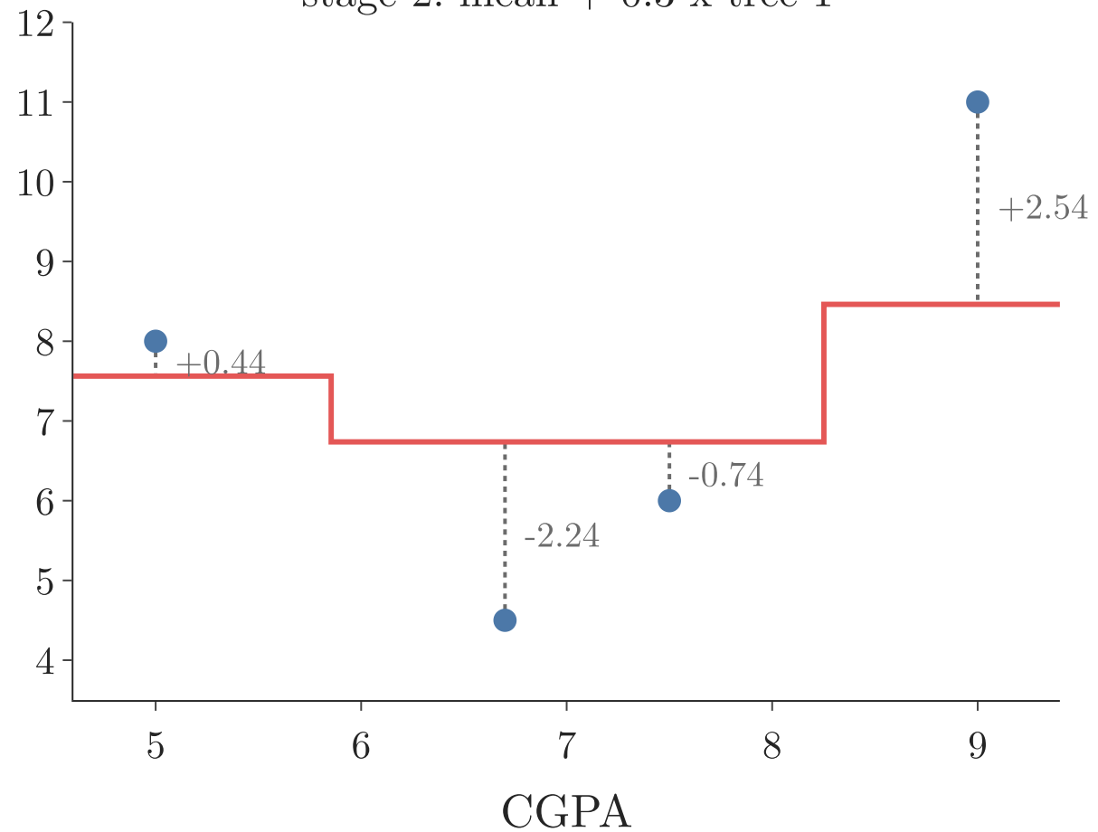
stage 2: mean + 0.3 x tree 1
