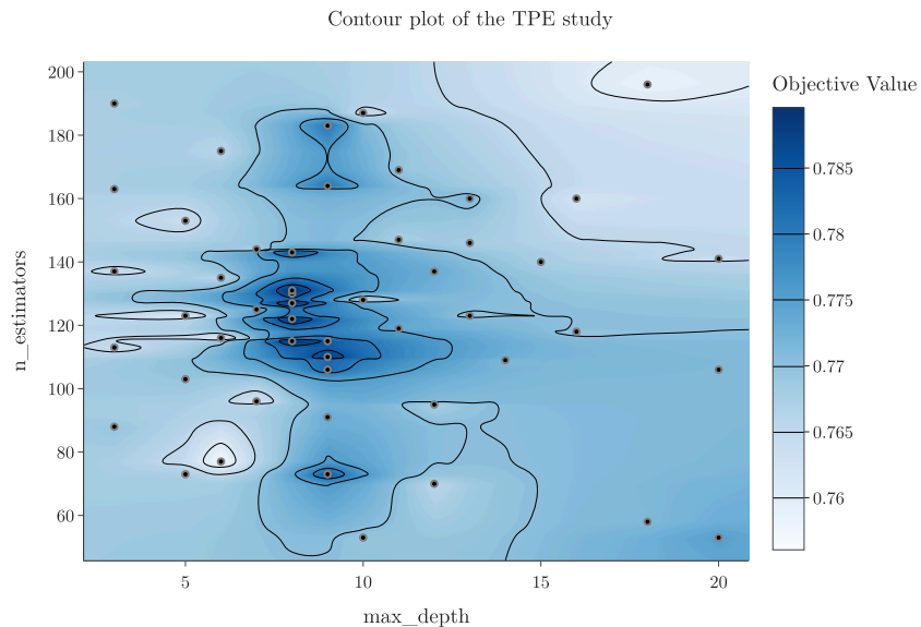
Figure 5: Contour plot of the TPE study: max_depth against n_estimators , darker is a higher score; dots are trials
