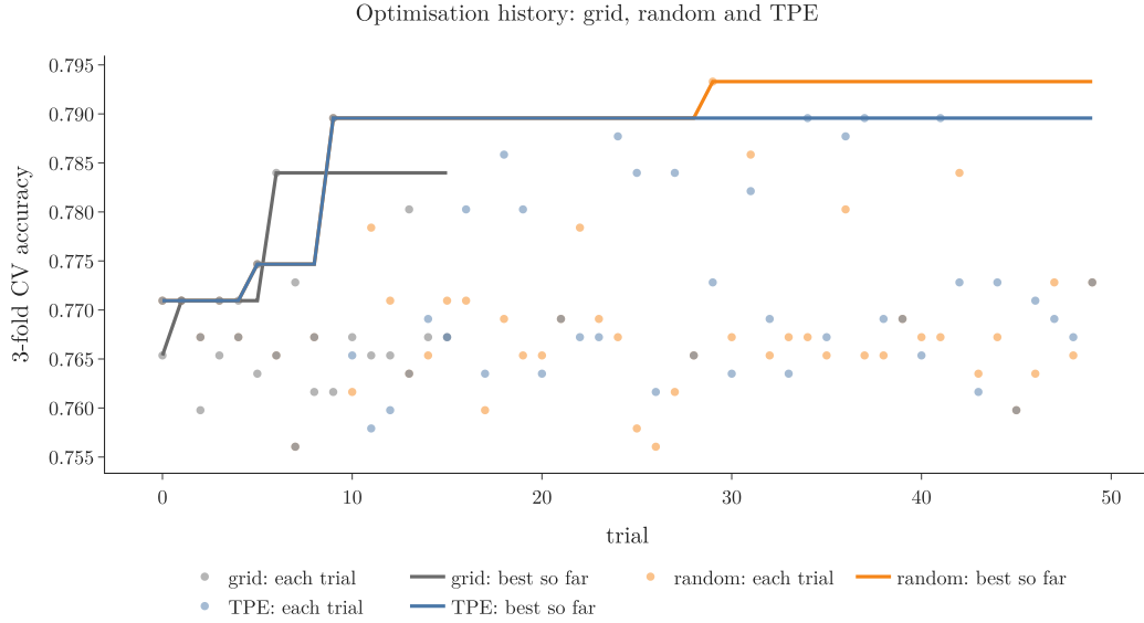
Figure 3: Optimisation history of the three studies: each trial (dots) and the best so far (lines)
