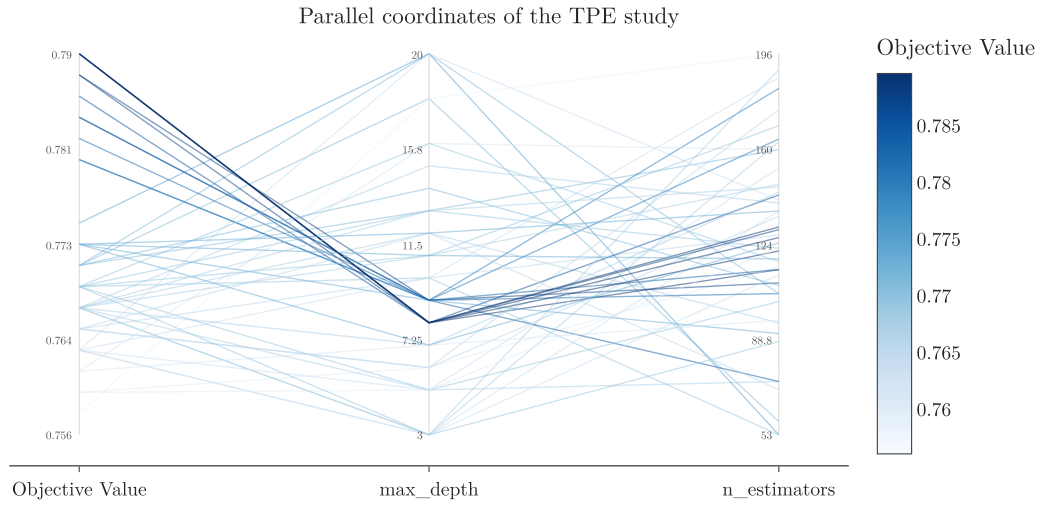
Figure 4: Parallel coordinates of the TPE study: each line is a trial, darker is a higher score
