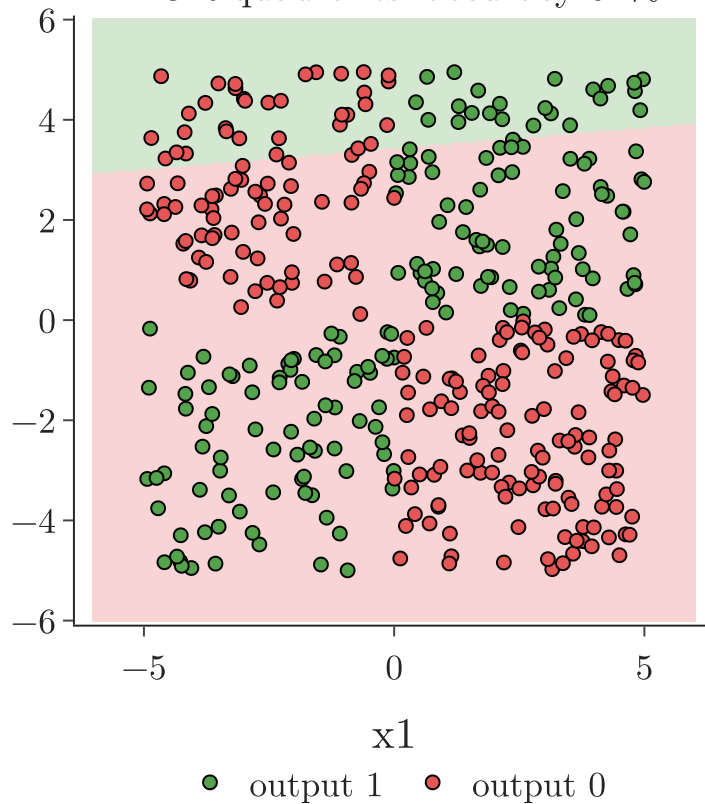
XOR quadrants: accuracy 52%
