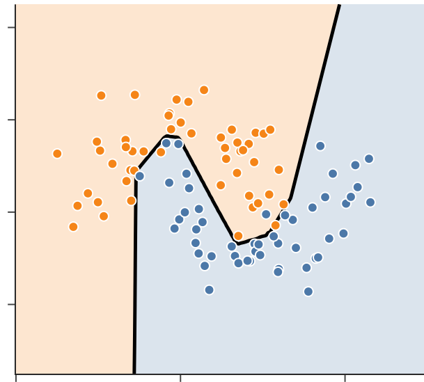
L1, \lambda = 0.001
