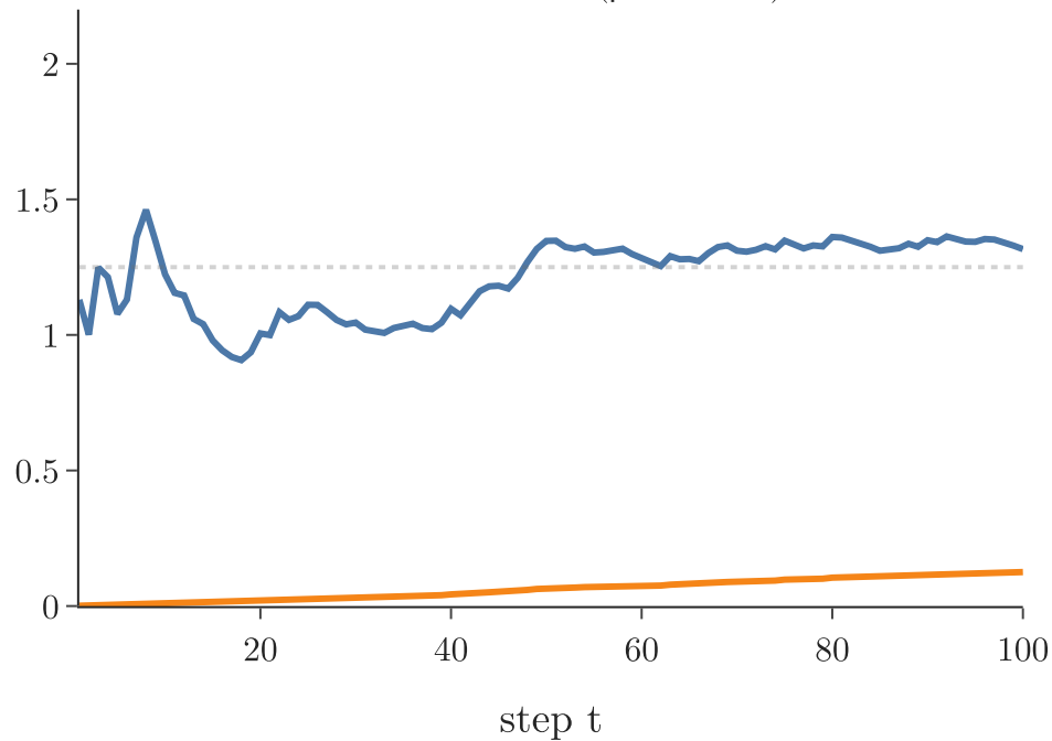
second moment v ( \beta_2 = 0.999 )
