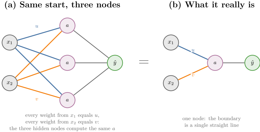
Figure 2: (a) After a start where all weights are equal, every weight leaving x_1 has one value u and every weight leaving x_2 one value v , so the hidden nodes all compute the same a . (b) The network behaves like a single hidden node
