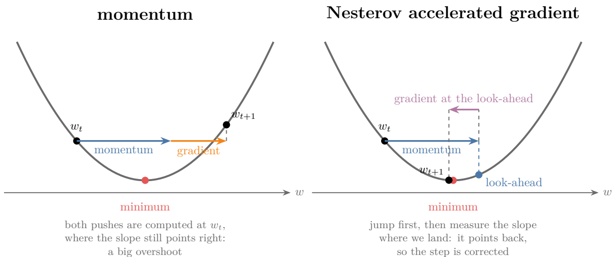
Figure 2: One step near the minimum. Left, momentum: the momentum jump and the gradient step are both computed at w_t , where the slope still points right, so the step overshoots. Right, NAG: jump first, then measure the slope at the look-ahead point, which points back, so the step is corrected
