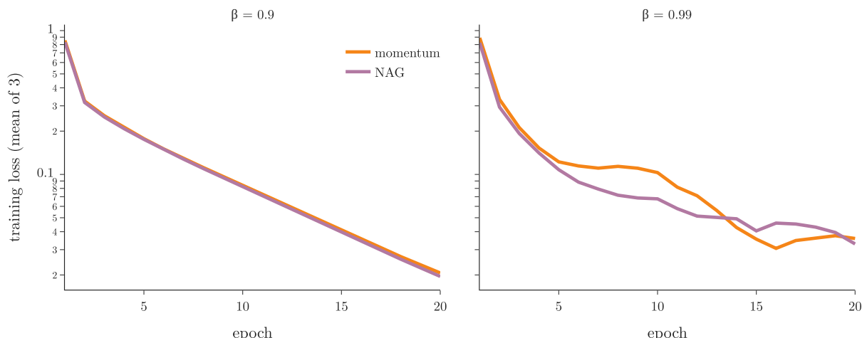
Figure 4: Training loss on MNIST per epoch, mean of 3 seeds. Left: \beta = 0.9 , the two curves overlap. Right: \beta = 0.99 , NAG (purple) mostly below momentum (orange)
