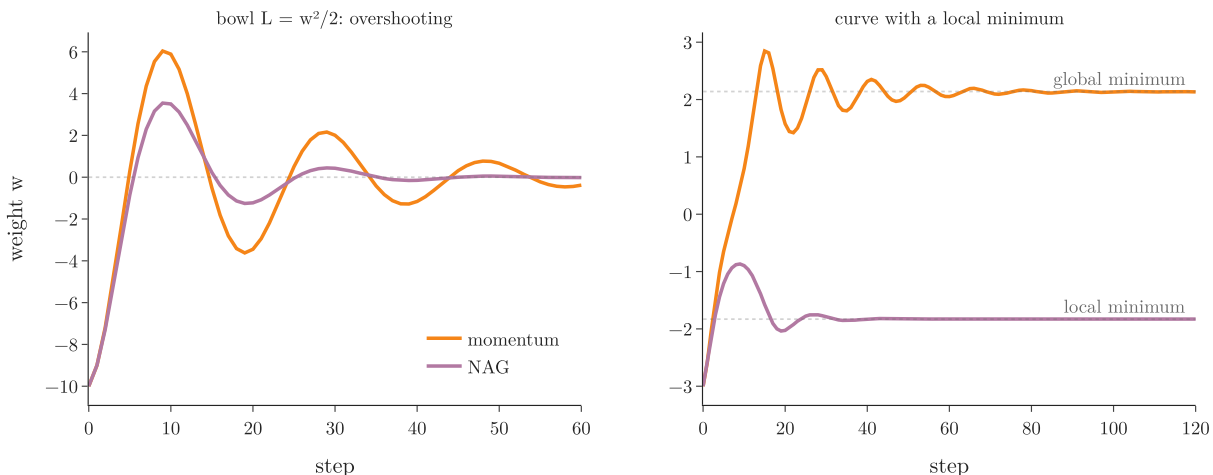
Figure 3: The weight over the steps. Left: the bowl L = w^2/2 from w = -10 , \eta = 0.1 , \beta = 0.9 ; NAG (purple) swings less far past the minimum and settles sooner than momentum (orange). Right: a curve with a local minimum from w = -3 , \eta = 0.05 , \beta = 0.9 ; momentum rolls on to the global minimum, NAG stays in the local one
