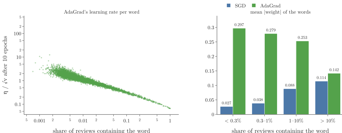
Figure 3: IMDB, 5,000 words. Left: AdaGrad’s learning rate for each word after 10 epochs against the share of reviews containing the word; the rarer the word, the larger its learning rate. Right: mean size of the learned weights per frequency band; with SGD the rare words barely move
