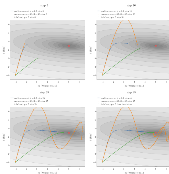
Figure 1: Gradient descent, momentum and AdaGrad on a loss stretched by a sparse feature. Gradient descent and momentum first move along b , then crawl along m ; AdaGrad heads for the minimum
