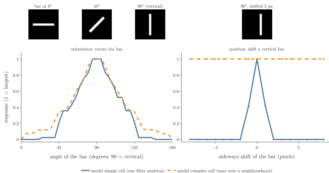
Figure 3: A model simple cell (one filter position, blue) and a model complex cell (maximum over a neighbourhood, orange). Left: both are tuned to orientation, strongest for a vertical bar and silent for a horizontal one. Right: shifting the vertical bar sideways by 2 pixels silences the simple cell, while the complex cell keeps responding
