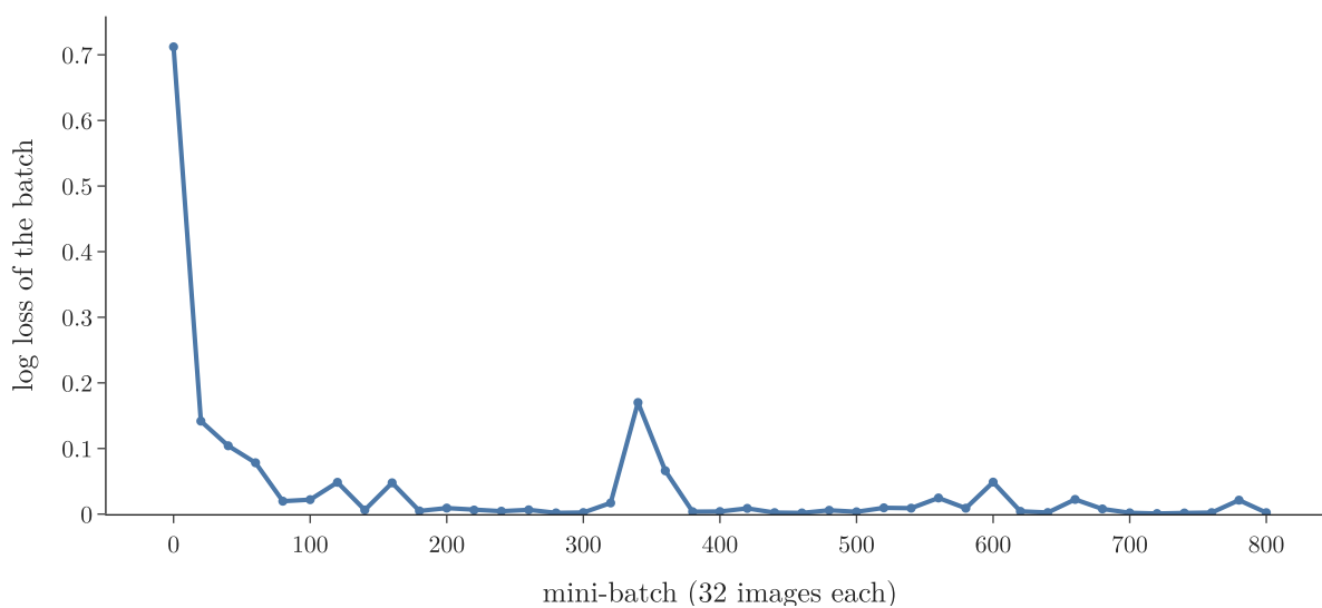
Figure 3: The loss of the batch while training with the hand-derived gradients; it drops from 0.71 to near 0 within the first few hundred mini-batches
