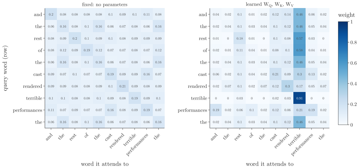
Figure 4: Attention weights on a real review. Left: without parameters, each word borrows mostly from itself and spreads the rest evenly. Right: with learned W_Q, W_K, W_V , almost every word borrows most from “terrible”, the word that decides the sentiment
