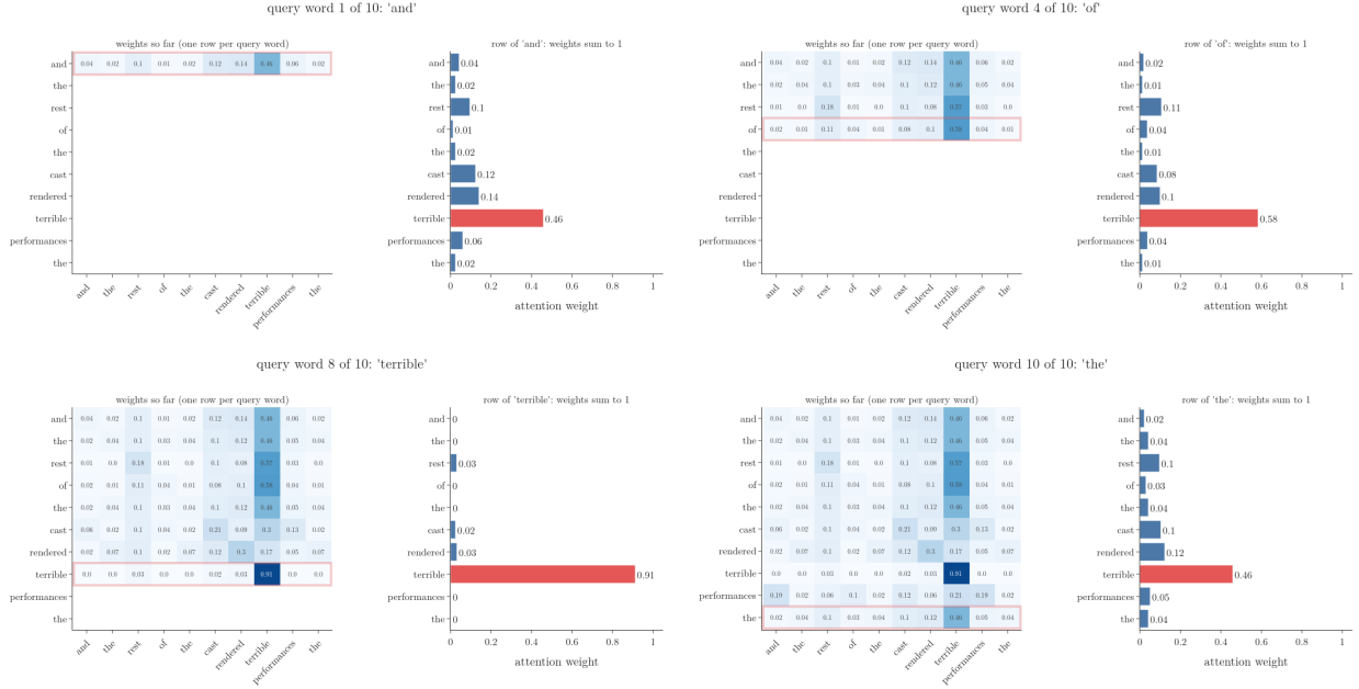
Figure 5: The learned weights forming one query word at a time. Left: the weight matrix filling row by row. Right: the current query word’s weights, which sum to 1; the largest is red
