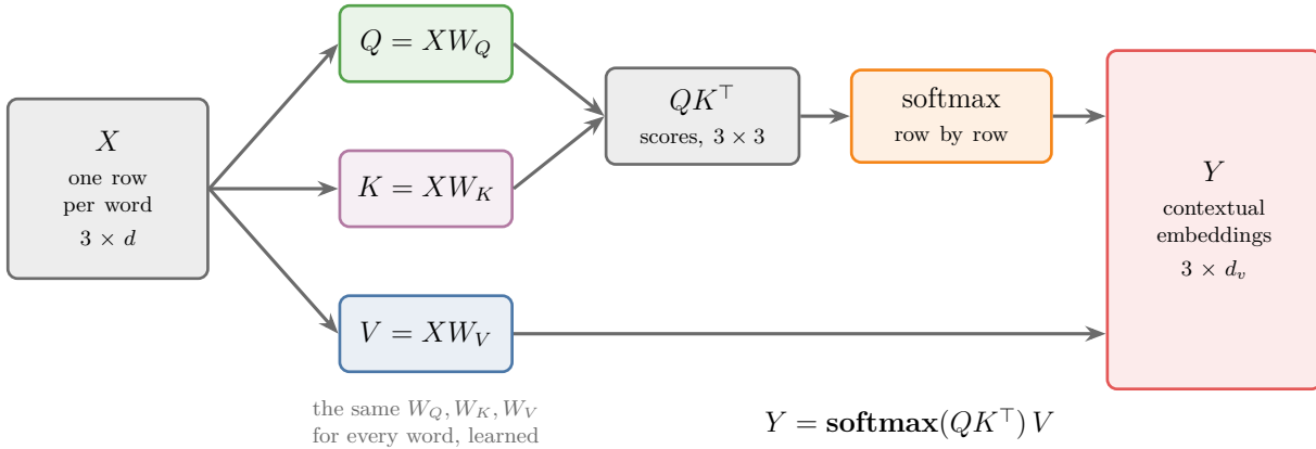
Figure 3: Self-attention with learned matrices, for a whole sentence at once
