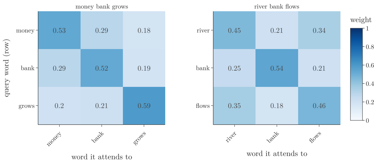
Figure 2: The weights of the simple self-attention for both phrases, with real embeddings. Row i shows how word i mixes the words of its phrase; every row sums to 1
