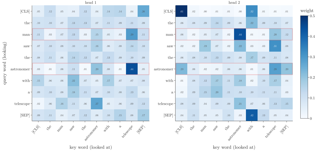
Figure 2: Heads 1 and 2 of BERT-base’s first layer. Each row is a query word, and its 10 weights sum to 1. Outlined: the rows of “man” and “astronomer”
