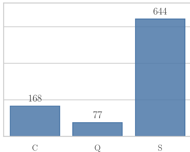
Embarked
