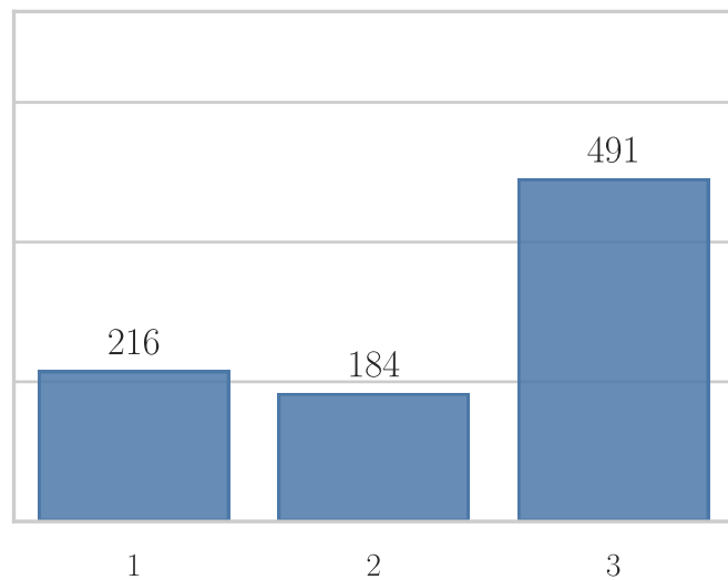
Pclass
