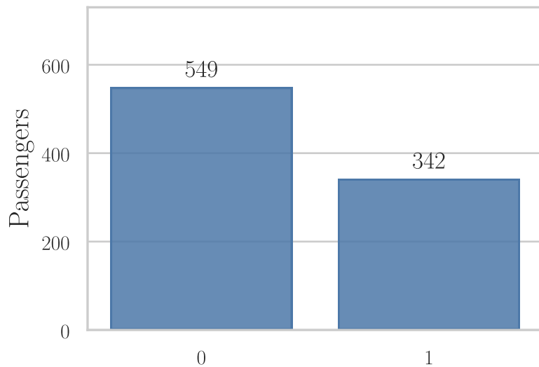
Survived
