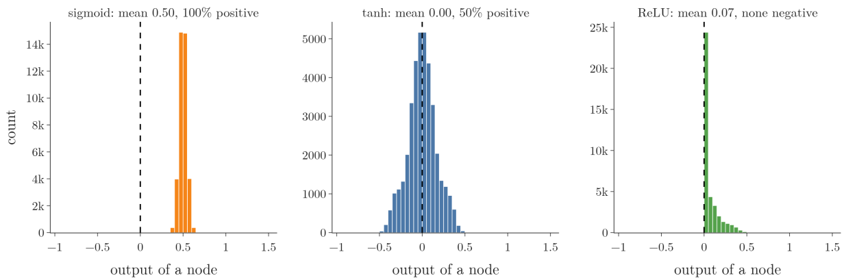
Figure 5: The outputs of one freshly initialised 128-node layer for the 300 circles observations, with three activations: 38,400 values each. Dashed line: 0.
