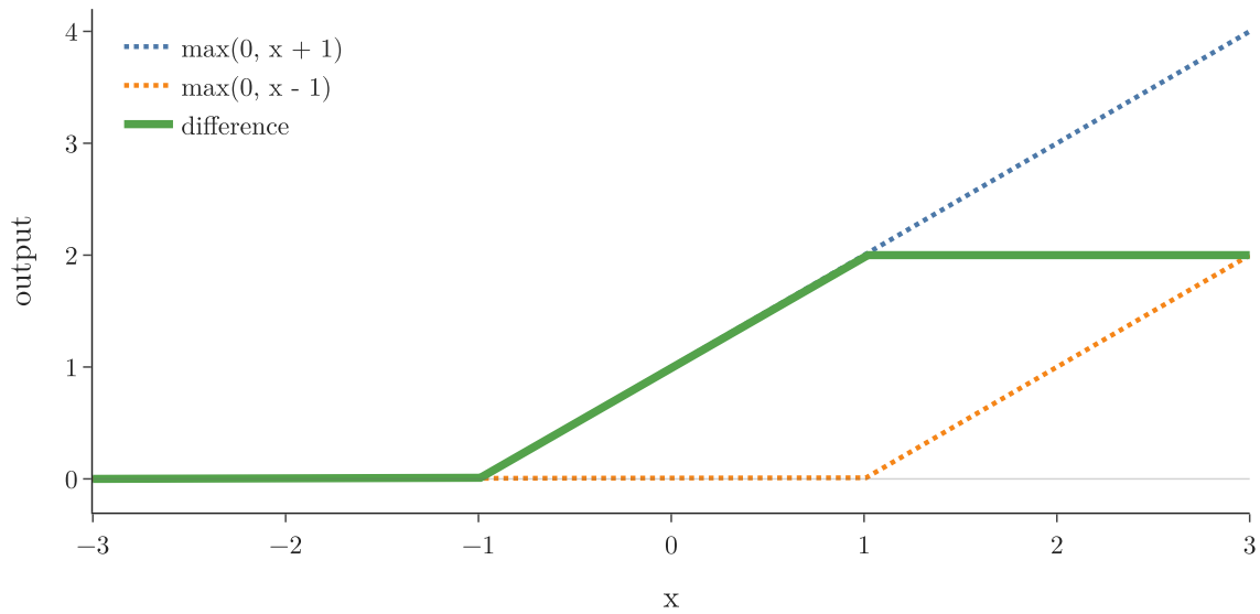
Figure 6: Two ReLUs (dotted) and their difference (green): flat, rising, flat. No straight line has two corners
