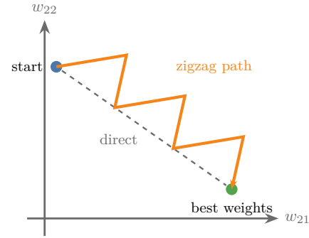
Figure 4: (a) With all-positive inputs, one update moves every weight into a node the same way: only the green quadrants are possible. (b) When the best weights need one weight up and the other down, gradient descent has to zigzag
