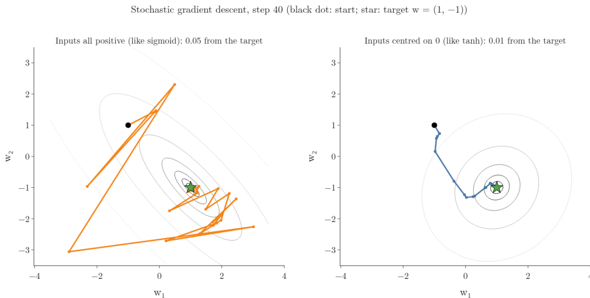
Figure 3: Stochastic gradient descent on one node with two weights. Left: inputs all positive. Right: the same inputs centred on 0. Grey: contours of the loss; black dot: start; star: the target weights.
