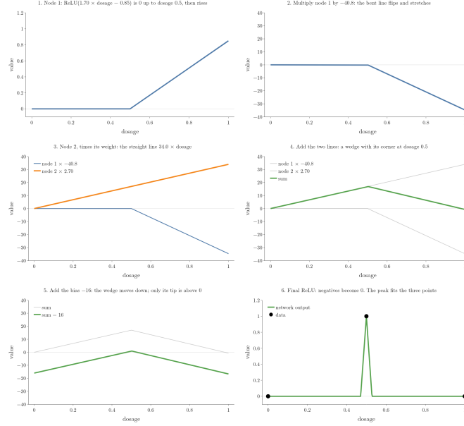
Figure 7: Two ReLU nodes fitting three points, one operation per frame: the bent line of node 1, its output weight, the straight line of node 2, their sum, the bias, the final ReLU. Numbers after StatQuest, “Neural Networks Pt. 3: ReLU In Action!!!”
