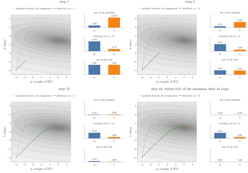
Figure 3: AdaGrad, \eta = 2 , on the students data, step by step. Left: its path (green) beside gradient descent's (grey). Right, for m (blue) and b (orange): the size of the gradient, the learning rate \eta/\sqrt{v} and the size of the update
