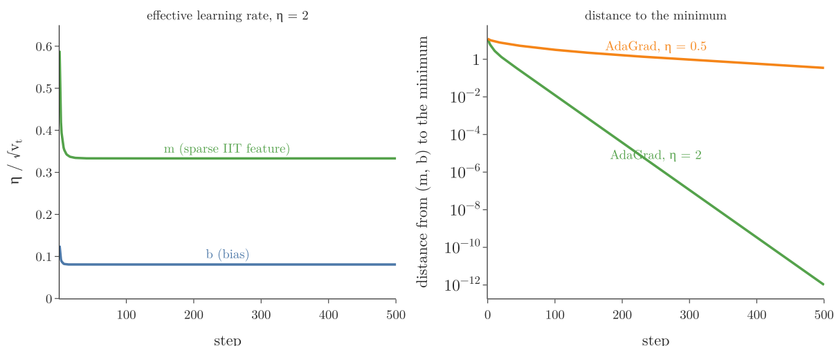
Figure 5: AdaGrad on the students data. Left: the effective learning rates of m and b with \eta = 2 fall in the first steps and never rise again. Right: distance to the minimum; with \eta = 2 AdaGrad converges, with \eta = 0.5 it is still 0.35 away after 500 steps
