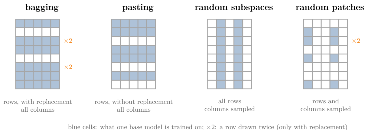
Figure 7: What one base model sees under each type: blue cells are the rows (observations) and columns (features) it is trained on
