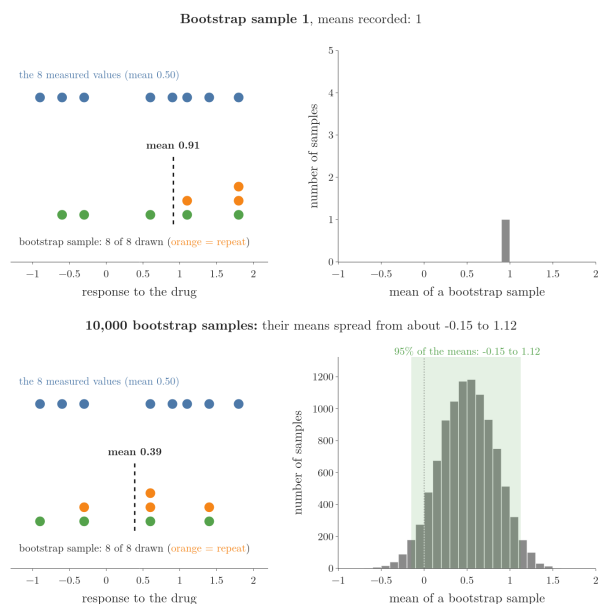
Figure 3: Bootstrapping the mean of 8 drug responses (example data). Left: the 8 measured values (blue) and one bootstrap sample drawn from them (green: first draw of a value; orange: a repeat). Right: the means of the bootstrap samples so far. Idea after StatQuest, “Bootstrapping Main Ideas!!!”.
