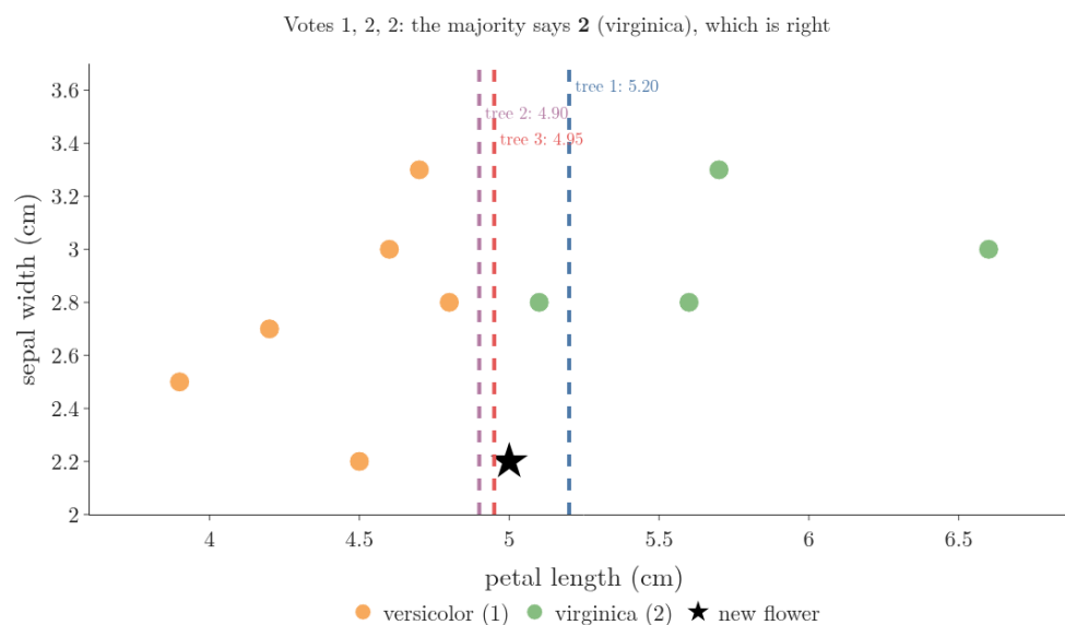
Figure 6: Bagging by hand. Each frame shows one tree's bootstrap sample (bigger dots are drawn more often, hollow dots are not drawn) and its cut on petal length; the last frame shows all three cuts and the vote on the new flower (star).
