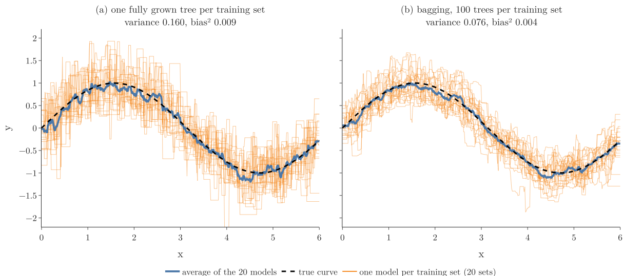
Figure 4: The same experiment repeated on 20 different training sets: (a) a single fully grown tree, (b) bagging with 100 trees. The spread of the orange curves is the variance
