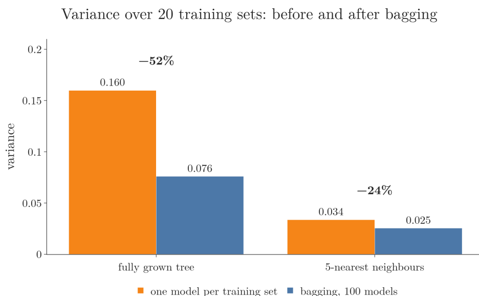
Figure 5: Variance over the 20 training sets of Figure 4, for one model per set (orange) and for bagging with 100 models per set (blue).
