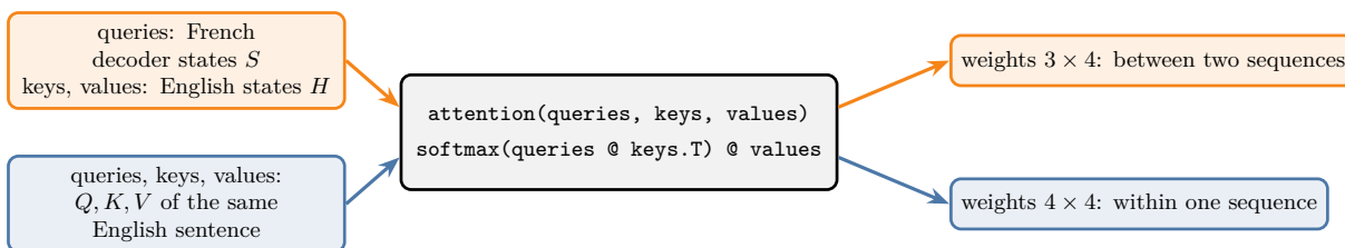
Figure 5: One function, two calls. Fed the French decoder states as queries and the English states as keys and values, it relates two sequences; fed the queries, keys and values of one sentence, it relates the sentence to itself
