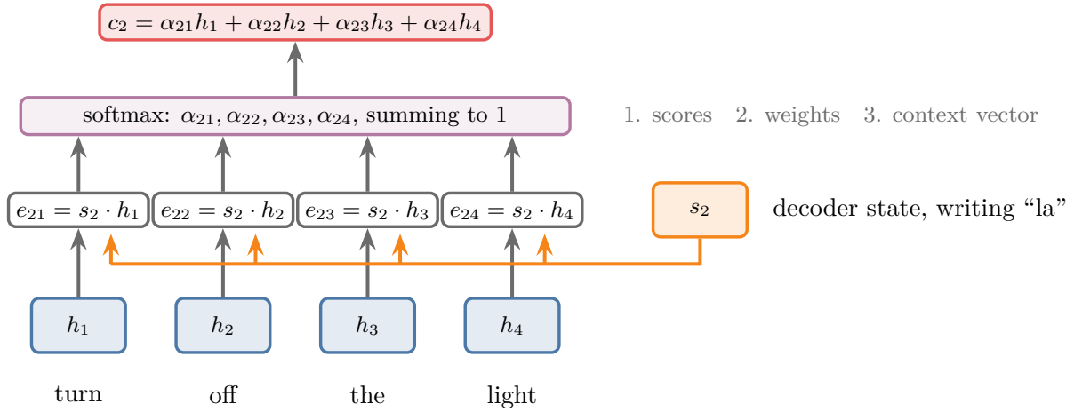
Figure 2: The three equations for decoder step 2, writing “la”. The decoder state s_2 (orange) is compared with every encoder state by a dot product; the softmax turns the four scores into weights; the weights mix the encoder states into c_2
