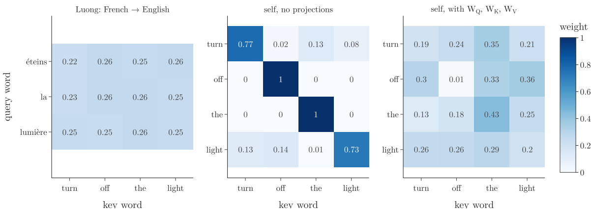
Figure 6: Weight matrices from the Notebook (untrained networks, so the values have no meaning yet; the shapes do). Left: Luong attention, French queries over English keys, 3 \times 4 . Middle: self-attention on the English embeddings without projections. Right: with W_Q , W_K , W_V and scaling. Both self-attention matrices are 4 \times 4
