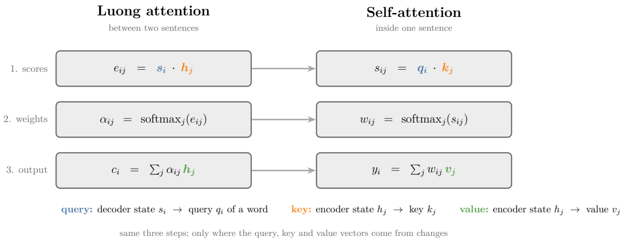
Figure 3: The three equations of Luong attention (left) and of self-attention (right), step by step. The colours mark the only substitutions: the decoder state becomes a query (blue), the encoder state used for comparing becomes a key (orange), and the encoder state that is mixed becomes a value (green)
