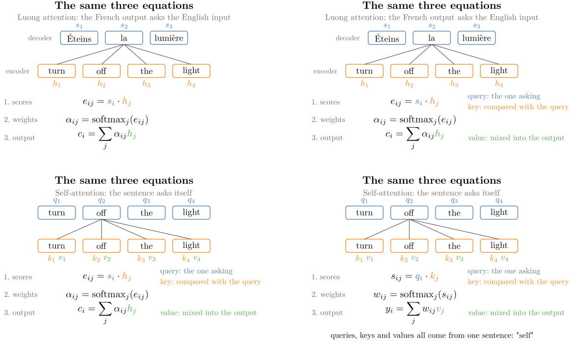
Figure 4: Luong attention turning into self-attention. The French row leaves, the English sentence takes its place and asks itself, and in each equation the decoder state becomes a query (blue), the encoder state becomes a key (orange) where it is compared and a value (green) where it is mixed
