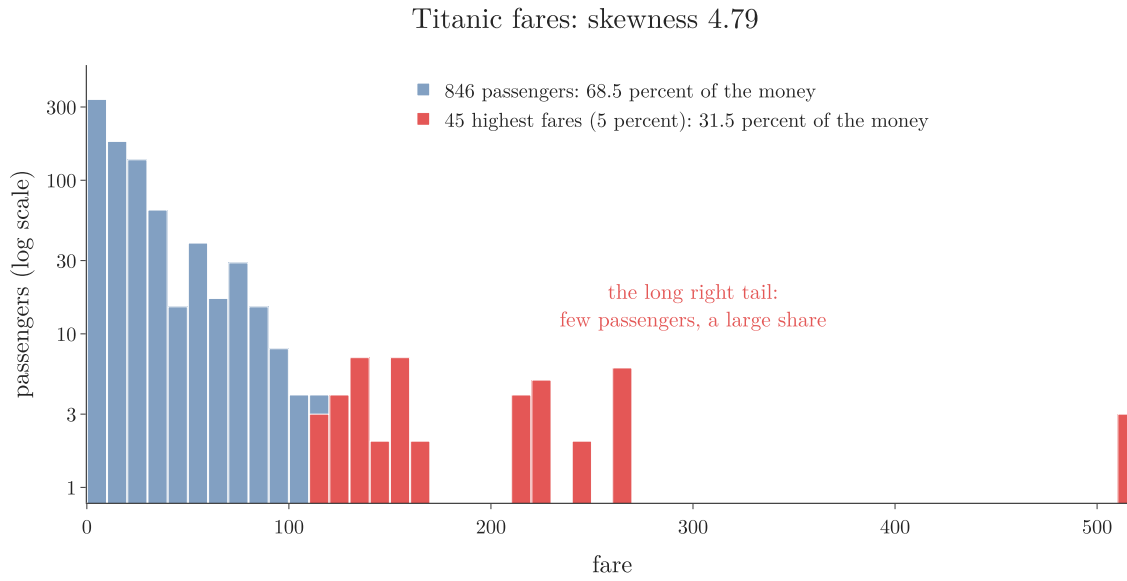
Figure 2: The 891 Titanic fares on a log count scale. The 45 highest fares (red) are the long right tail: 5 percent of the passengers, 31.5 percent of the money.
