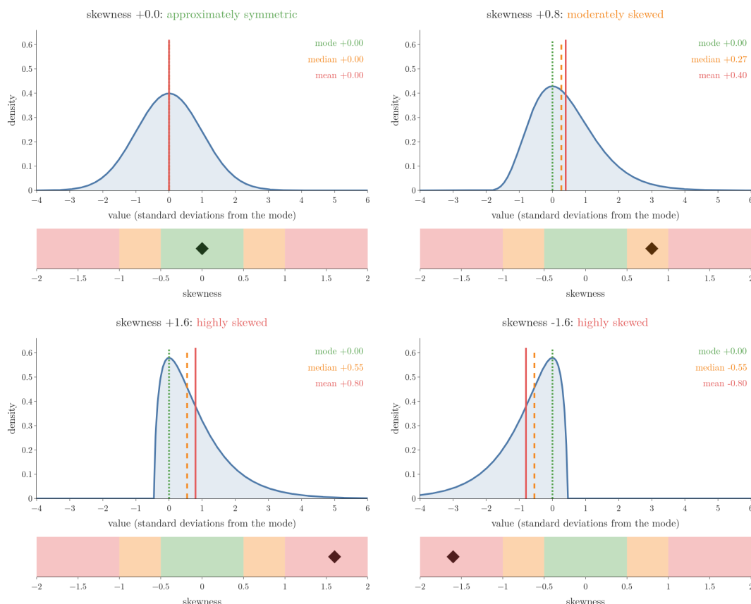
Figure 4: Skewness swept from 0 to 1.6 and to -1.6: the mode stays at the peak while the median and, further, the mean follow the long tail
