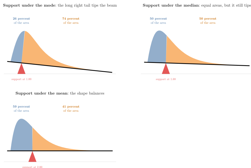
Figure 3: A right-skewed shape on a beam (mode 1, median 1.68, mean 2). The support under the mode or the median lets the long right tail tip the beam; under the mean it balances. Idea after Khan Academy, “Median, mean and skew from density curves”
