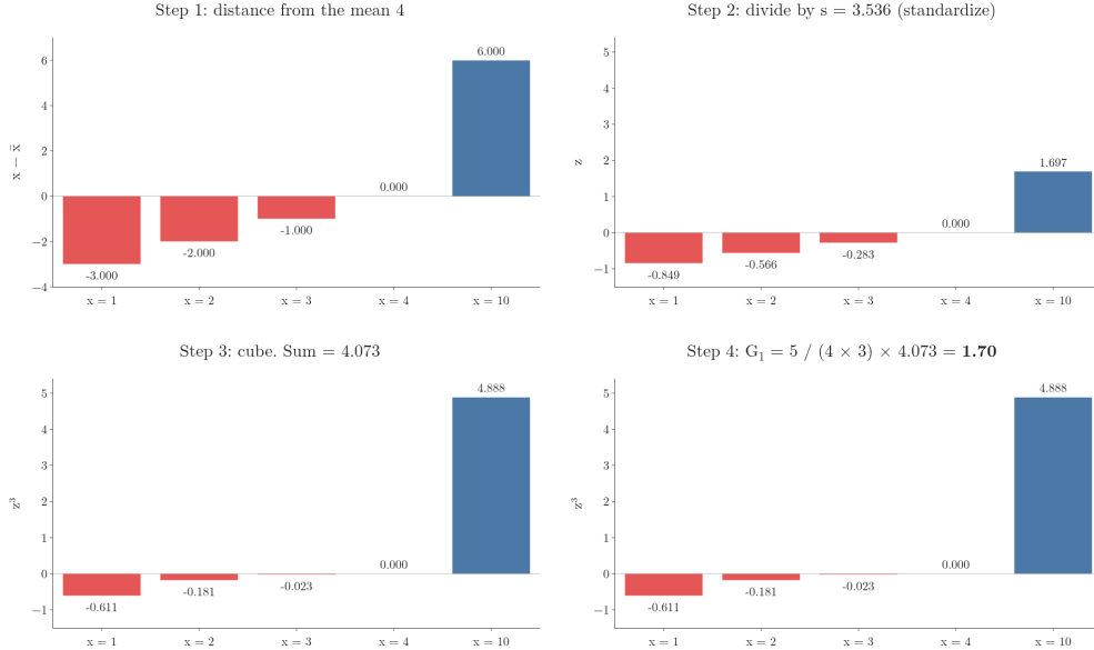
Figure 5: The sample skewness of 1, 2, 3, 4, 10 in four steps: distances from the mean, standardized values, cubes (sum 4.073), and the final G_1 = 1.70 .
