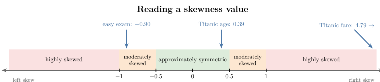
Figure 6: A rule of thumb for reading skewness values
