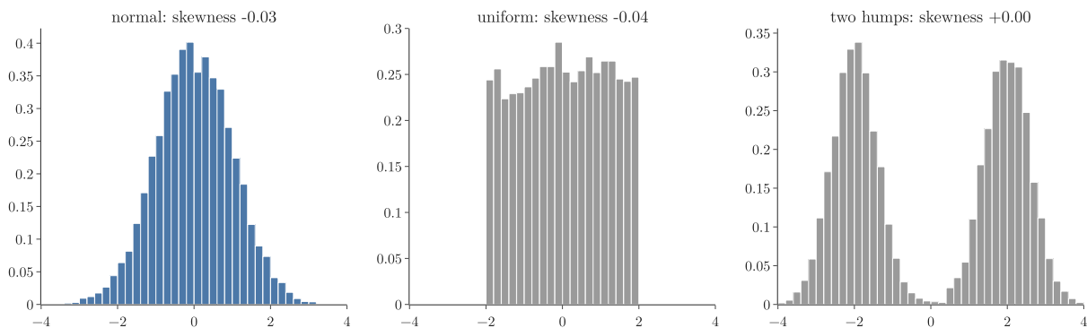
Figure 7: 10,000 values each from a normal, a uniform and a symmetric two-humped distribution. All three have skewness close to 0; only the first is normal.
